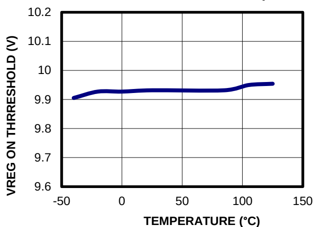
VREG On Threshold vs. Temperature
