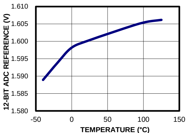
12-Bit ADC Reference vs. Temperature
