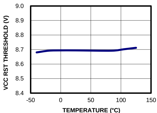
VCC RST Threshold vs. Temperature
