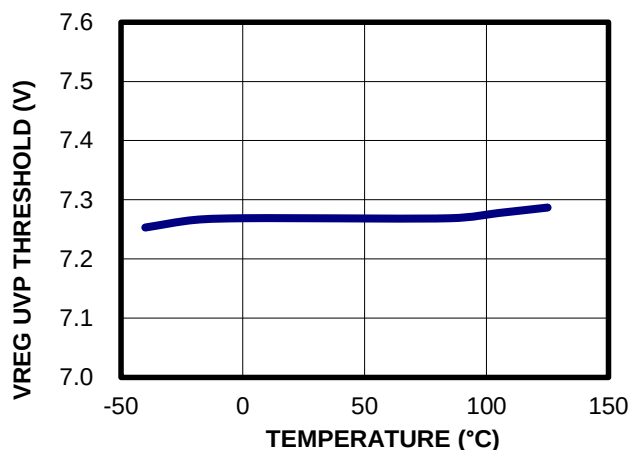
VREG UVP Threshold vs. Temperature
