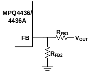
Figure 9: Feedback Network
