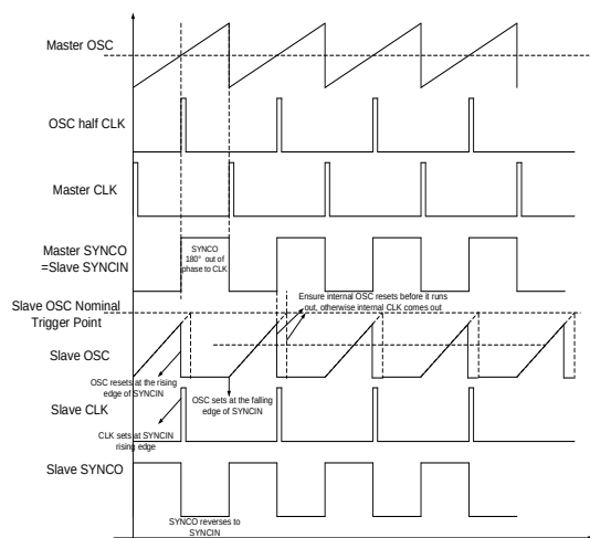
Figure 6: SYNCIN & SYNCO Scheme
