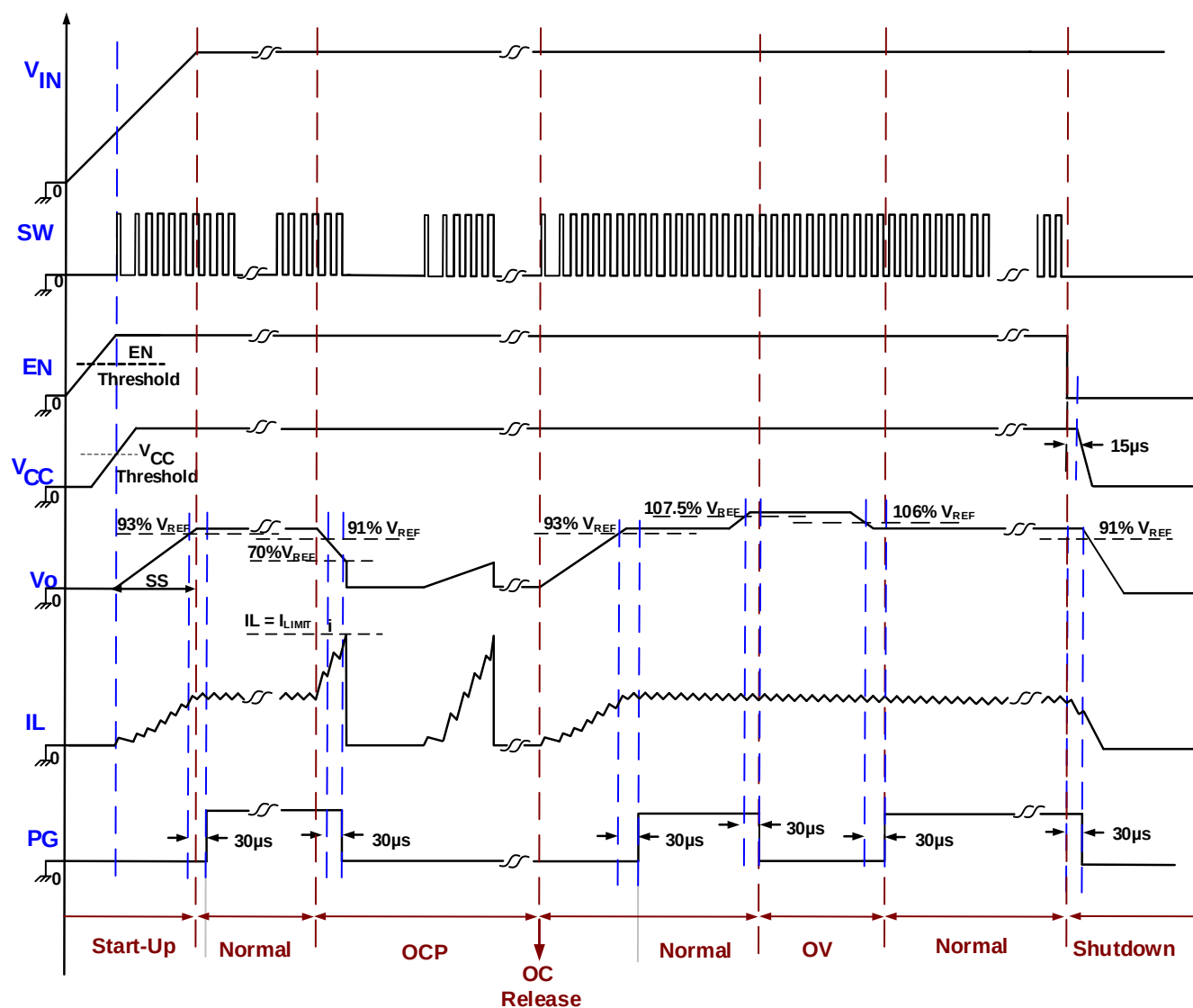
Figure 2: Timing Sequence
