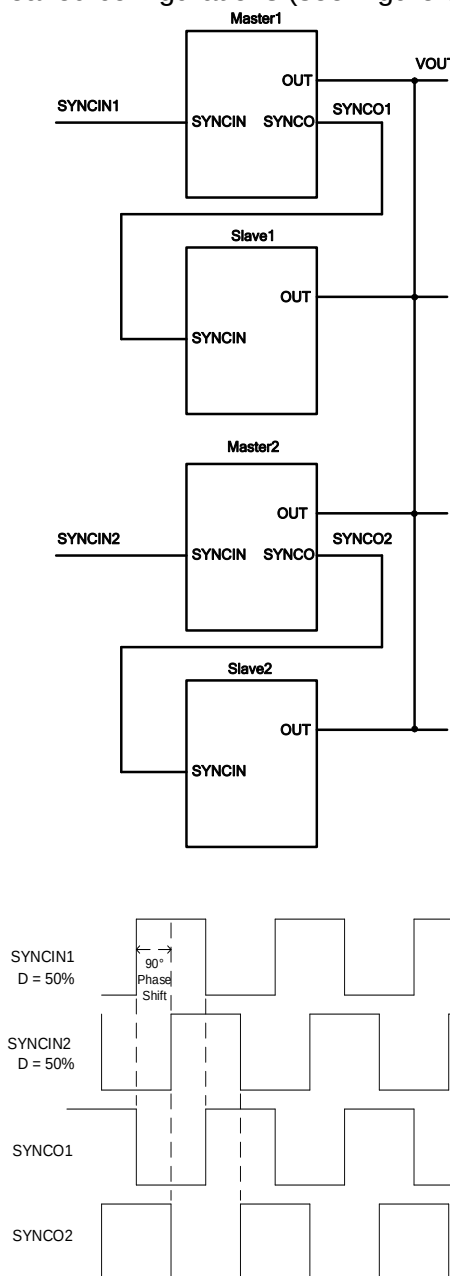
Figure 8: Four-Phase Configuration
