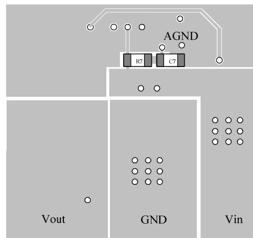
Figure 14—PCB Layout
