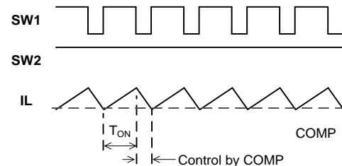
Figure 5: Buck Waveform
