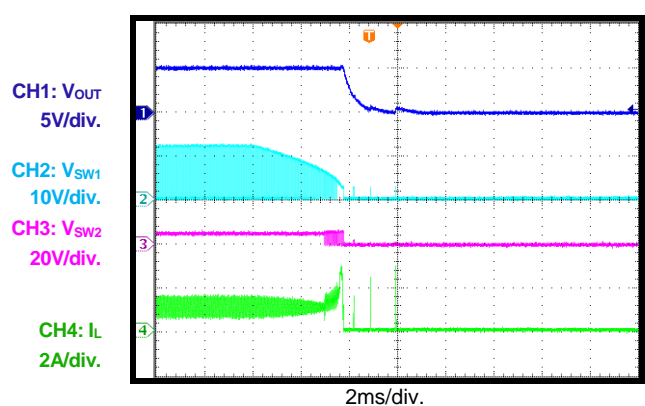
V_{IN} Power Off Load = 1A
