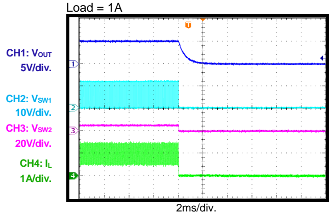
ENPWR Bit Disable through I 2 C Command Load = 1A
