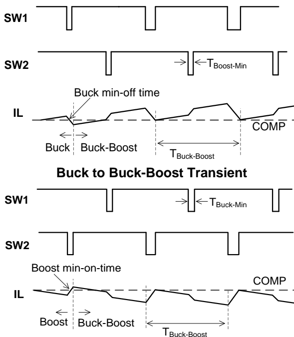
Buck to Buck-Boost Transient Boost to Buck-Boost Transient Figure 7: Buck-Boost Waveform
