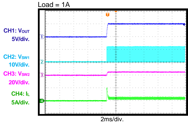
ENPWR Bit Enable through I 2 C Command Load = 1A
