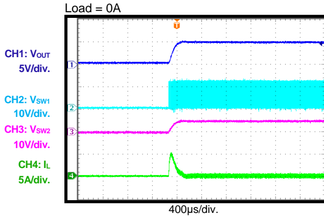
ENPWR Bit Enable through I 2 C Command Load = 0A
