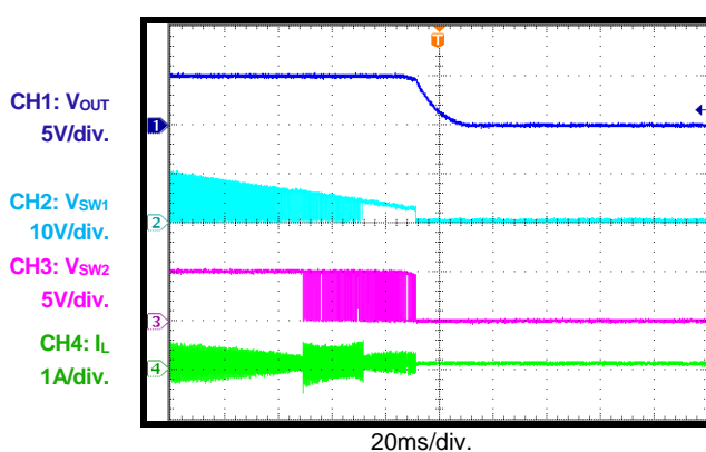
V_{IN} Power Off Load = 0A
