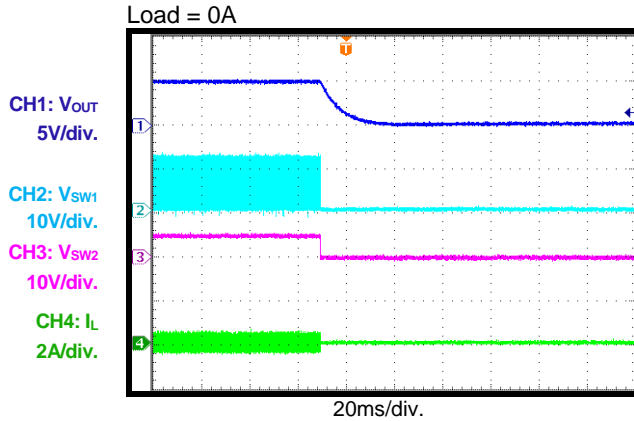
ENPWR Bit Disable through I 2 C Command Load = 0A
