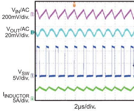
Input/Output Voltage Ripple I_{OUT} = 4A
