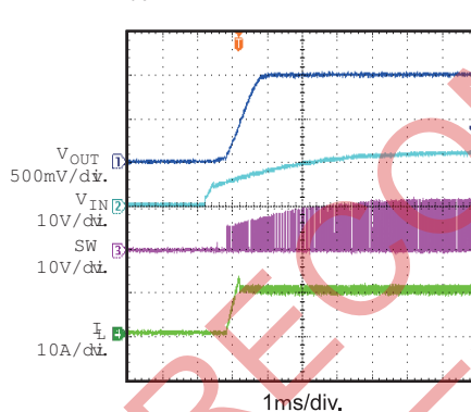
Start Up Through I_{IN} I_{OUT}=10A
