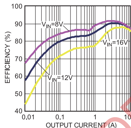
Figure 40 — Efficiency Curve
