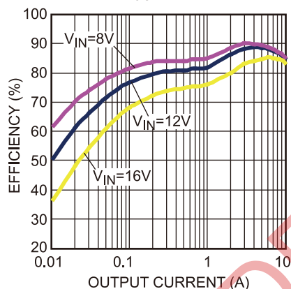
Figure 28 — Efficiency Curve
