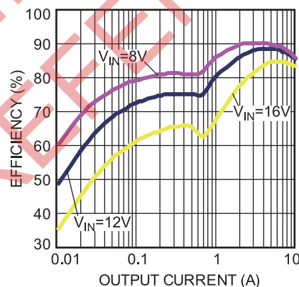
Figure 36 — Efficiency Curve
