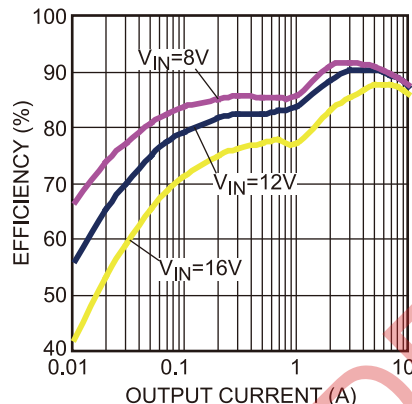
Figure 34 — Efficiency Curve
