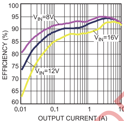
Figure 46 — Efficiency Curve
