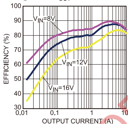
Figure 16 — Efficiency Curve
