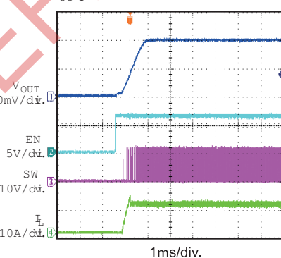
Start up through EN I_{OUT}=10A
