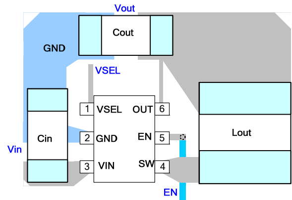
Figure 10: Two Ends of Input Decoupling Capacitor Close to Pin 2 and Pin 3
