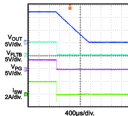
Thermal Shutdown
