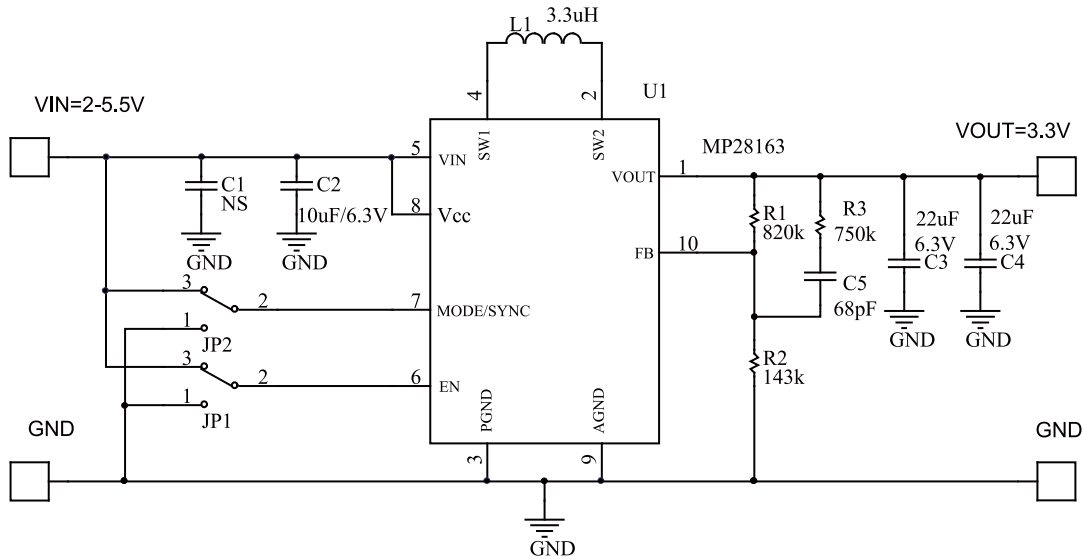
Figure 5—3.3V Output Application Circuit
