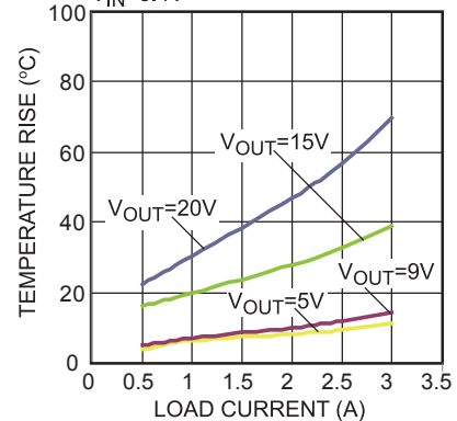
MP3428A Case Temperature Rising For Figure 11
