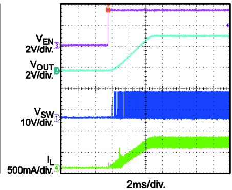
Start-Up through EN I_{OUT} = 0.6A
