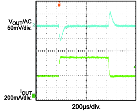
Load Transient I_{OUT} = 0.3A-0.6A, 1.6A/\mu s
