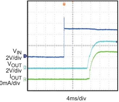
Hot Insertion V_{IN}
