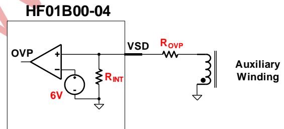
Figure 8—OVP Circuit
