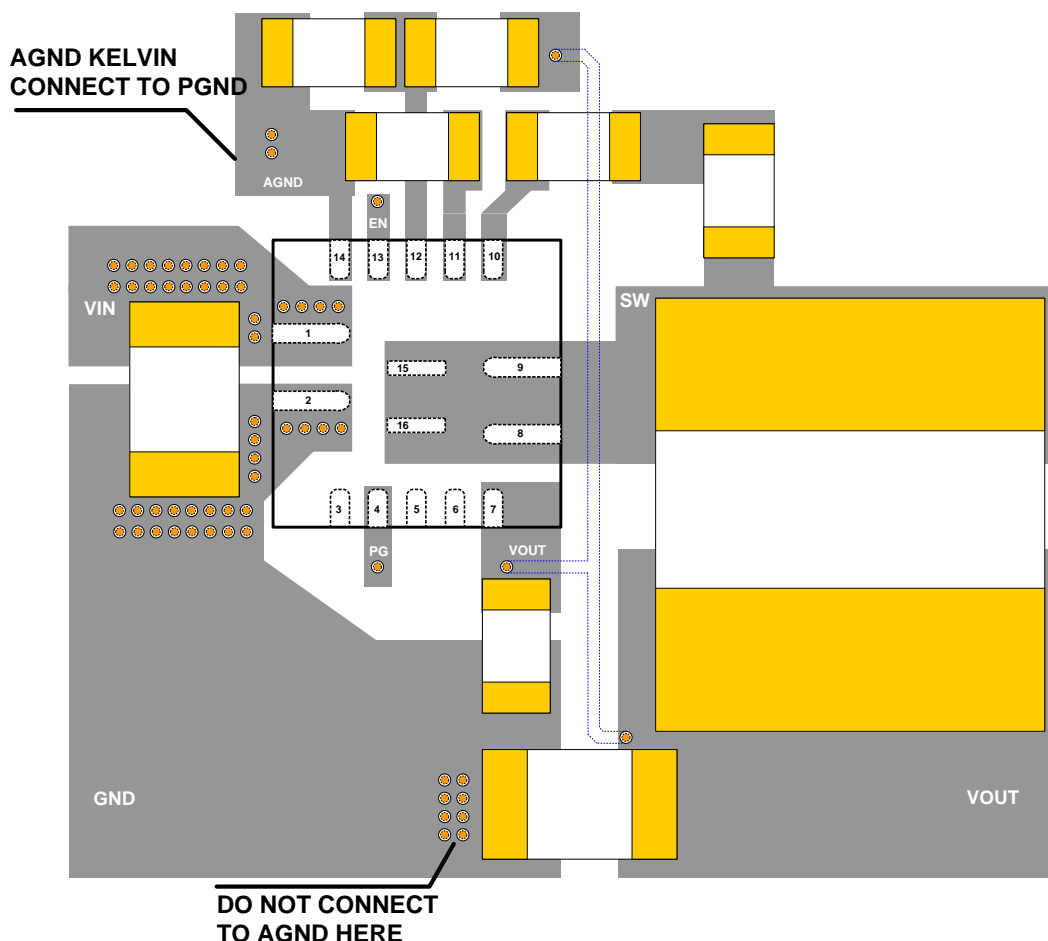
Figure 13—Recommend Layout
