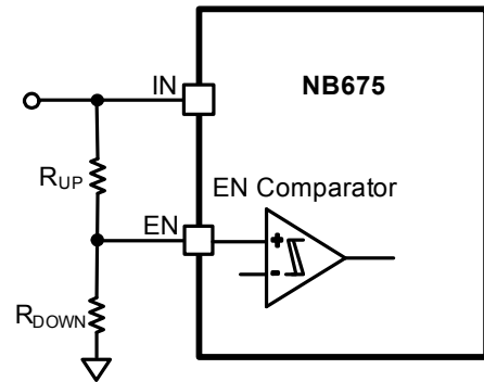
Figure 9—Adjustable UVLO
