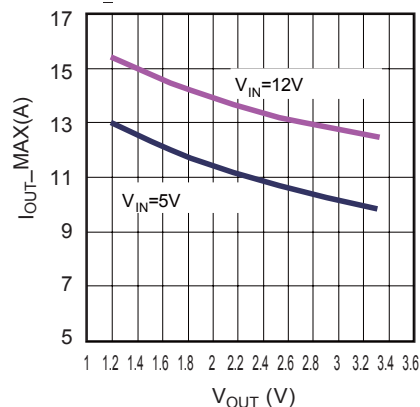
Current Derating Curves
