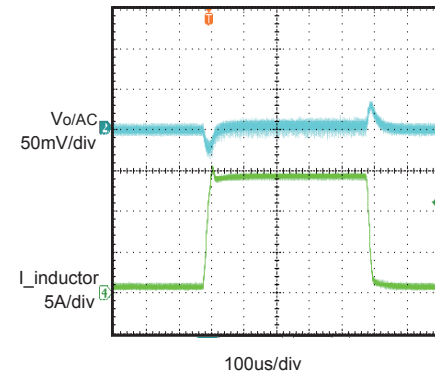
Two Phase Transient Response
