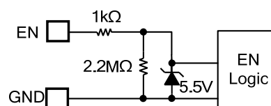
Figure 2: Zener Diode between EN and GND
