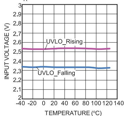
V_{IN} UVLO Rising/Falling Threshold vs. Temperature T_A = -40^\circ C to +125^\circ C
