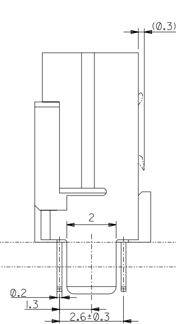
DETAILED FRONTAGE
