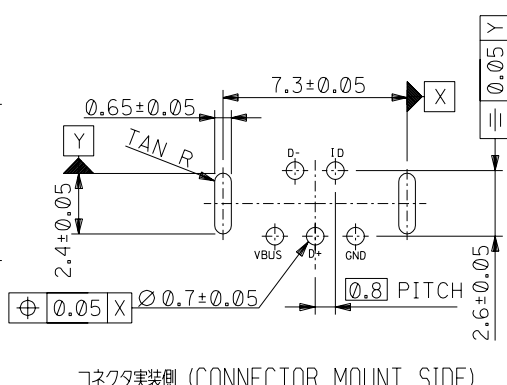
CONNECTOR MOUNT SIDE
