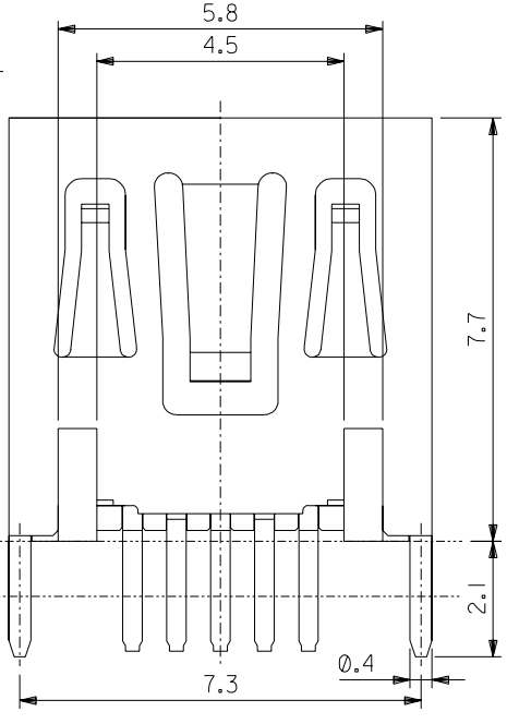
CONNECTOR MOUNT SIDE
