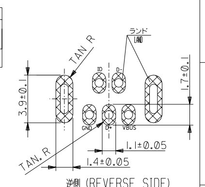
RECOMMENDED P.C.B. PATTERN LAYOUT
