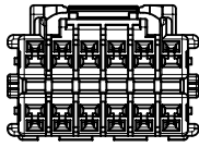
VIEW OF CKT.10,12 (SCALE 1:1)
