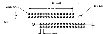
PCB LAYOUT FOR REFERENCE ONLY
