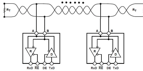
Figure10. Typical application circuit
