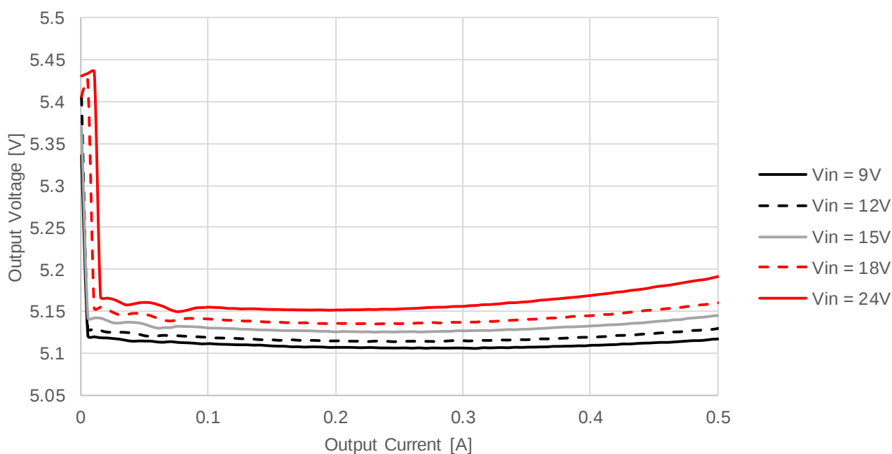
173950578 Load Regulation V_{OUT} = 5V , T_A = 85^\circ C
