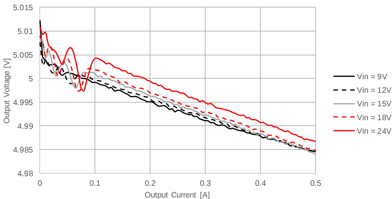
173950578 Load Regulation V_{OUT} = 5V , T_A = 25^\circ C
