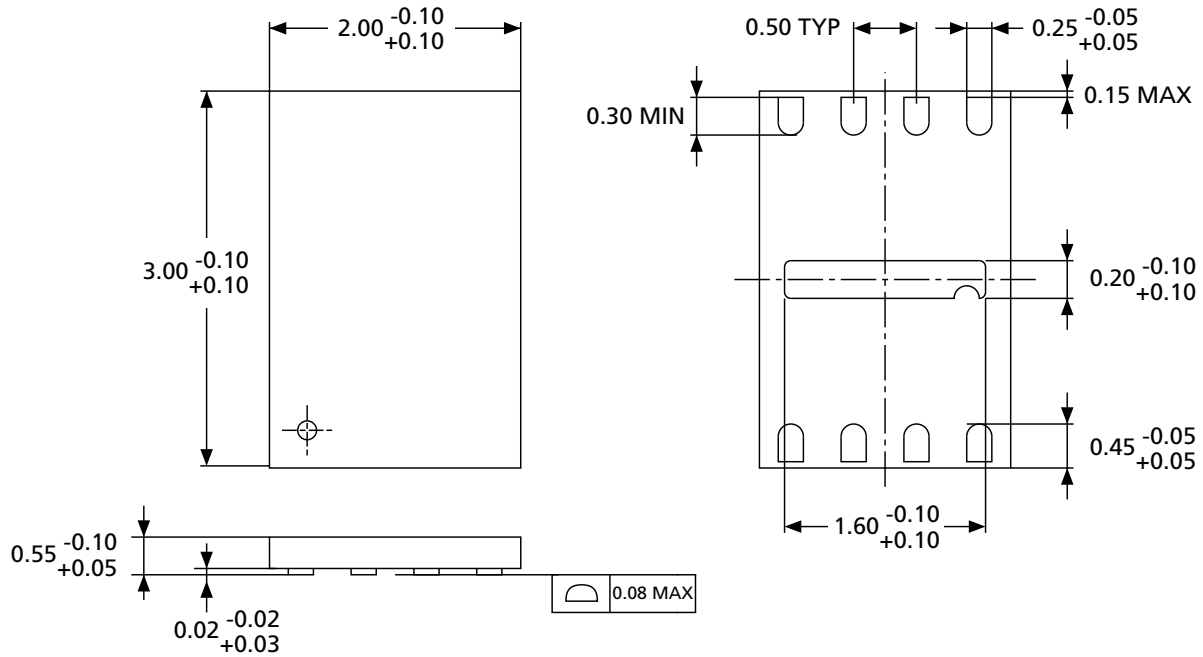
Figure 32: UFDFPN8 (MLP8) 2mm x 3mm
