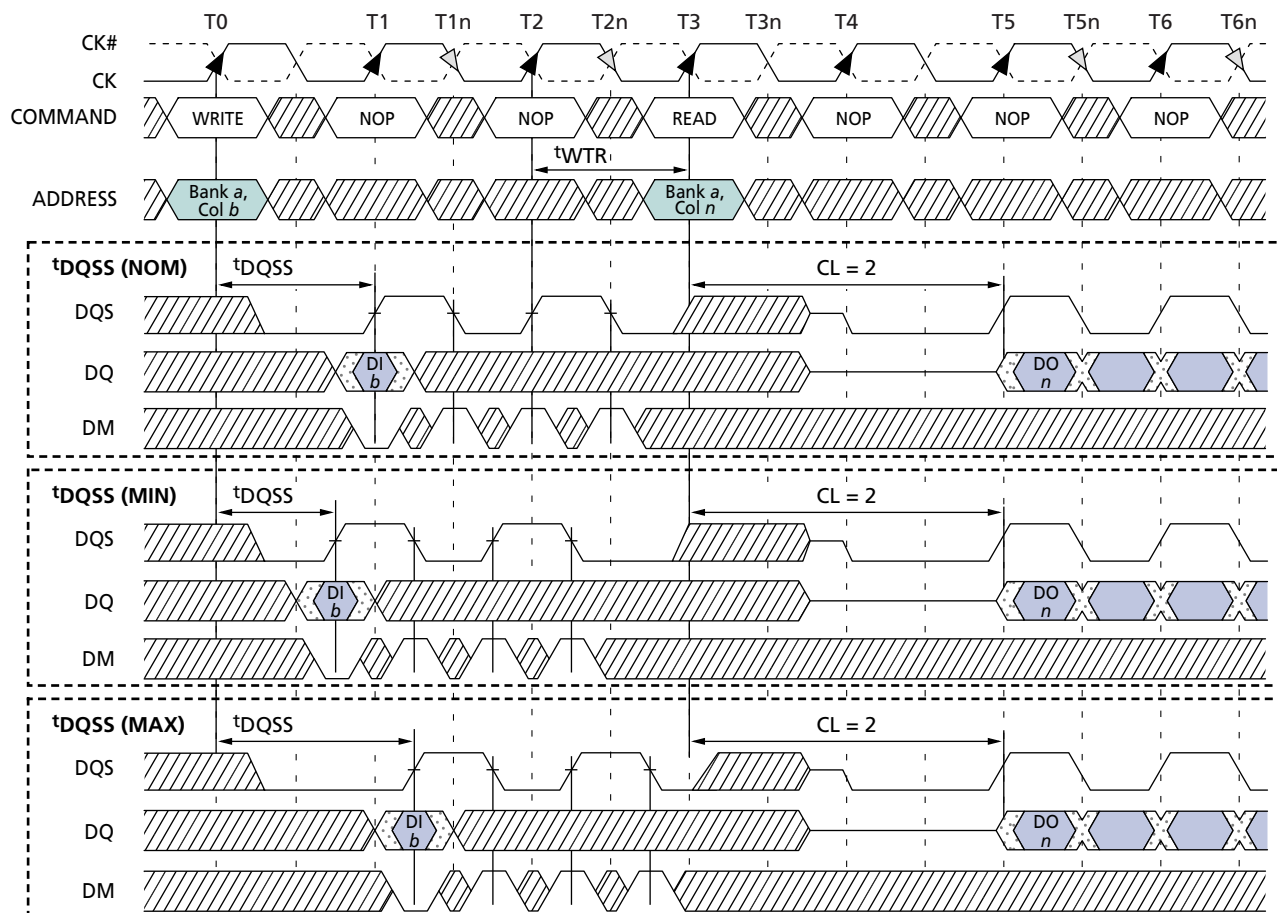
Figure 27: WRITE-to-READ – Odd Number of Data, Interrupting
