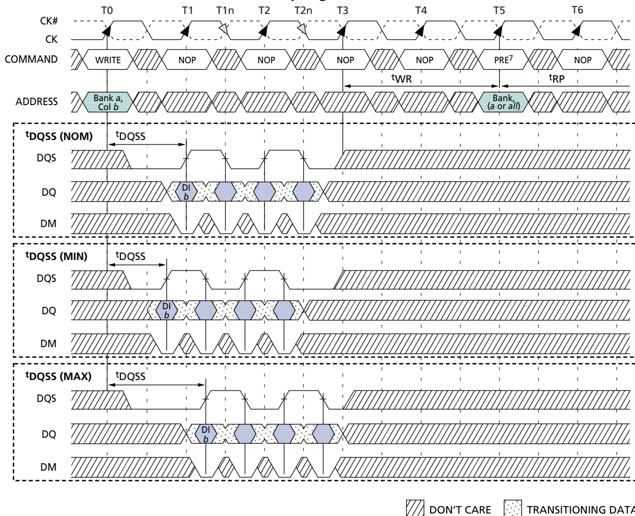
Figure 28: WRITE-to-PRECHARGE – Uninterrupting
