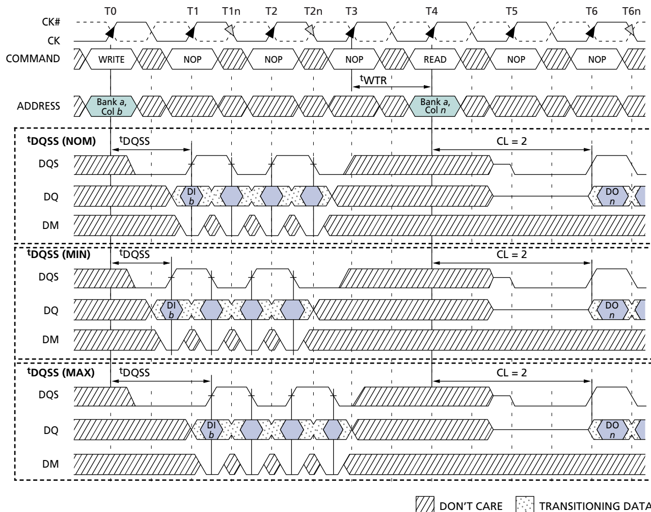
Figure 25: WRITE-to-READ – Uninterrupting
