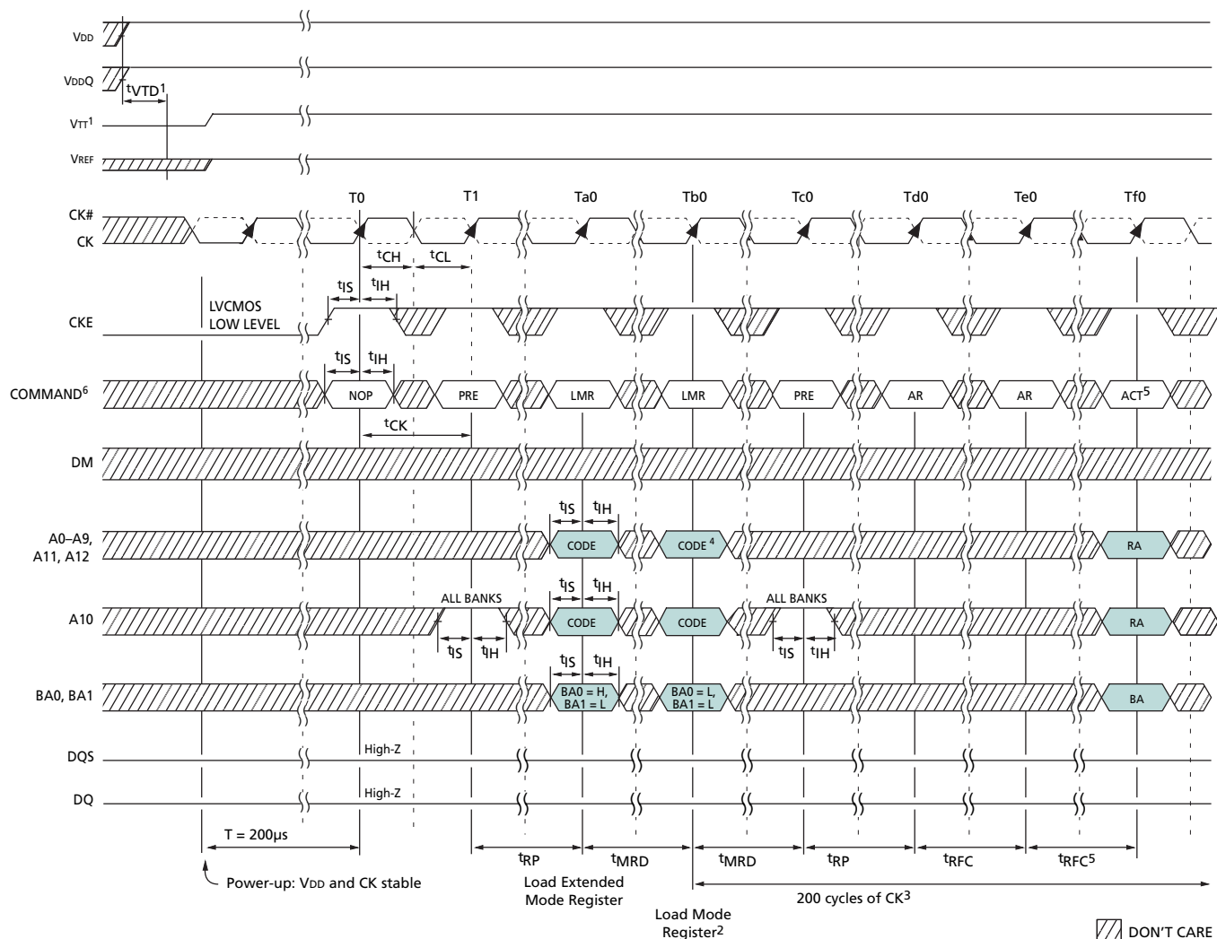
Figure 45: Initialize and Load Mode Registers
