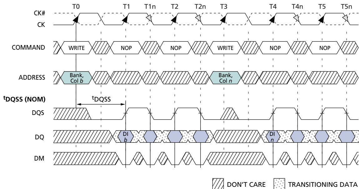
Figure 23: Nonconsecutive WRITE-to-WRITE
