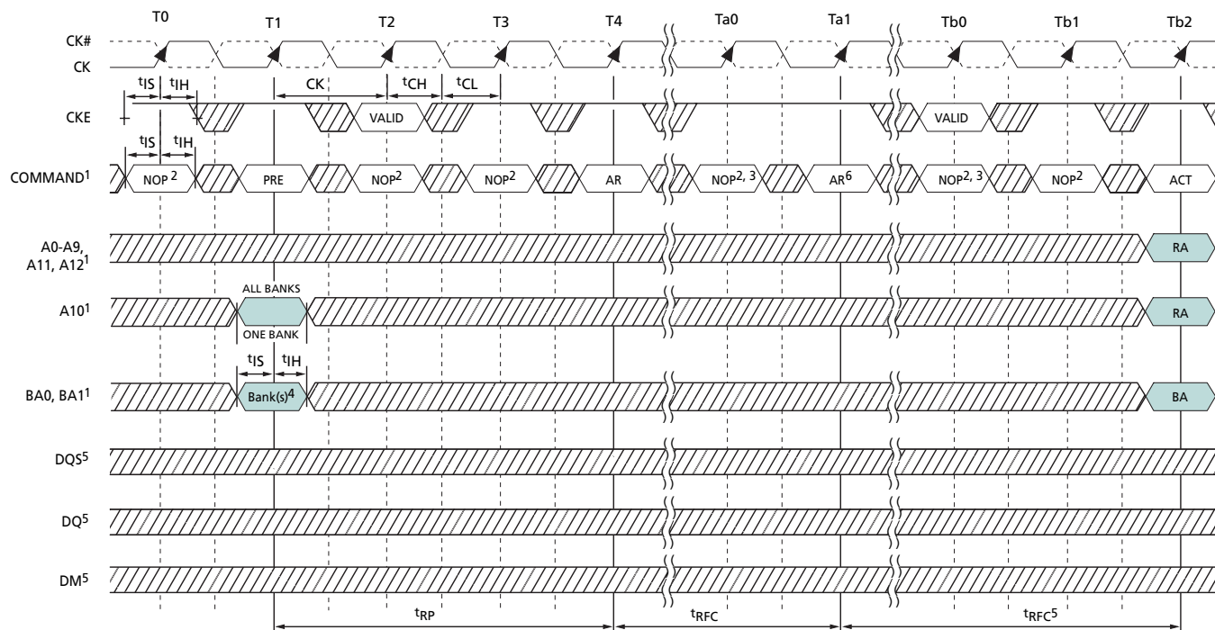
Figure 47: Auto Refresh Mode
