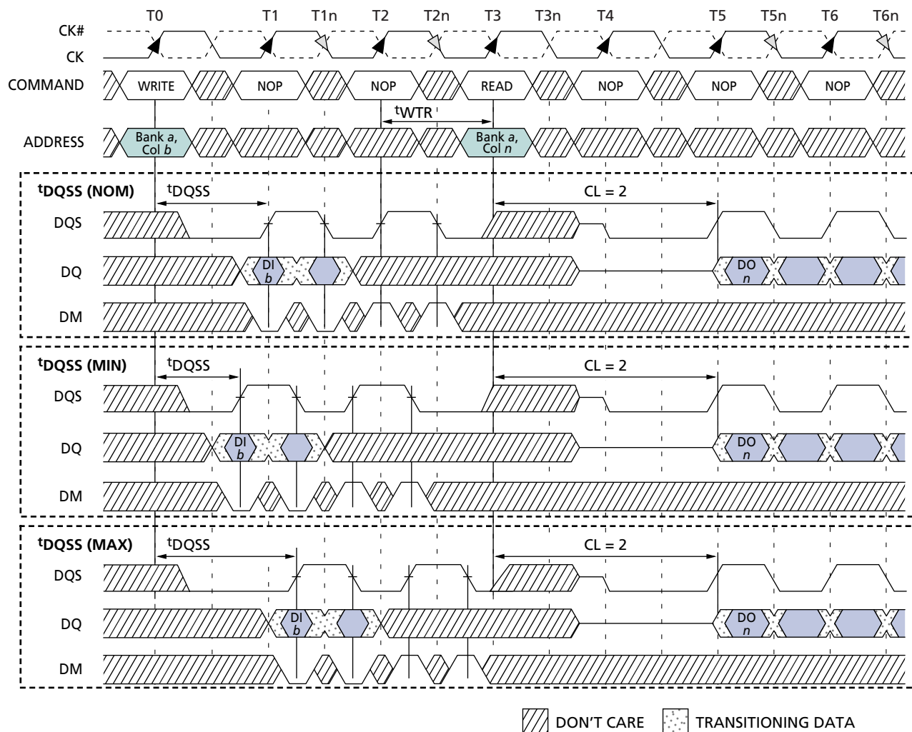
Figure 26: WRITE-to-READ – Interrupting
