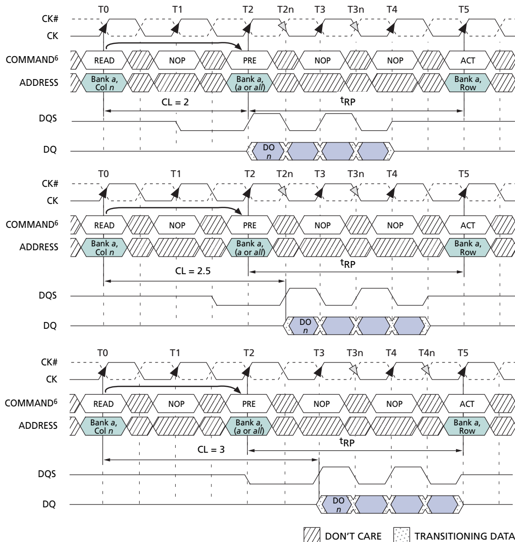
Figure 19: READ-to-PRECHARGE
