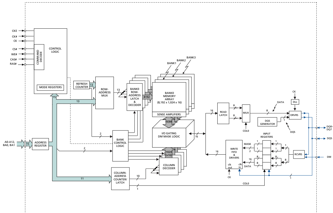
Figure 3: 64 Meg x 8 Functional Block Diagram
