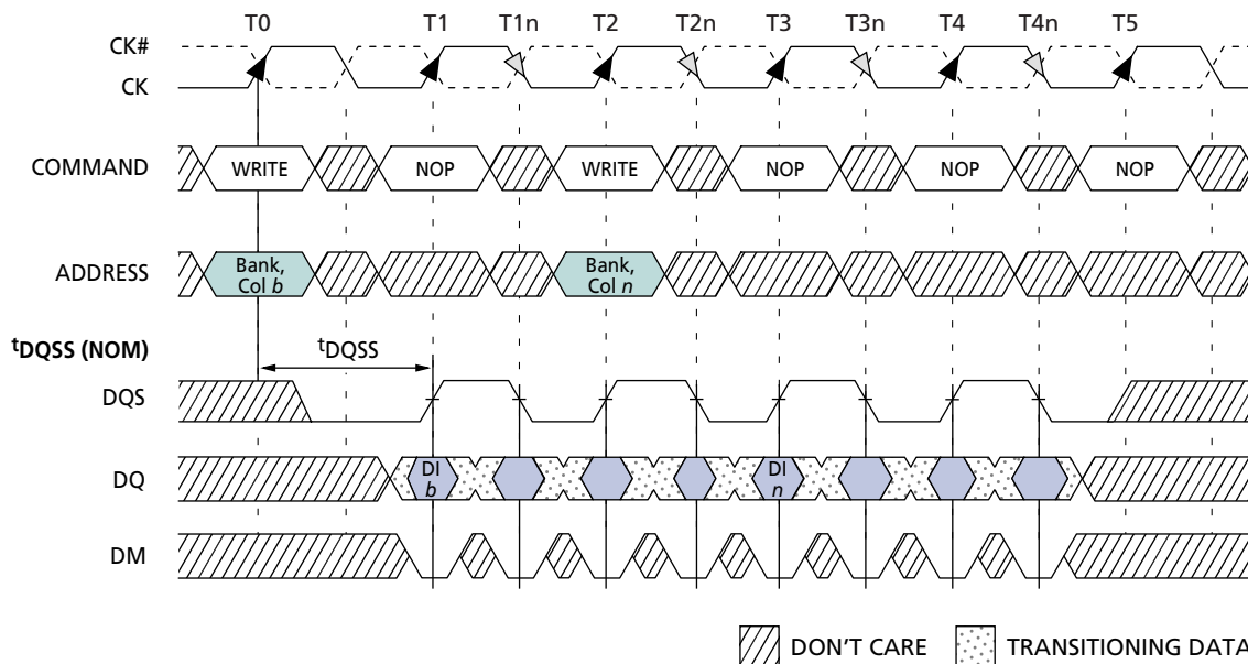
Figure 22: Consecutive WRITE-to-WRITE
