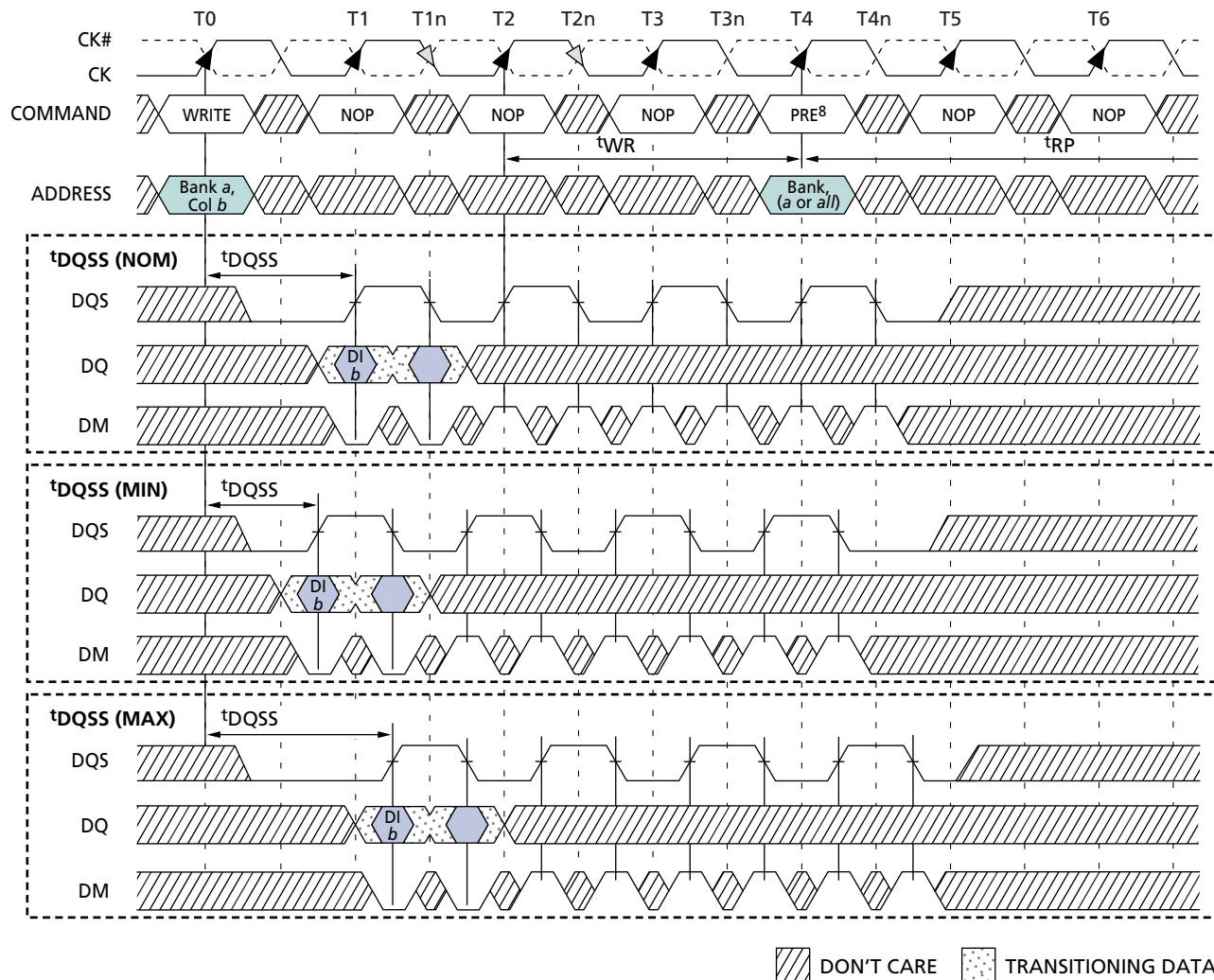
Figure 29: WRITE-to-PRECHARGE – Interrupting
