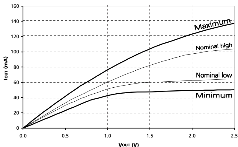
Figure 39: Reduced Drive Pull-Up Characteristics
