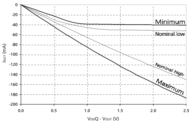
Figure 39: Reduced Drive Pull-Up Characteristics
