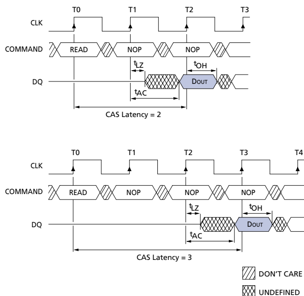
Figure 6: CAS Latency
