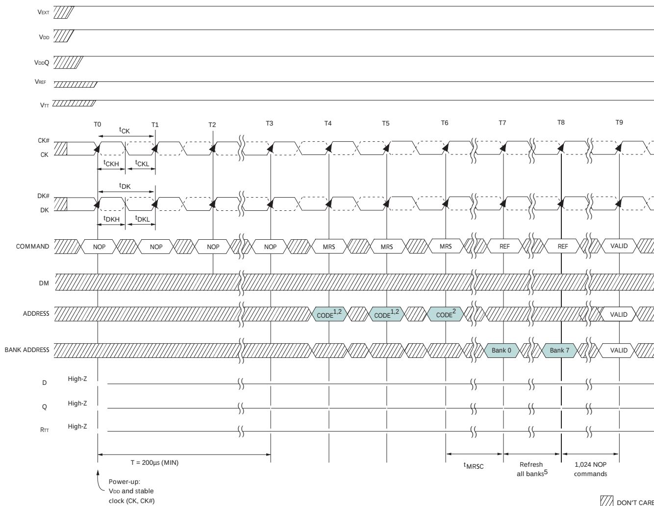
Figure 15: Power-Up/Initialization Sequence
