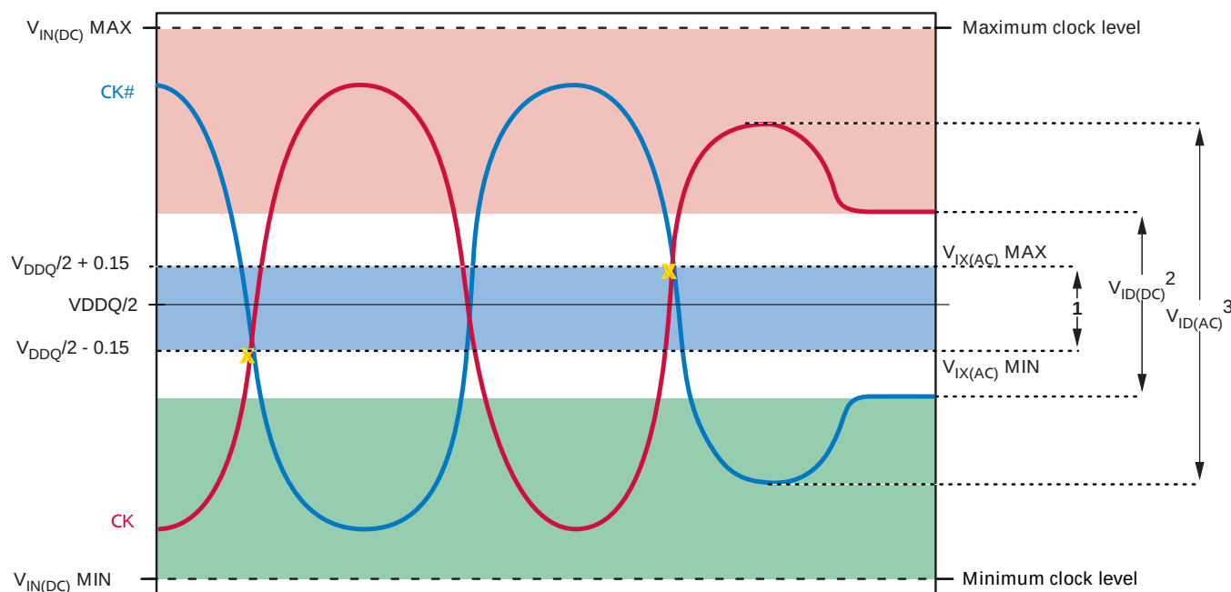
Figure 5: Clock Input
