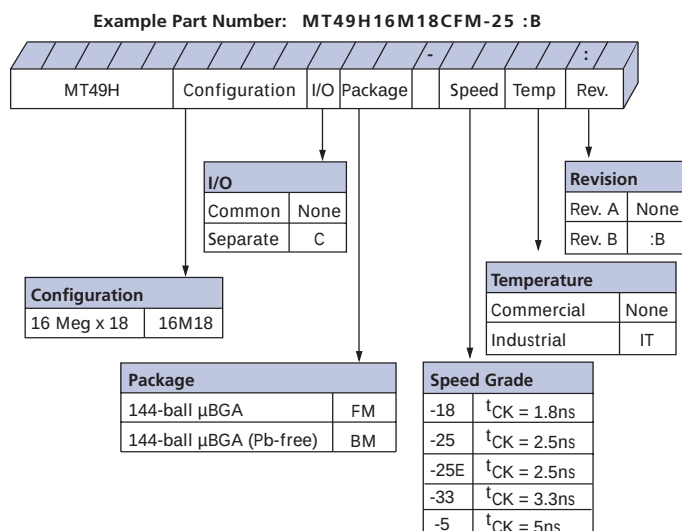
Figure 1: 288Mb RLDRAM II SIO Part Numbers
