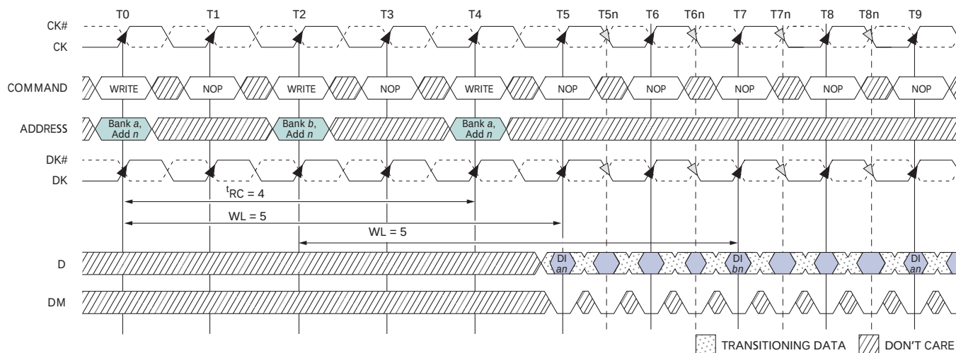
Figure 18: Consecutive WRITE-to-WRITE
