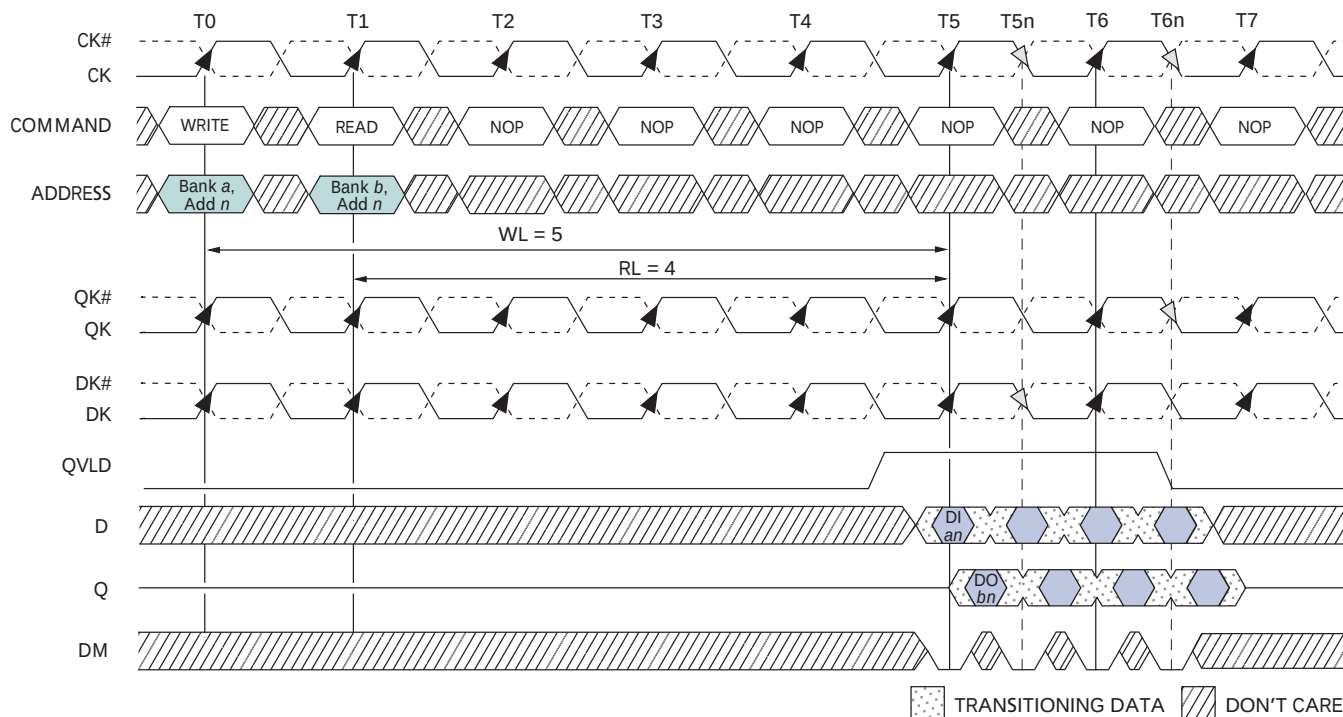
Figure 19: WRITE-to-READ
