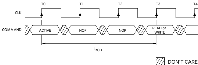
Figure 4 Example: Meeting t_{RCD}(\text{MIN}) When 2 < t_{RCD}(\text{MIN})/t_{CK} \leq 3
