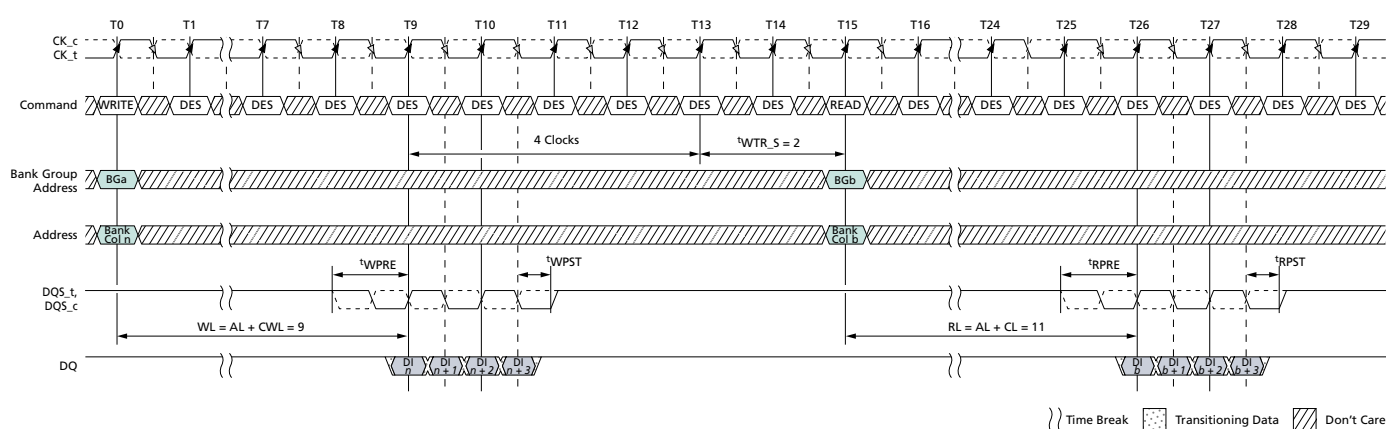
Figure 179: WRITE (BC4) OTF to READ (BC4) OTF with 1^{\text{t}} CK Preamble in Different Bank Group
