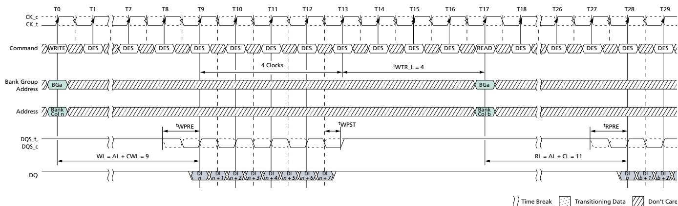
Figure 178: WRITE (BL8) to READ (BL8) with 1^{\text{t}} CK Preamble in Same Bank Group
