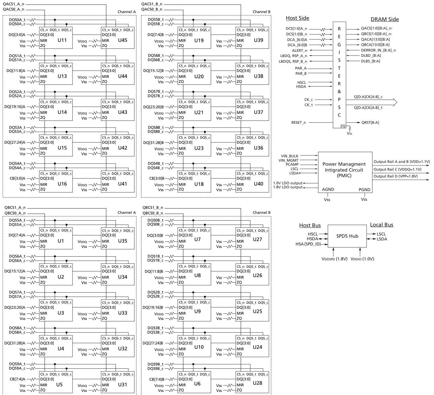
Figure 3: Functional Block Diagram (R/C-A0)
