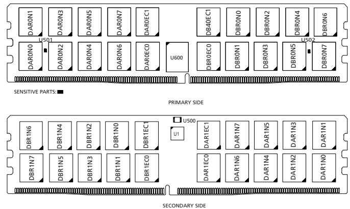
Figure 2: 288-Pin DDR5 RDIMM (R/C-A1)
