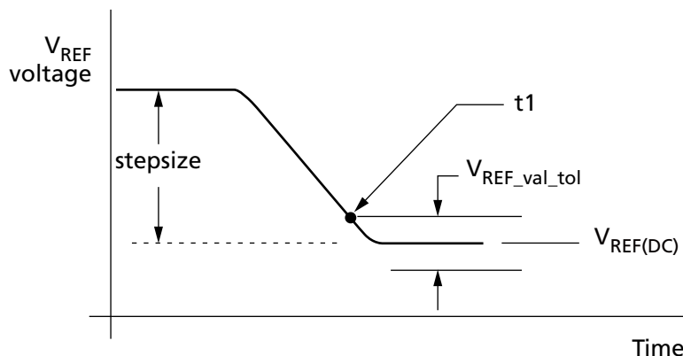
Figure 116: V_{REF(DQ)} Full Step from V_{REF,min} to V_{REF,max}
