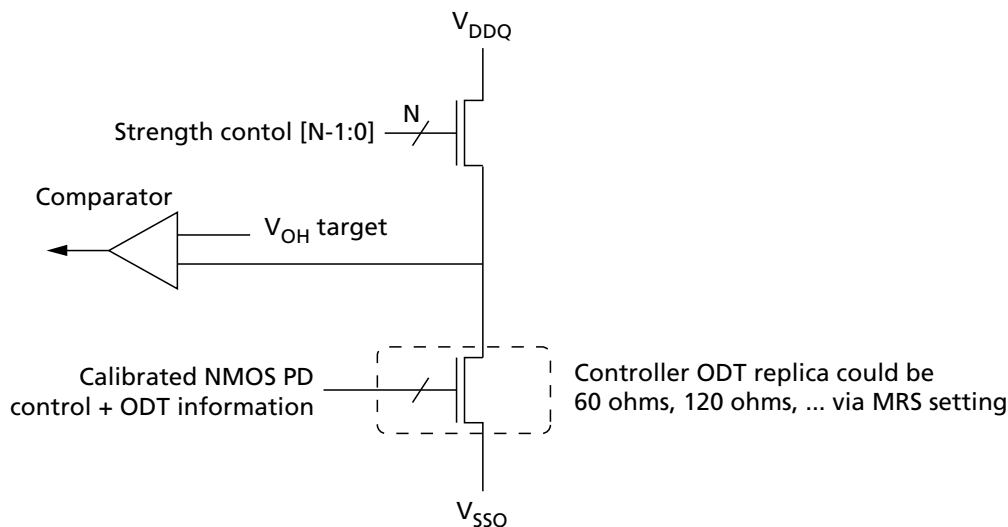
Figure 193: Pull-Up Calibration
