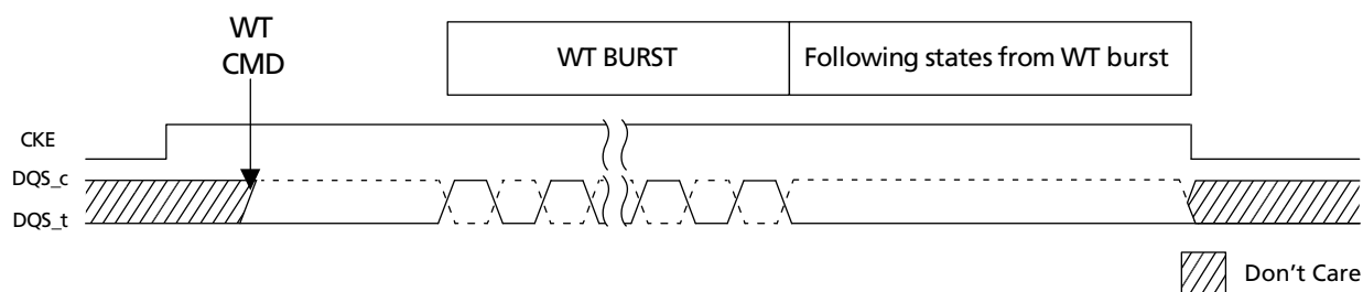
Figure 41: WDQS Control Mode 1
