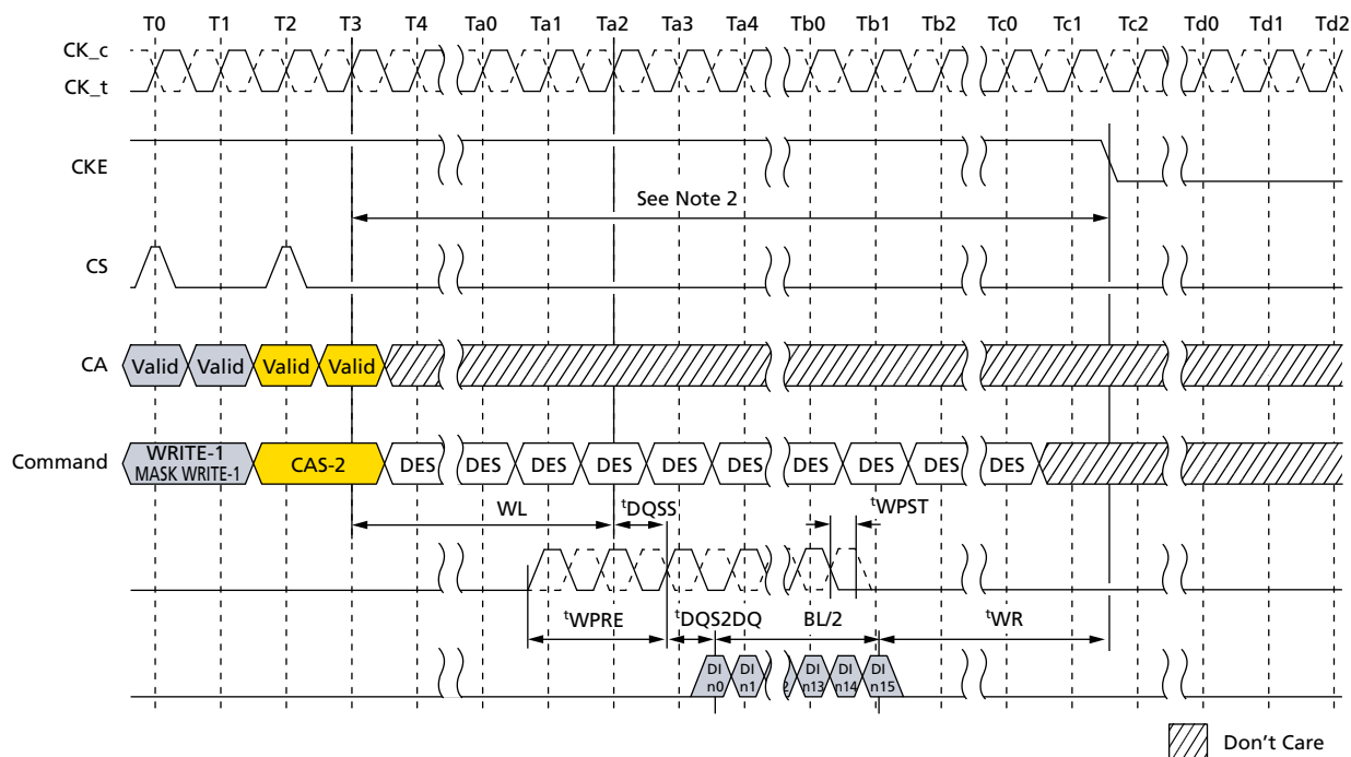
Figure 89: Write and Mask Write to Power-Down Entry
