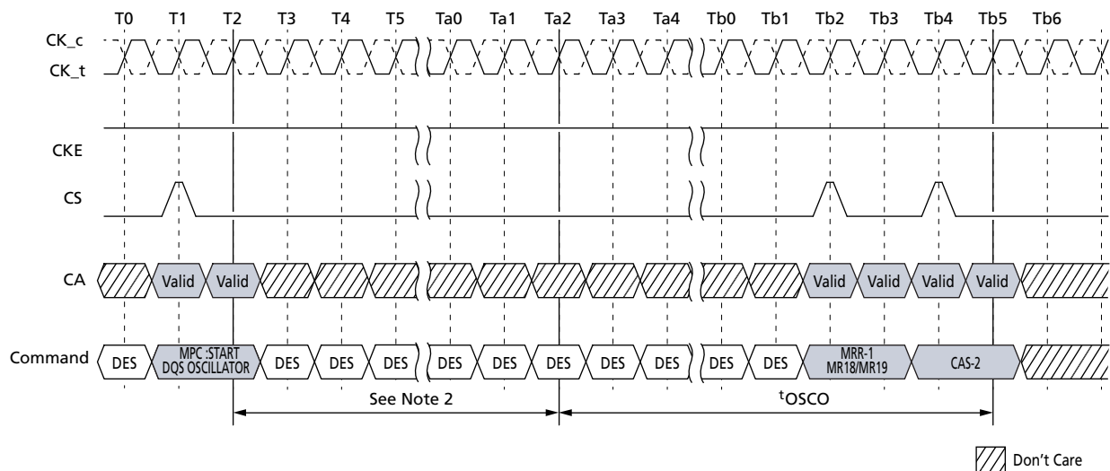
Figure 139: In Case of DQS Interval Oscillator is Stopped by DQS Interval Timer
