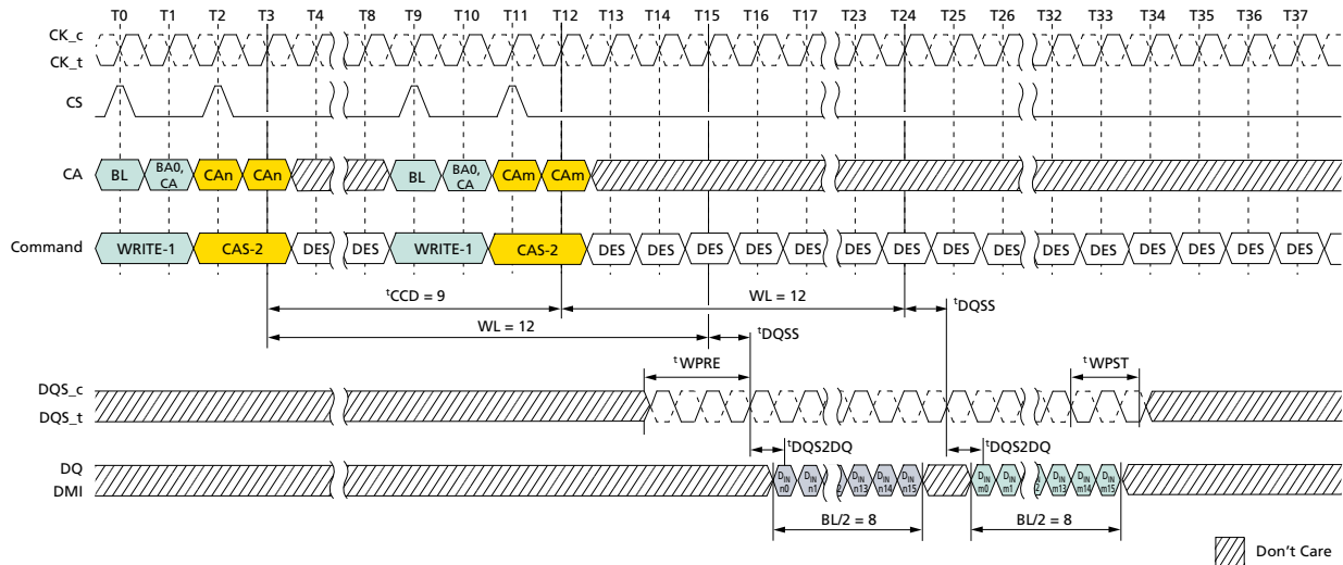
Figure 62: Consecutive WRITE: t_{CCD} = \text{MIN} + 1, 1.5nCK Postamble
