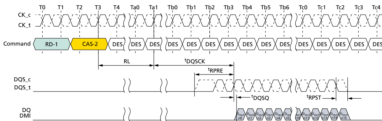
Figure 20: DQS Read Preamble and Postamble – Toggling Preamble and 0.5 n CK Postamble
