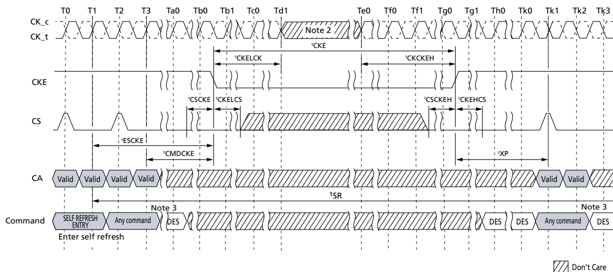
Figure 84: Command Input Timings after Power-Down Exit During Self Refresh
