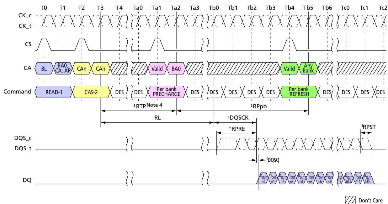
Figure 80: Burst READ Operation Followed by Per-Bank Refresh
