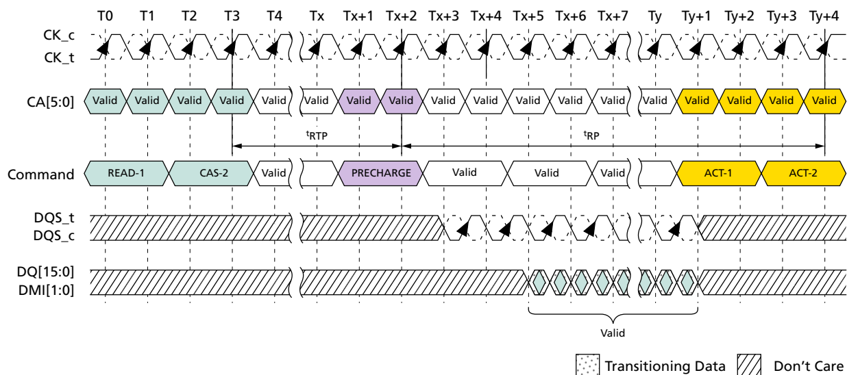
Figure 68: Burst READ Followed by Precharge – BL16, Toggling Preamble, 0.5nCK Postamble
