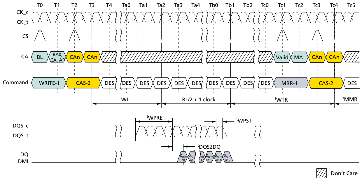
Figure 99: WRITE-to-MRR Timing
