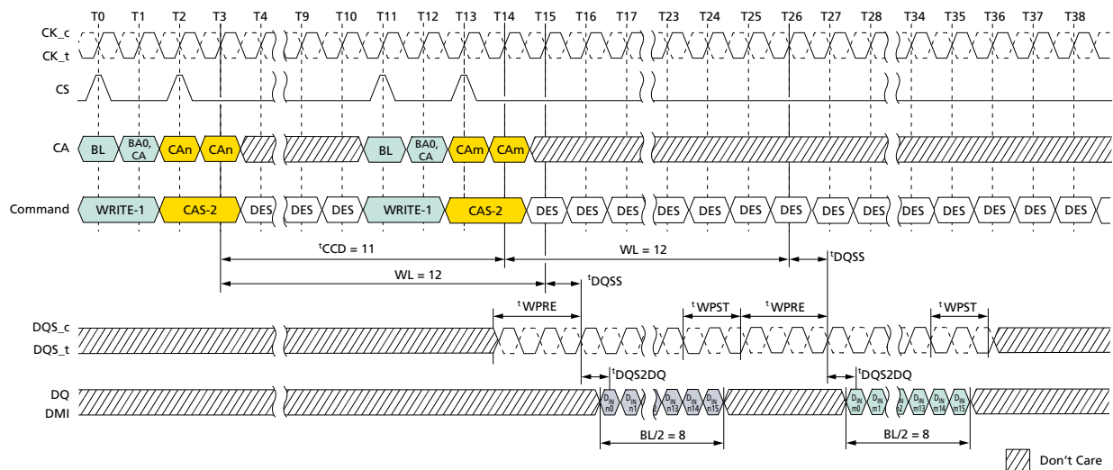
Figure 66: Consecutive WRITE: t_{CCD} = \text{MIN} + 3, 1.5n\text{CK} Postamble
