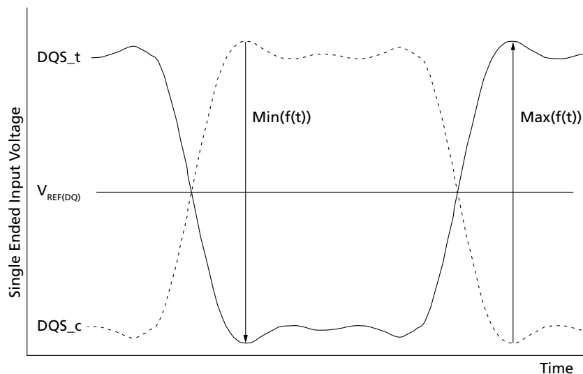
Figure 161: Definition of Differential DQS Peak Voltage
