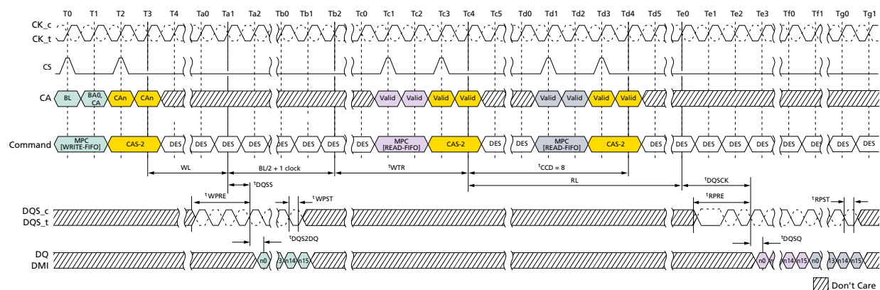
Figure 133: MPC[WRITE-FIFO]-to-MPC[READ-FIFO] Timing
