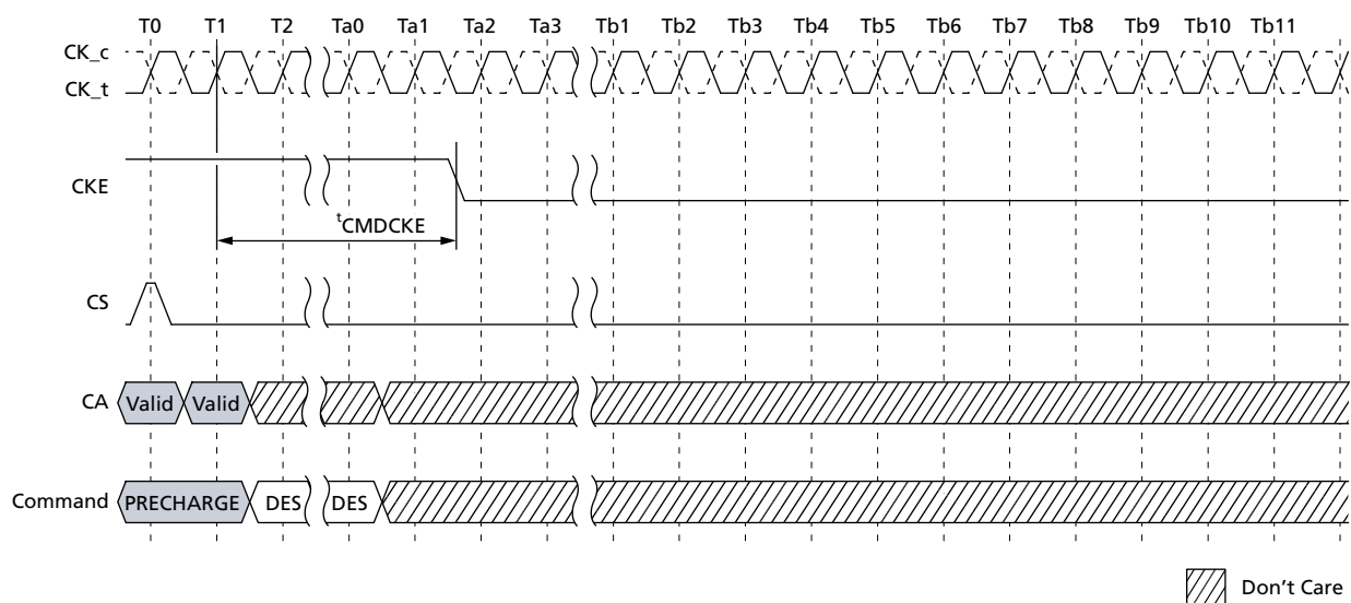
Figure 93: PRECHARGE Command to Power-Down Entry
