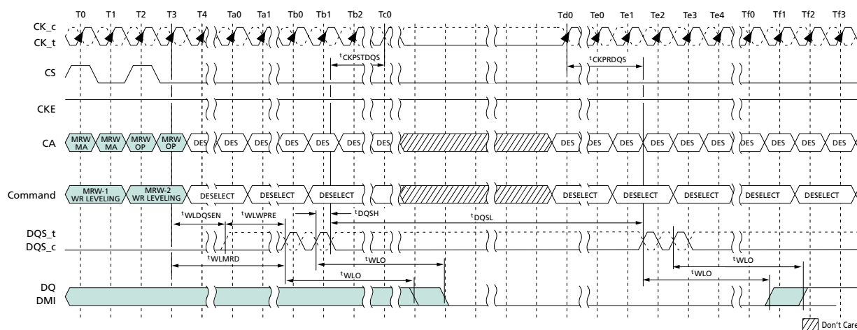
Figure 124: Clock Stop and Timing During Write Leveling
