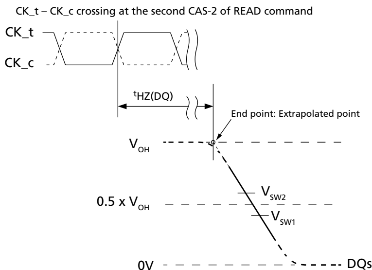
Figure 31: t_{HZ}(DQ) Method for Calculating Transitions and Endpoint
