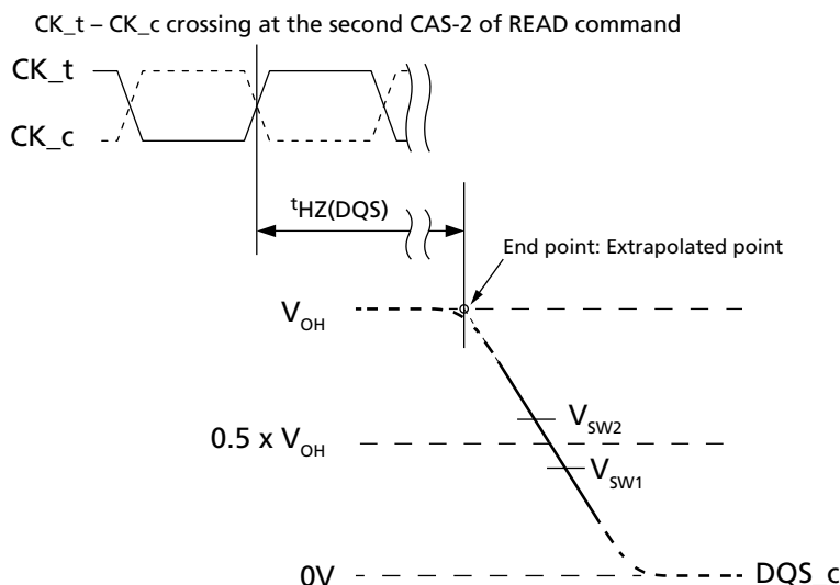
Figure 29: t_{HZ}(\text{DQS}) Method for Calculating Transitions and Endpoint
