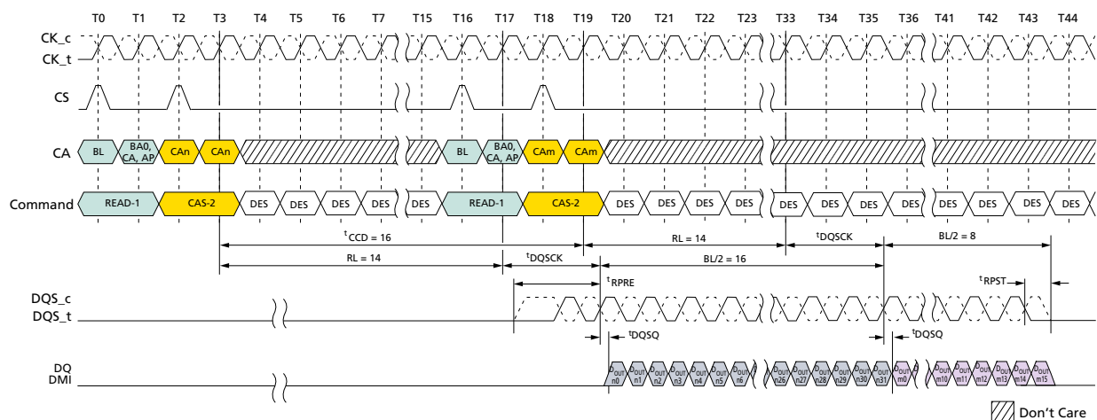
Figure 24: Burst Read Timing
