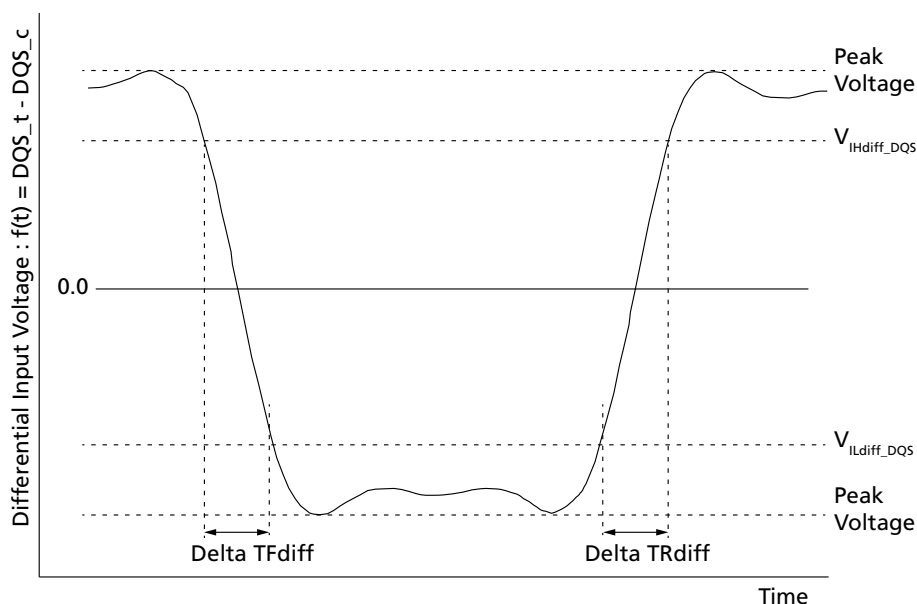
Figure 163: Differential Input Slew Rate Definition for DQS t , DQS c
