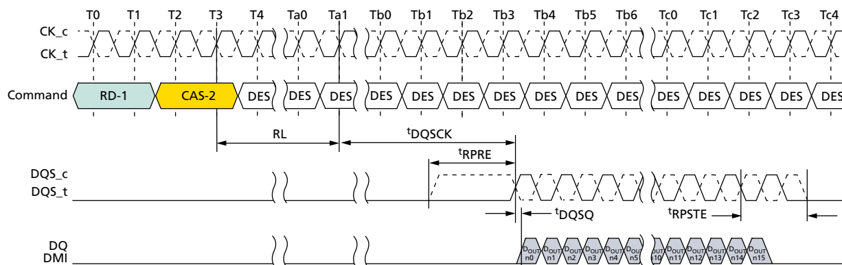
Figure 21: DQS Read Preamble and Postamble – Static Preamble and 1.5 n CK Postamble
