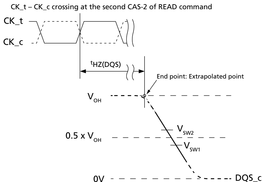
Figure 185: t_{HZ}(DQS) Method for Calculating Transitions and Endpoint
