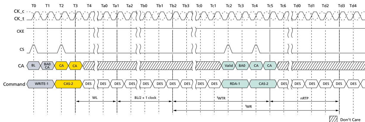
Figure 75: Delay Time From WRITE-to-READ with Auto Precharge
