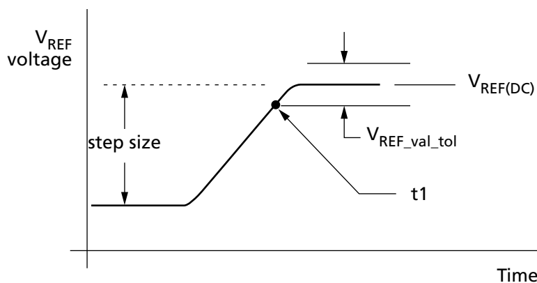
Figure 107: V_{REF(CA)} Single-Step Increment
