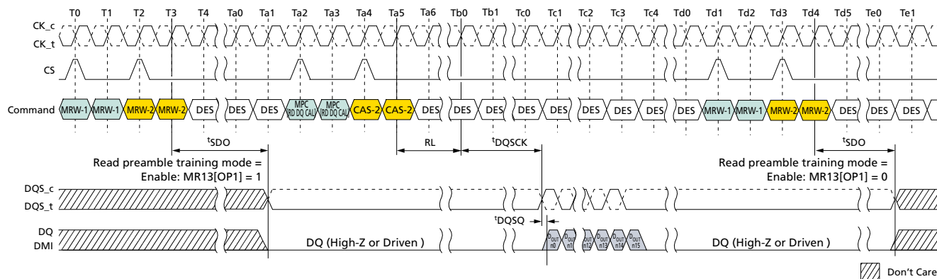
Figure 152: Read Preamble Training
