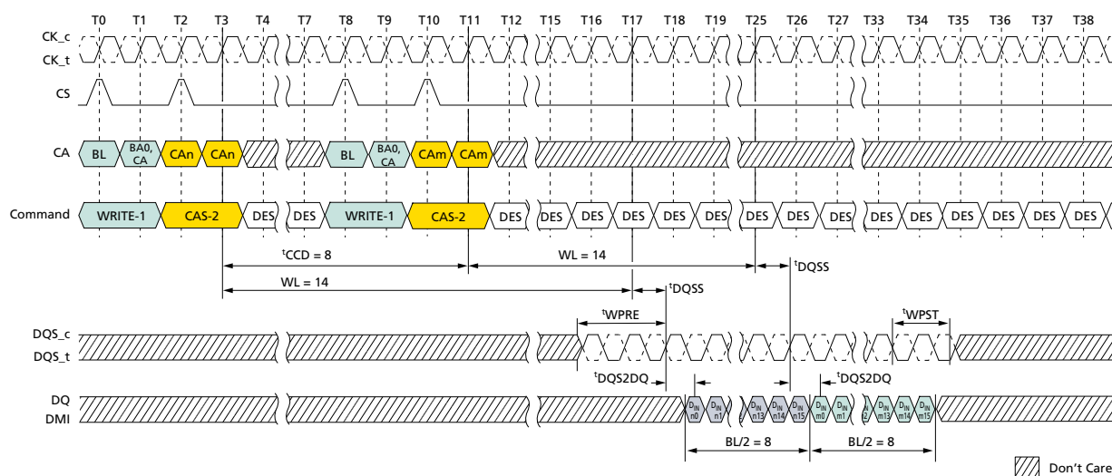
Figure 60: Seamless WRITE: t_{\text{CCD}} = \text{MIN} , 1.5n\text{CK} Postamble
