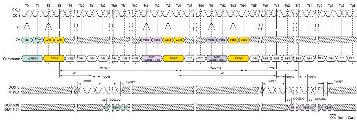
Figure 126: WRITE-FIFO – t_{WPRE} = 2nCK , t_{WPST} = 0.5nCK
