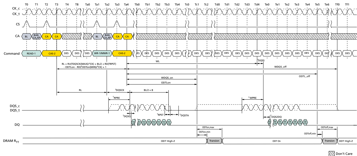
Figure 44: Burst READ Followed by Burst WRITE or Burst MASKED WRITE (ODT Enable)
