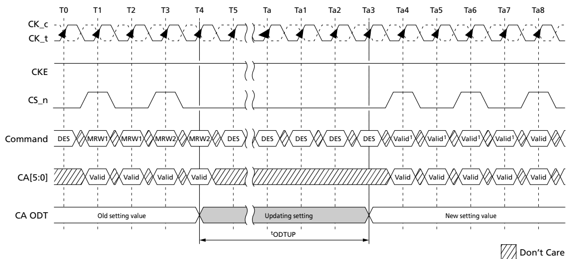
Figure 147: ODT for CA Setting Update Timing in 4-Clock Cycle Command
