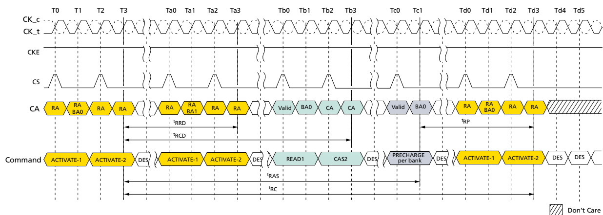
Figure 18: ACTIVATE Command
