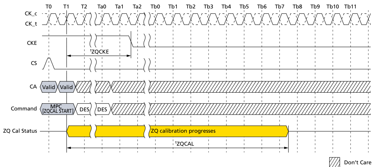
Figure 96: MULTI PURPOSE Command for ZQCAL Start to Power-Down Entry
