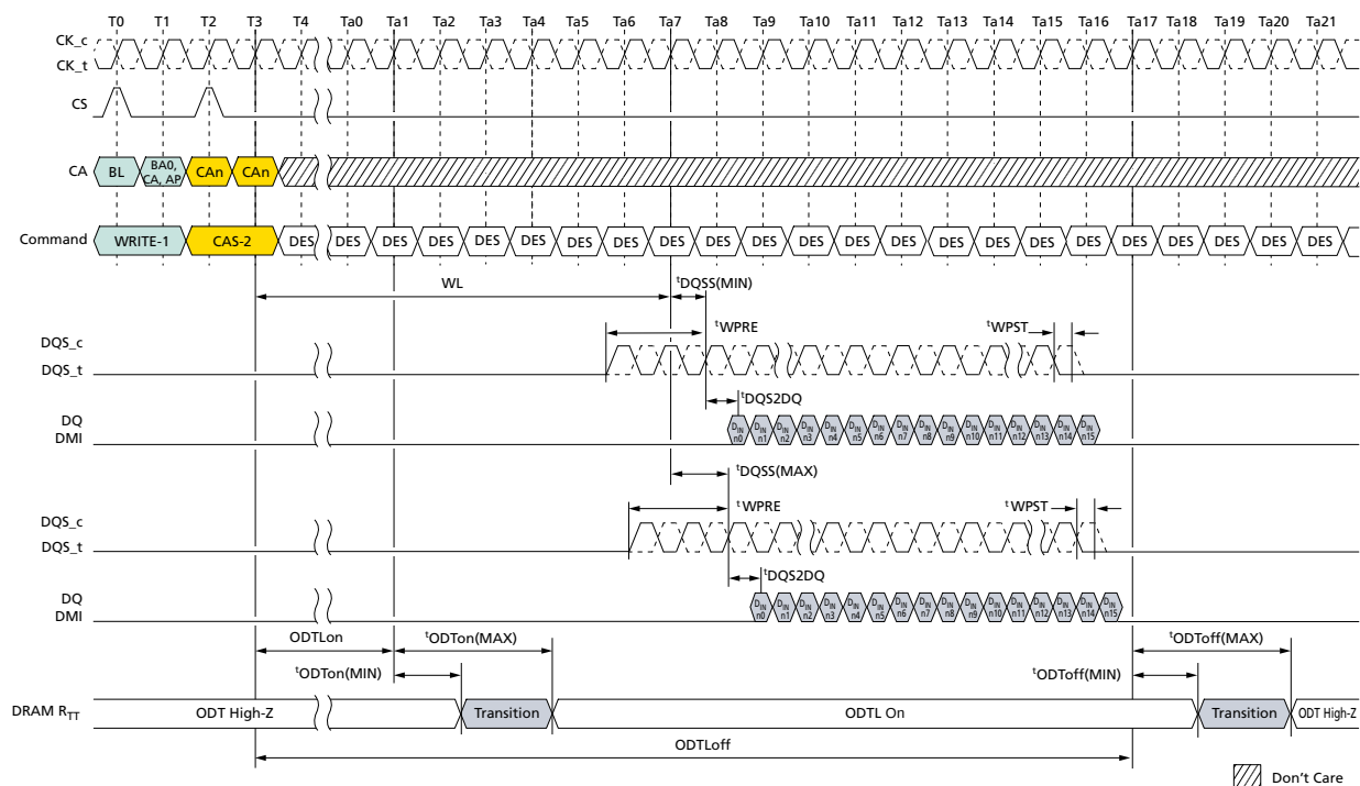
Figure 149: Asynchronous ODTon/ODToff Timing
