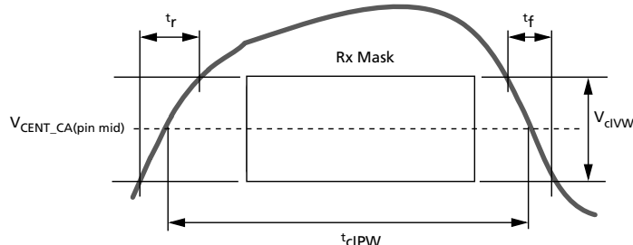
Figure 176: CA t_{cIPW} and SRIN_cIVW Definition (for Each Input Pulse)
