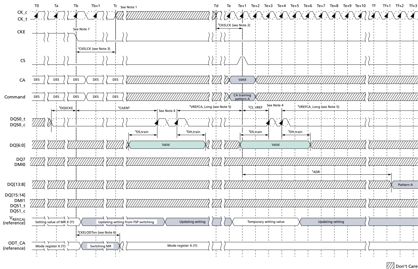
Figure 119: Consecutive V_{REF(CA)} Value Update
