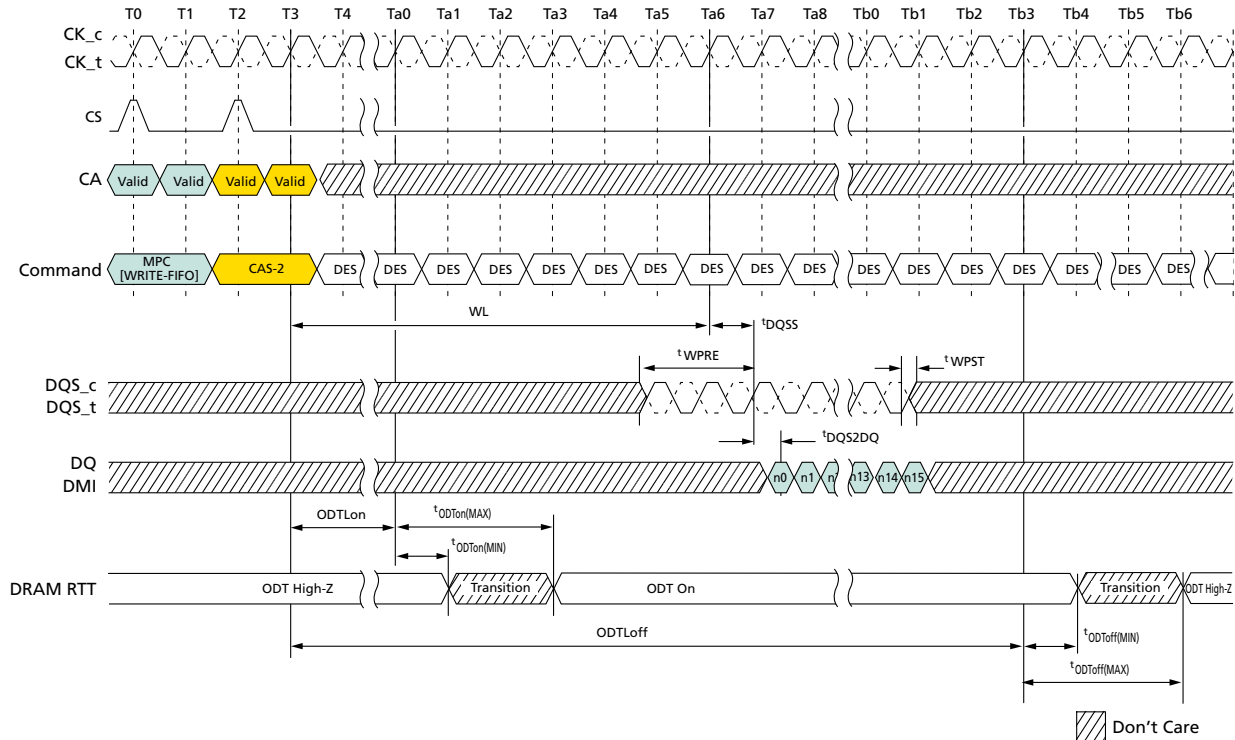
Figure 135: MPC[WRITE-FIFO] with DQ ODT Timing
