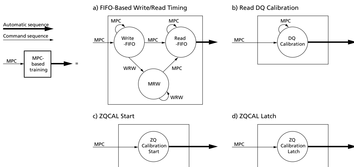
Figure 16: Simplified State Diagram
