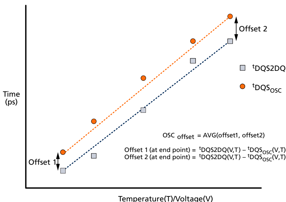
Figure 137: Interval Oscillator Offset – \text{OSC}_{\text{Offset}}
