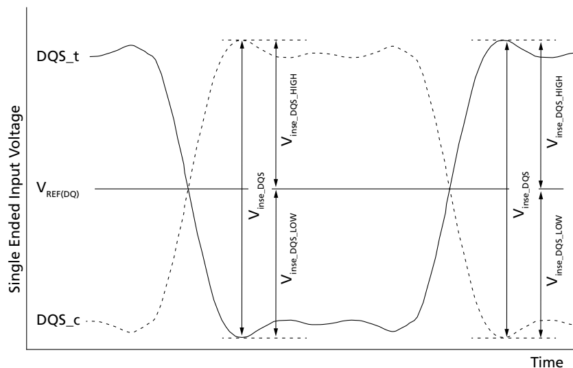
Figure 162: DQS Single-Ended Input Voltage
