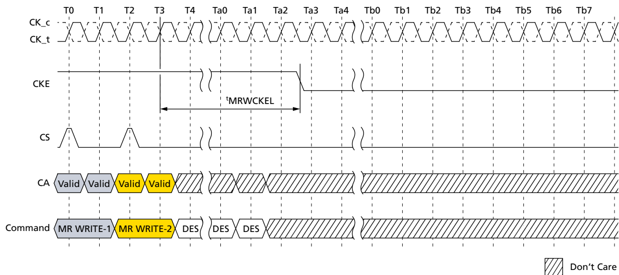
Figure 95: Mode Register Write to Power-Down Entry
