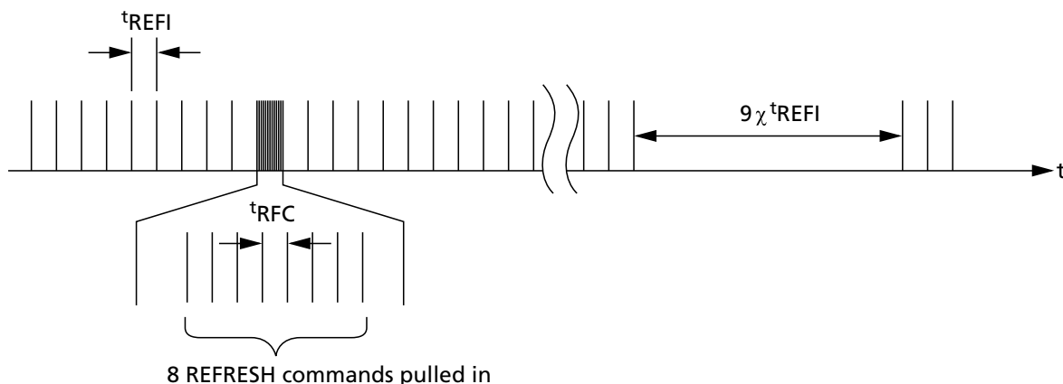
Figure 79: Pulling in REFRESH Commands (Example)
