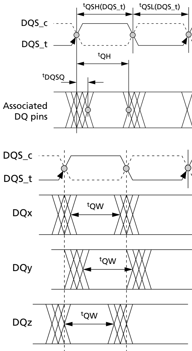
Figure 178: Read Data Timing Definitions – t_{QH} and t_{DQSQ} Across DQ Signals per DQS Group
