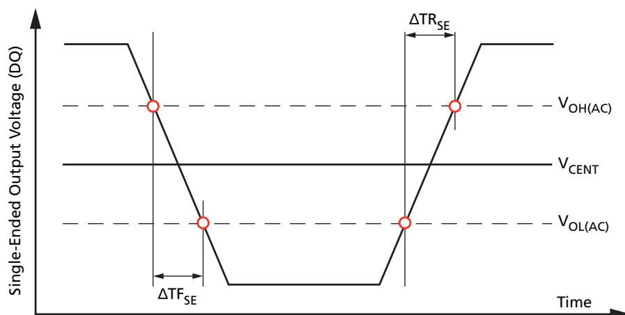
Figure 190: Single-Ended Output Slew Rate Definition
