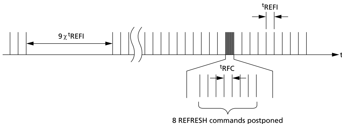
Figure 78: Postponing REFRESH Commands (Example)
