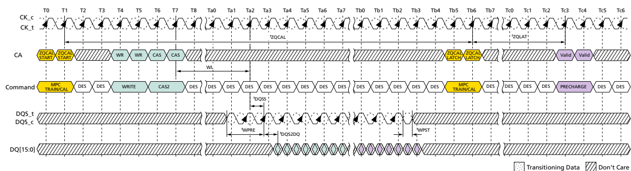
Figure 141: ZQCAL Timing
