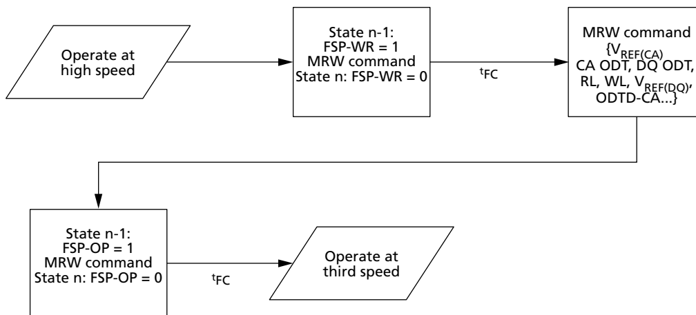
Figure 145: Example of Switching to a Third Trained Frequency Set Point
