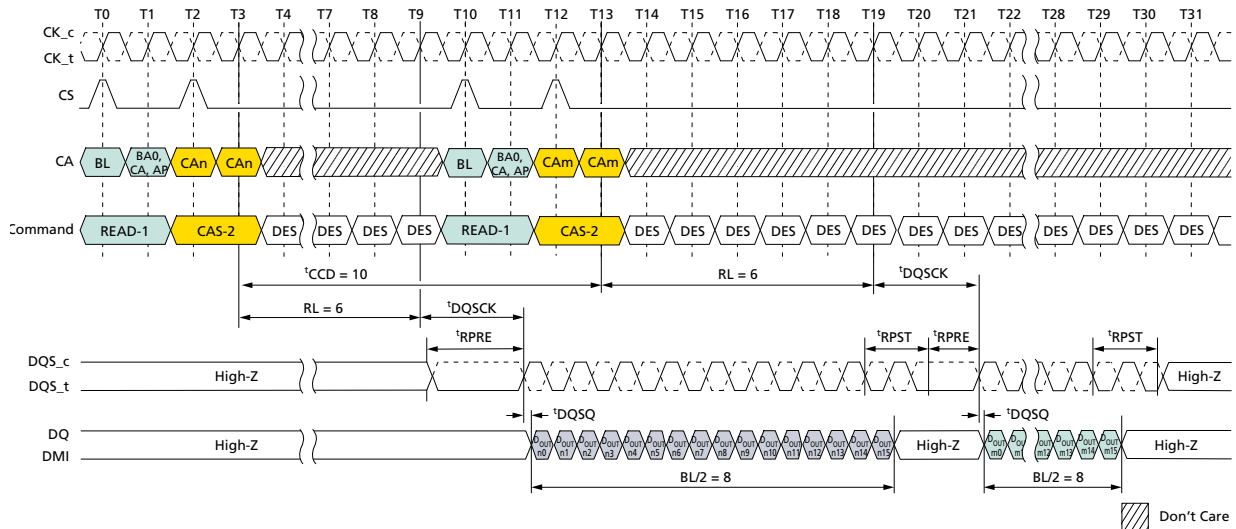
Figure 52: Consecutive READ: t_{CCD} = \text{MIN} + 2 , Preamble = Static, 1.5n\text{CK} Postamble
