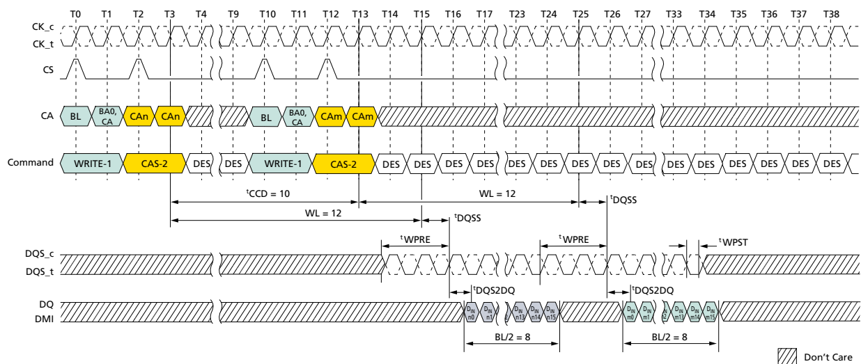
Figure 63: Consecutive WRITE: t_{CCD} = \text{MIN} + 2, 0.5n\text{CK} Postamble
