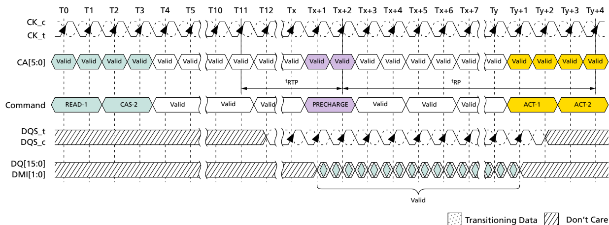
Figure 69: Burst READ Followed by Precharge – BL32, 2 t CK, 0.5nCK Postamble
