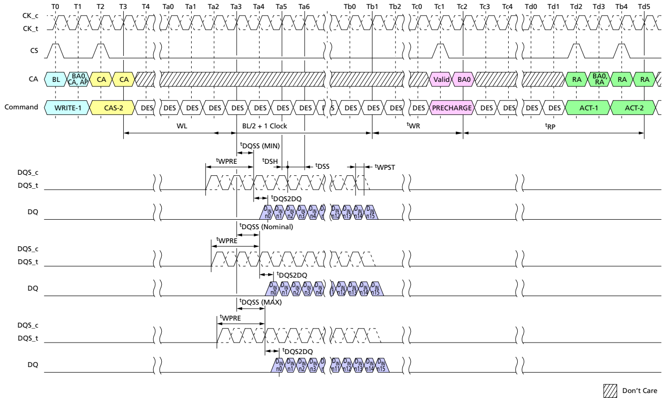
Figure 32: Burst WRITE Operation
