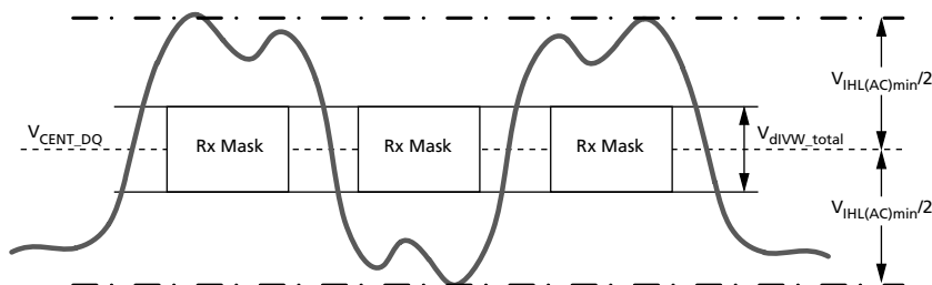
Figure 183: DQ V_{IHL(AC)} Definition (for Each Input Pulse)
