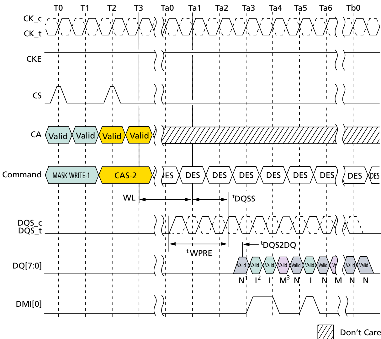
Figure 39: MASKED WRITE Command with Write DBI Enabled; DM Enabled
