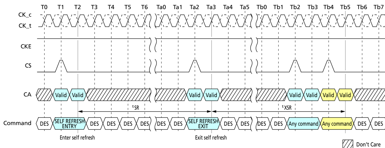
Figure 82: Self Refresh Entry/Exit Timing
