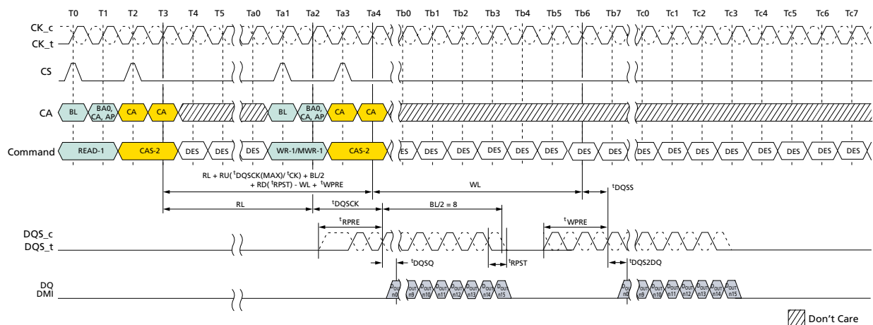
Figure 25: Burst Read Followed by Burst Write or Burst Mask Write
