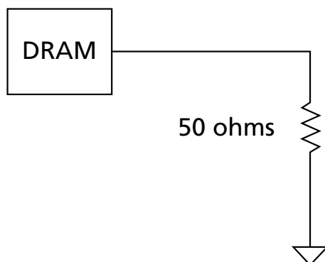
Figure 168: Driver Output Timing Reference Load
