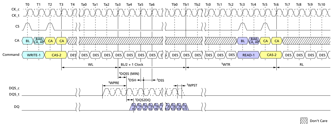
Figure 33: Burst Write Followed by Burst Read
