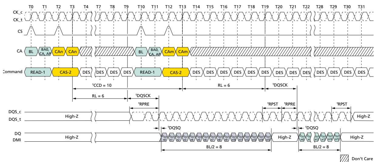
Figure 50: Consecutive READ: t_{CCD} = \text{MIN} + 2 , Preamble = Toggle, 1.5n\text{CK} Postamble
