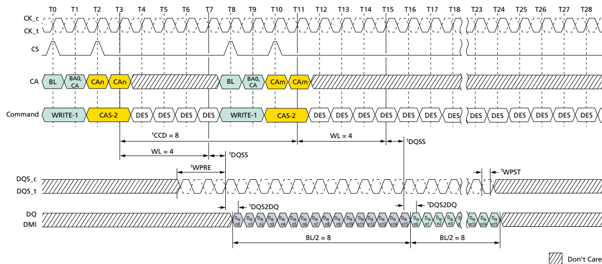
Figure 58: Seamless WRITE: t_{CCD} = \text{MIN} , 0.5n\text{CK} Postamble
