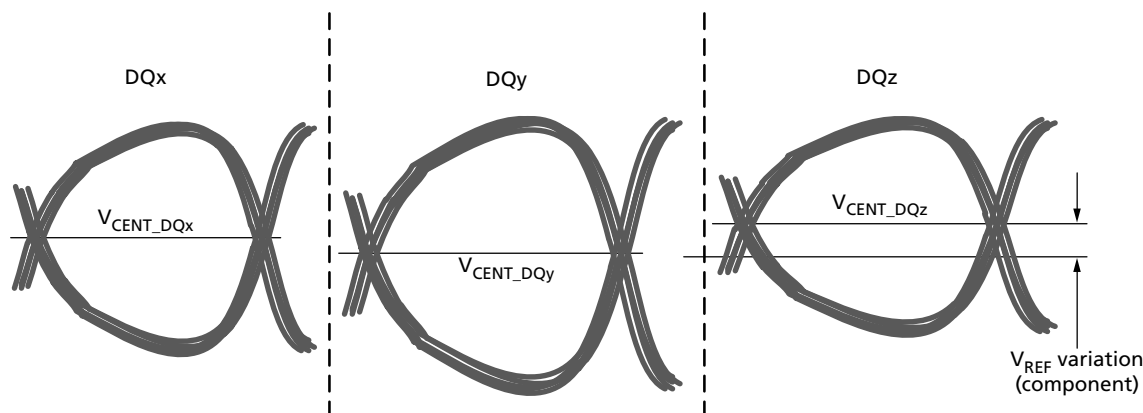
Figure 180: Across Pin V_{REF} DQ Voltage Variation
