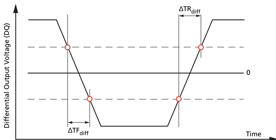
Figure 191: Differential Output Slew Rate Definition
