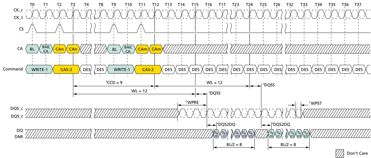
Figure 61: Consecutive WRITE: t_{CCD} = \text{MIN} + 1, 0.5nCK Postamble
