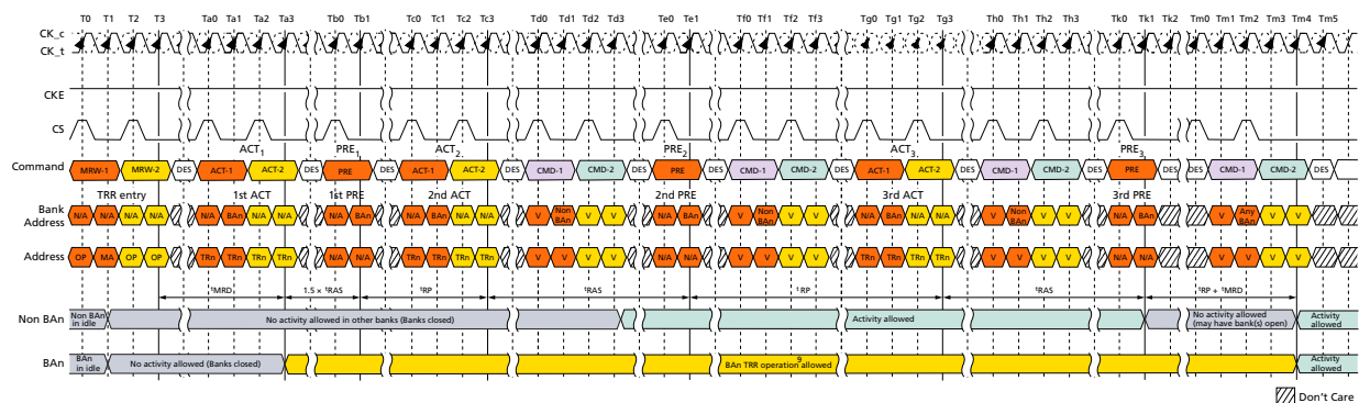
Figure 150: Target Row Refresh Mode
