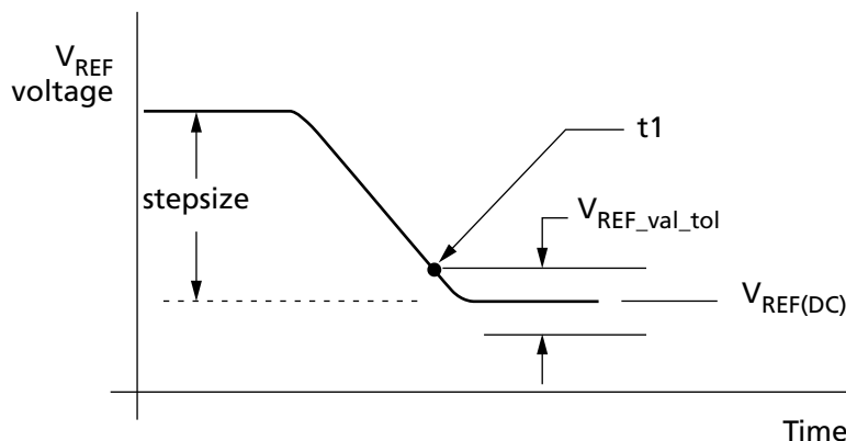
Figure 109: V_{REF(CA)} Full Step from V_{REF,min} to V_{REF,max}
