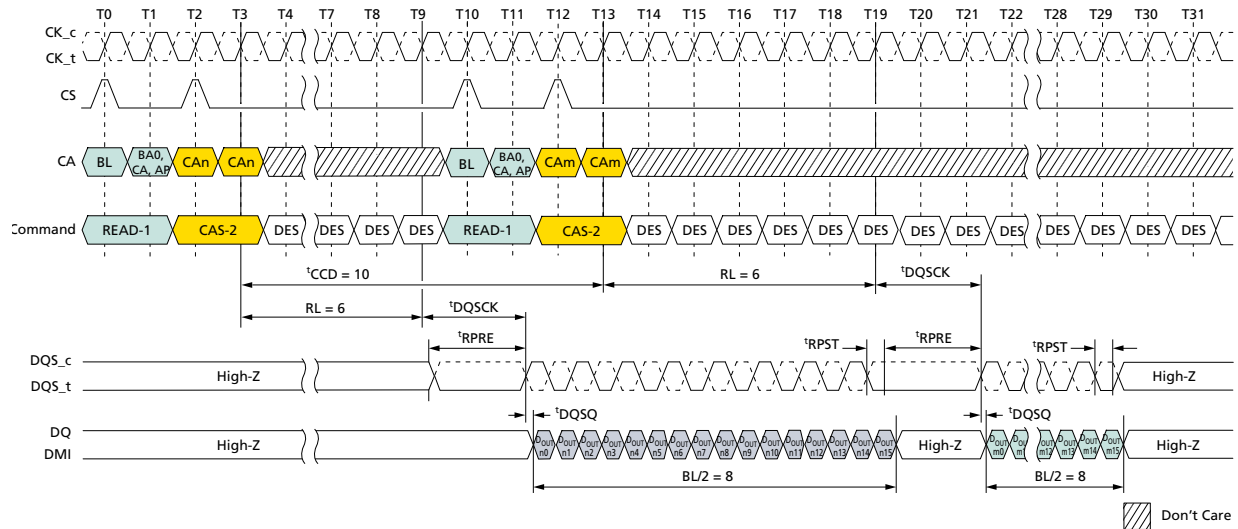
Figure 53: Consecutive READ: t_{CCD} = \text{MIN} + 2 , Preamble = Static, 0.5n\text{CK} Postamble
