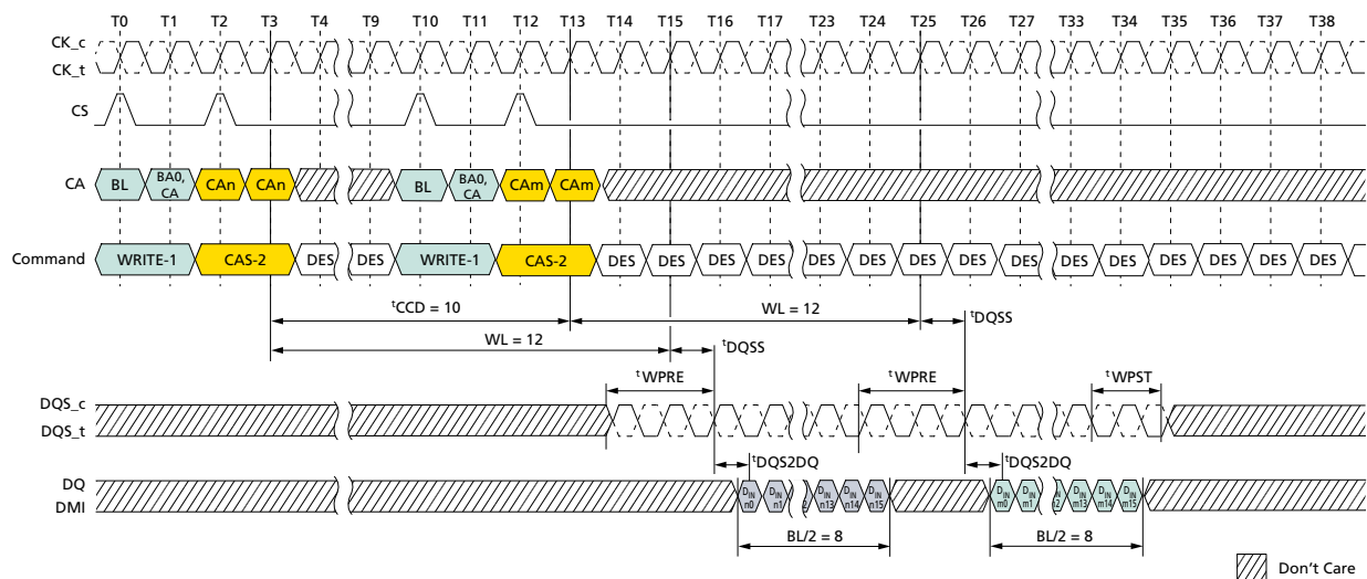
Figure 64: Consecutive WRITE: t_{CCD} = \text{MIN} + 2, 1.5n\text{CK} Postamble
