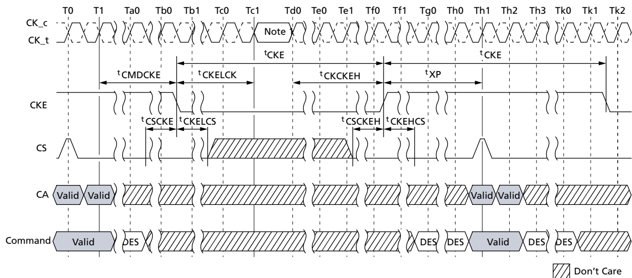
Figure 87: Basic Power-Down Entry and Exit Timing
