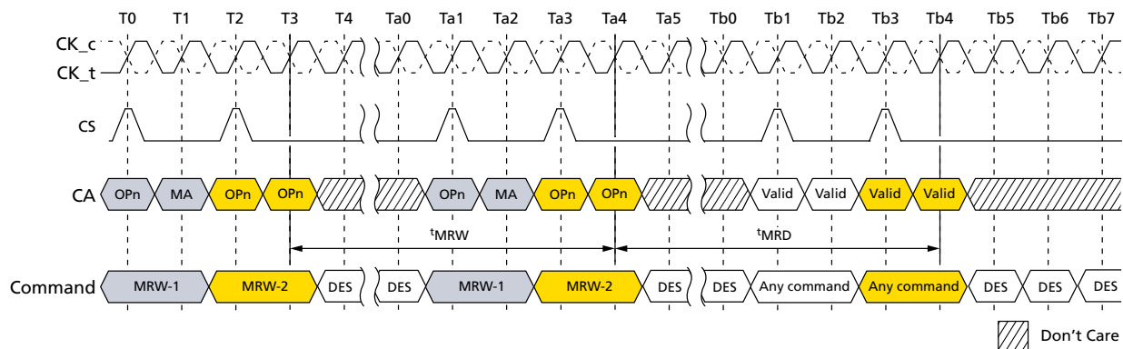
Figure 101: MODE REGISTER WRITE Timing
