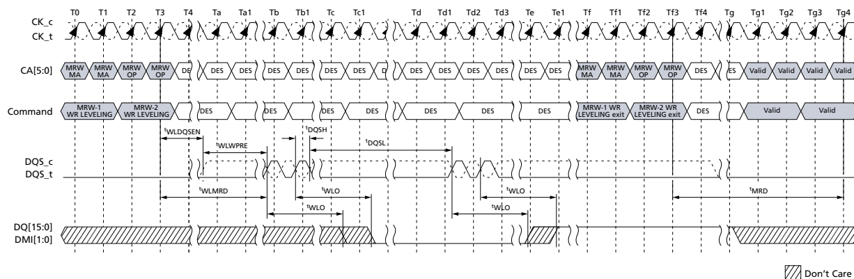
Figure 122: Write Leveling Timing – t_{DQSL}(\text{MAX})
