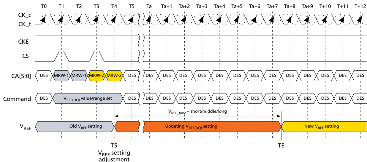
Figure 113: V_{REF(DQ)} Transition Time for Short, Middle, or Long Changes
