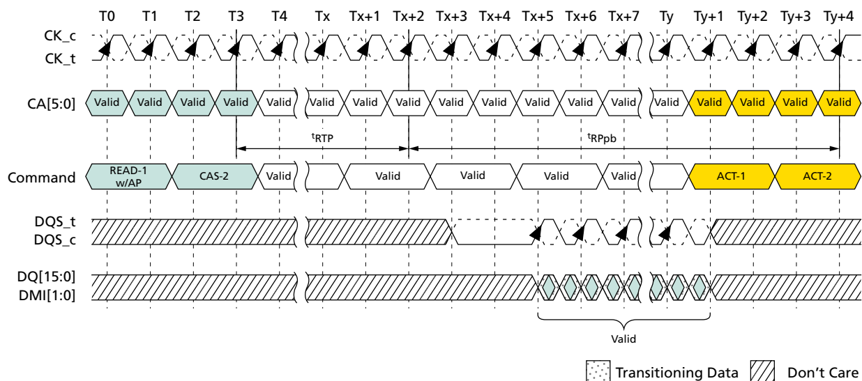
Figure 72: Burst READ With Auto Precharge – BL32, Toggling Preamble, 1.5nCK Postamble
