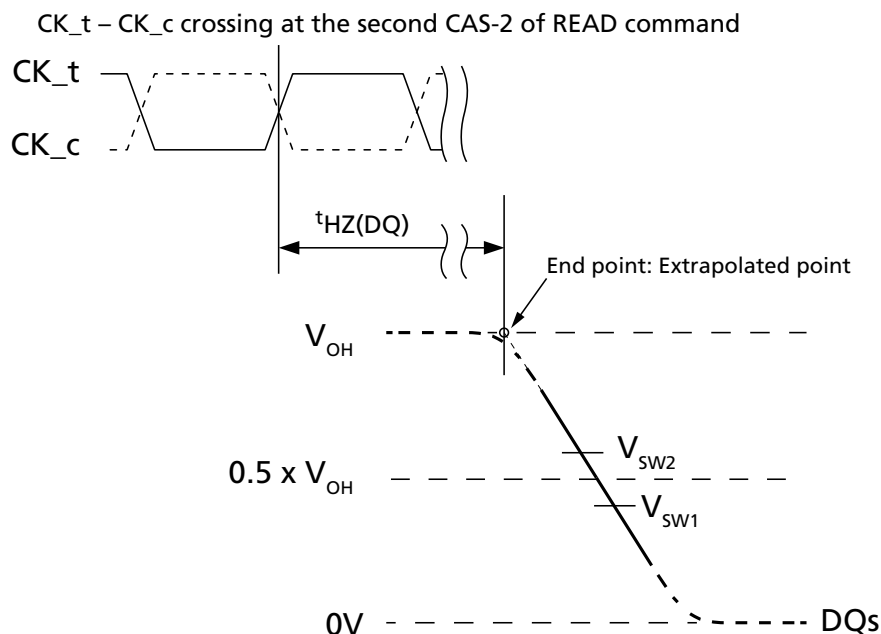
Figure 187: t_{HZ}(DQ) Method for Calculating Transitions and Endpoint
