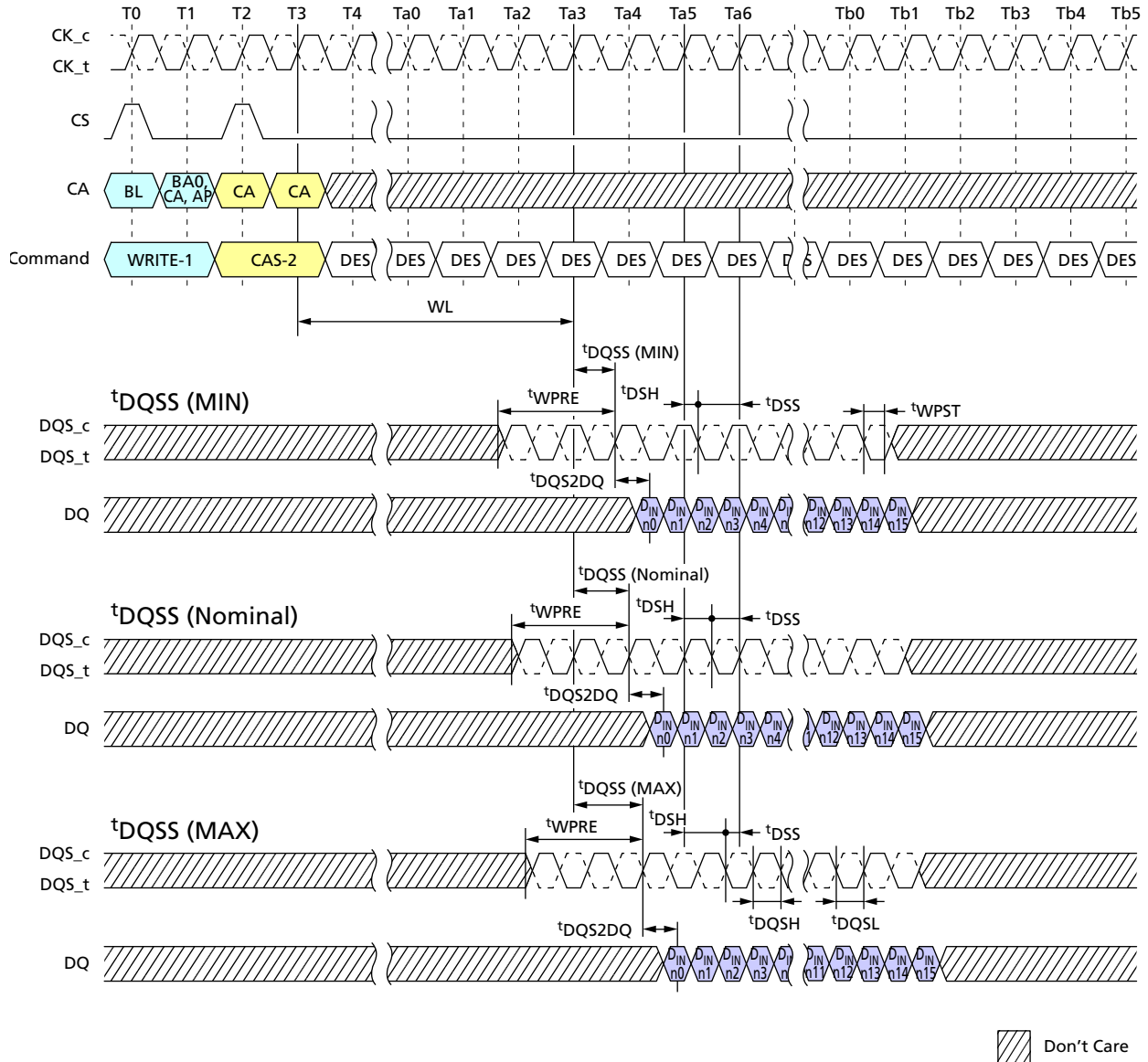
Figure 34: Write Timing
