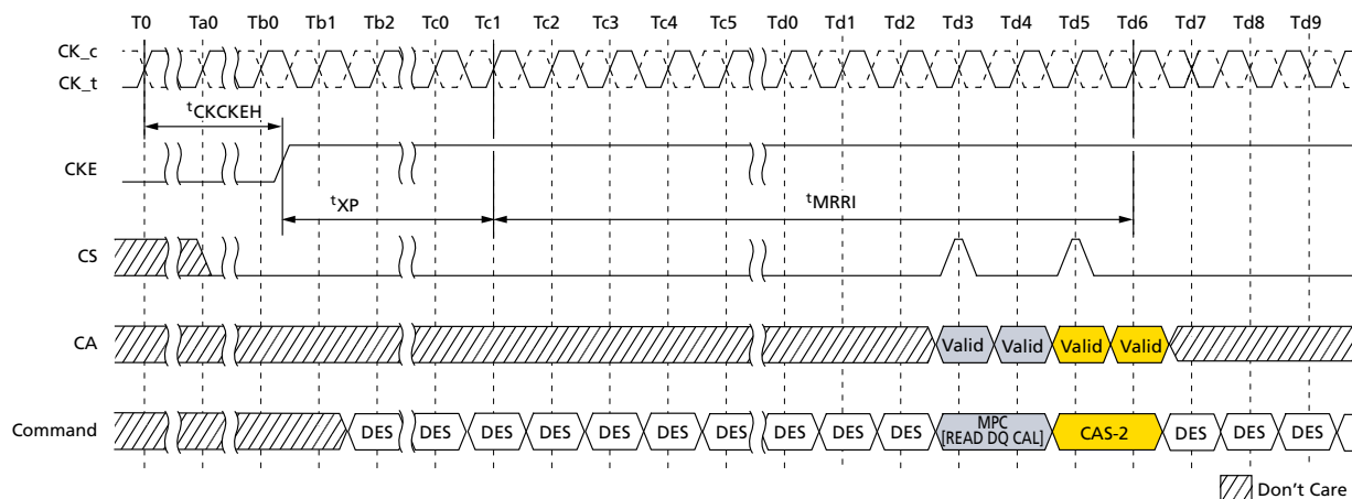
Figure 131: MPC[READ DQ CALIBRATION] Following Power-Down State
