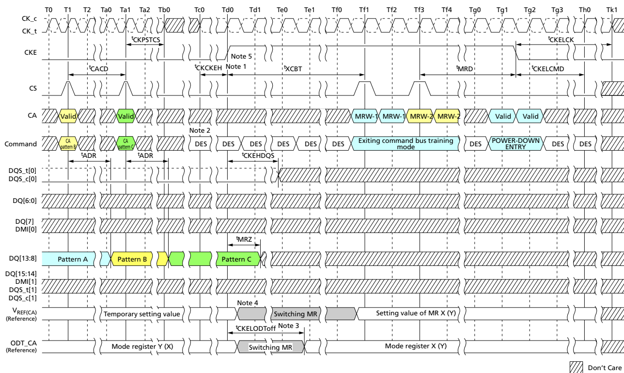
Figure 121: Command Bus Training Mode Exit with Power-Down Entry
