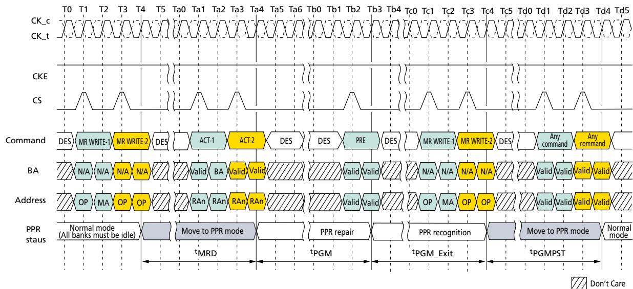
Figure 151: Post-Package Repair Timing
