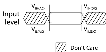
Figure 153: Input Timing Definition for CKE
