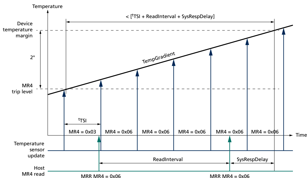
Figure 140: Temperature Sensor Timing
