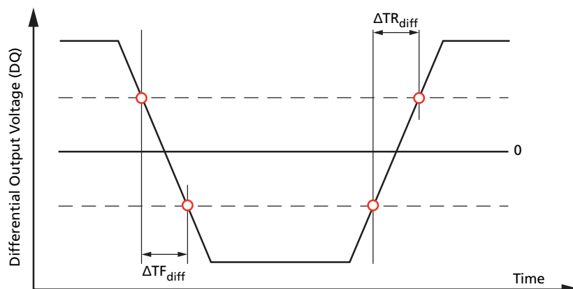
Figure 166: Differential Output Slew Rate Definition
