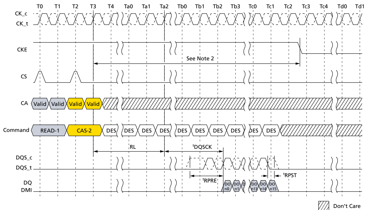
Figure 88: Read and Read with Auto Precharge to Power-Down Entry
