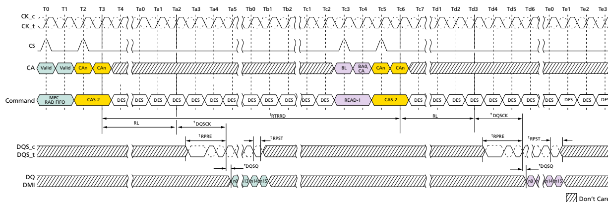
Figure 134: MPC[READ-FIFO] to Read Timing
