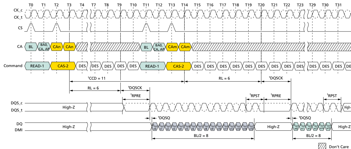
Figure 56: Consecutive READ: t_{CCD} = \text{MIN} + 3 , Preamble = Static, 1.5nCK Postamble
