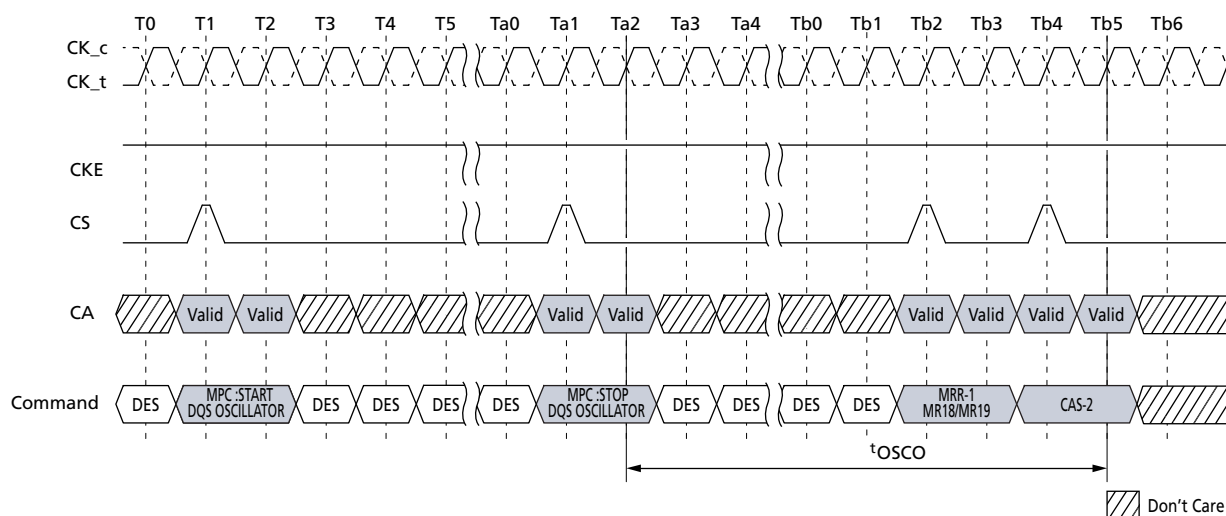
Figure 138: In Case of DQS Interval Oscillator is Stopped by MPC Command
