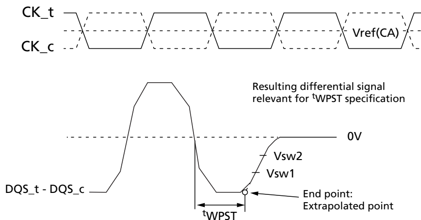
Figure 36: Method for Calculating t WPST Transitions and Endpoints
