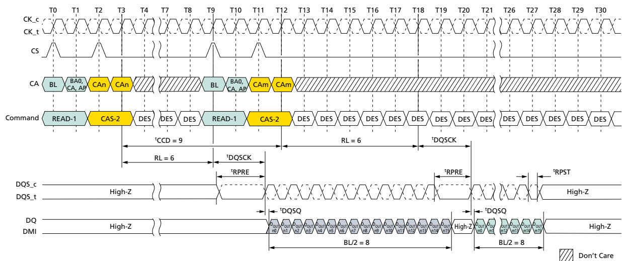
Figure 49: Consecutive READ: t_{CCD} = \text{MIN} + 1 , Preamble = Static, 0.5n\text{CK} Postamble
