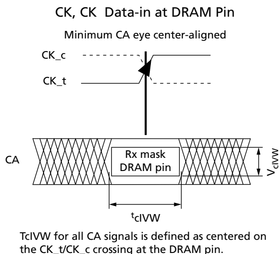
Figure 175: CA Timings at the DRAM Pins
