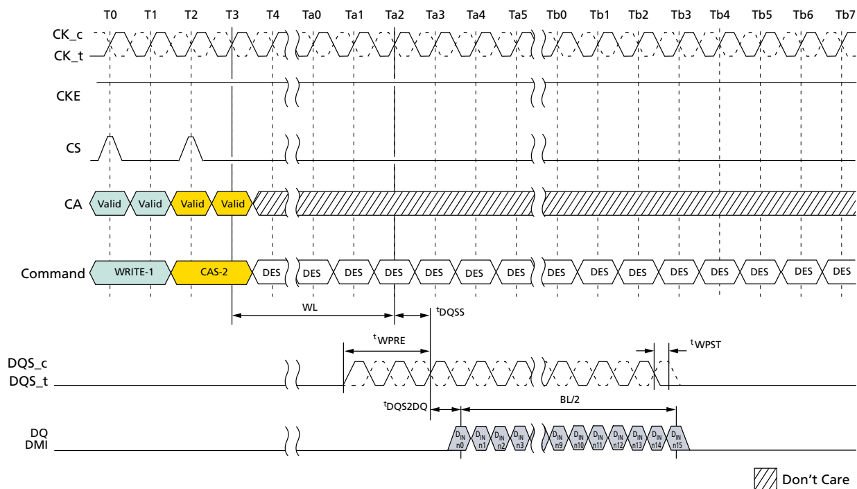
Figure 22: DQS Write Preamble and Postamble – 0.5nCK Postamble
