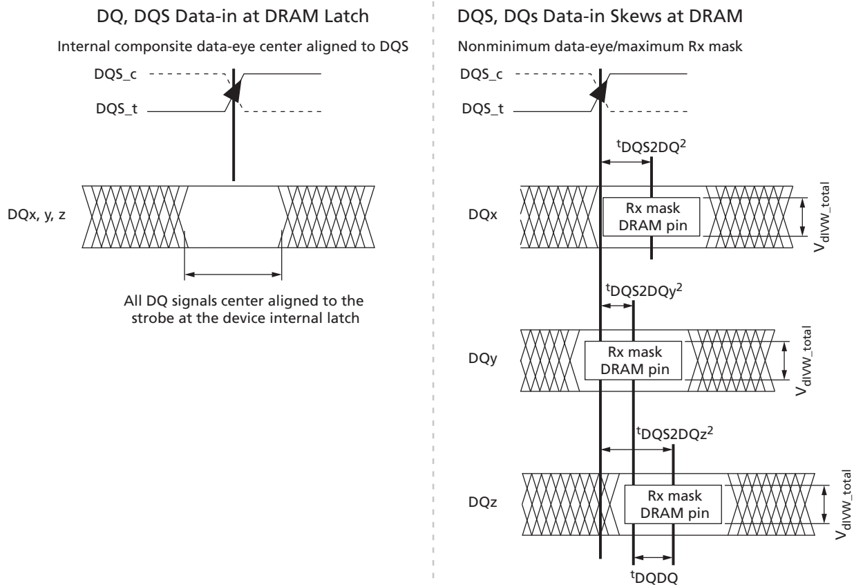
Figure 181: DQ-to-DQS t_{DQS2DQ} and t_{DQDQ}
