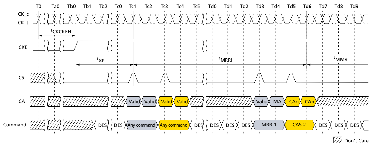
Figure 100: MRR Following Power-Down
