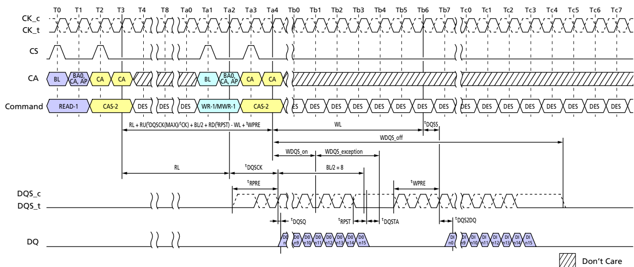
Figure 43: Burst READ Followed by Burst WRITE or Burst MASKED WRITE (ODT Disable)
