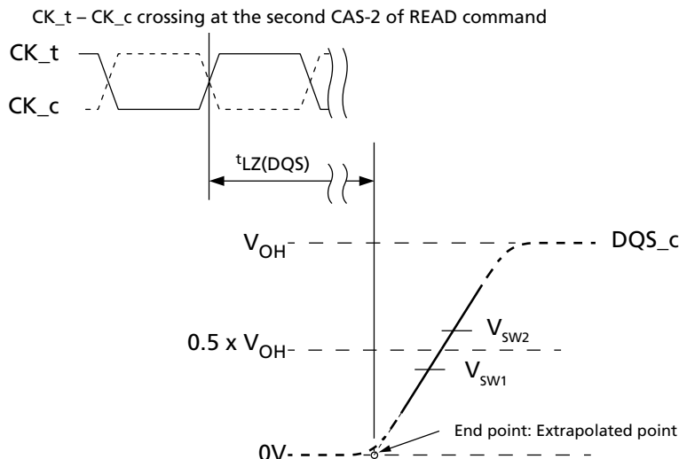
Figure 28: tLZ(DQS) Method for Calculating Transitions and Endpoint
