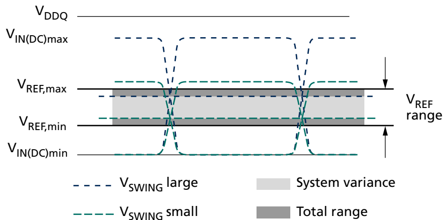
Figure 111: V_{REF} Operating Range ( V_{REF,max} , V_{REF,min} )
