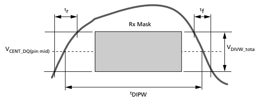
Figure 182: DQ t_{DIPW} and SRIN_dIVW Definition for Each Input Pulse
