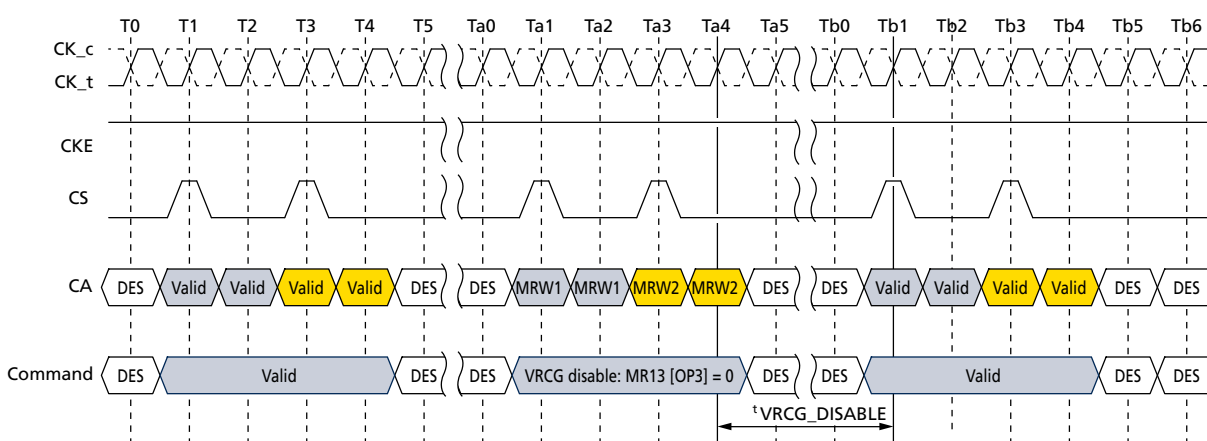
Figure 103: VRCG Disable Timing
