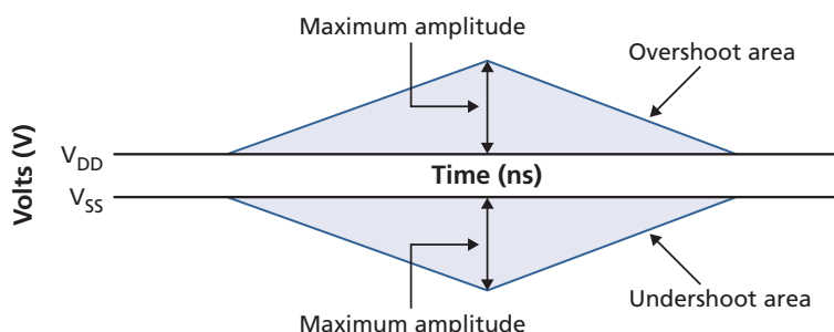
Figure 167: Overshoot and Undershoot Definition
