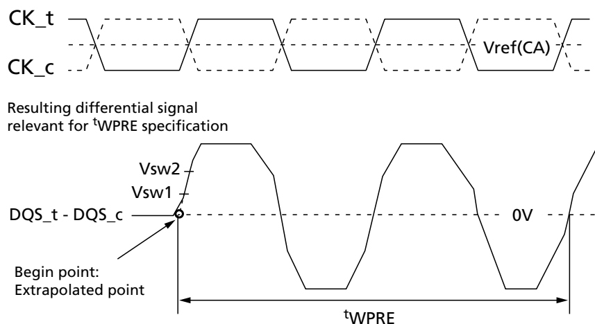
Figure 35: Method for Calculating t WPRE Transitions and Endpoints
