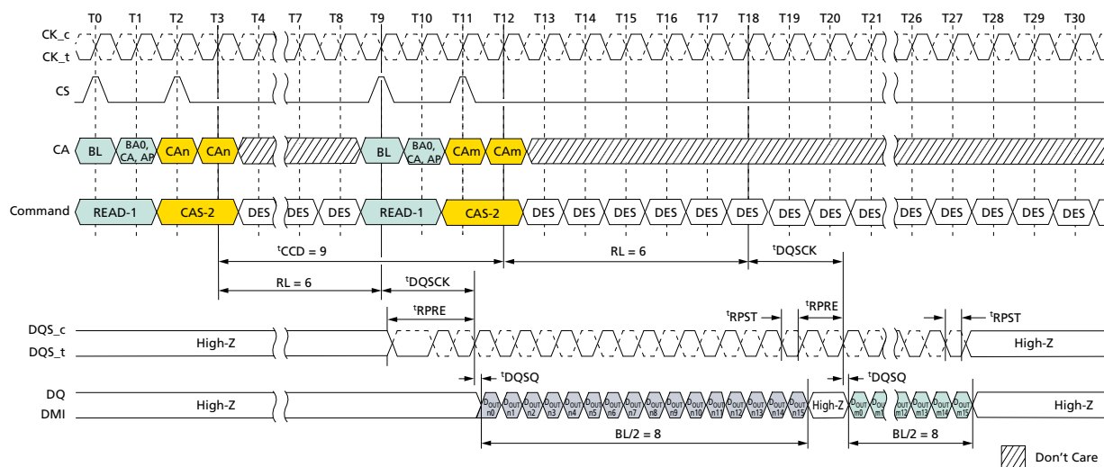
Figure 47: Consecutive READ: t_{CCD} = \text{MIN} + 1 , Preamble = Toggle, 0.5n\text{CK} Postamble
