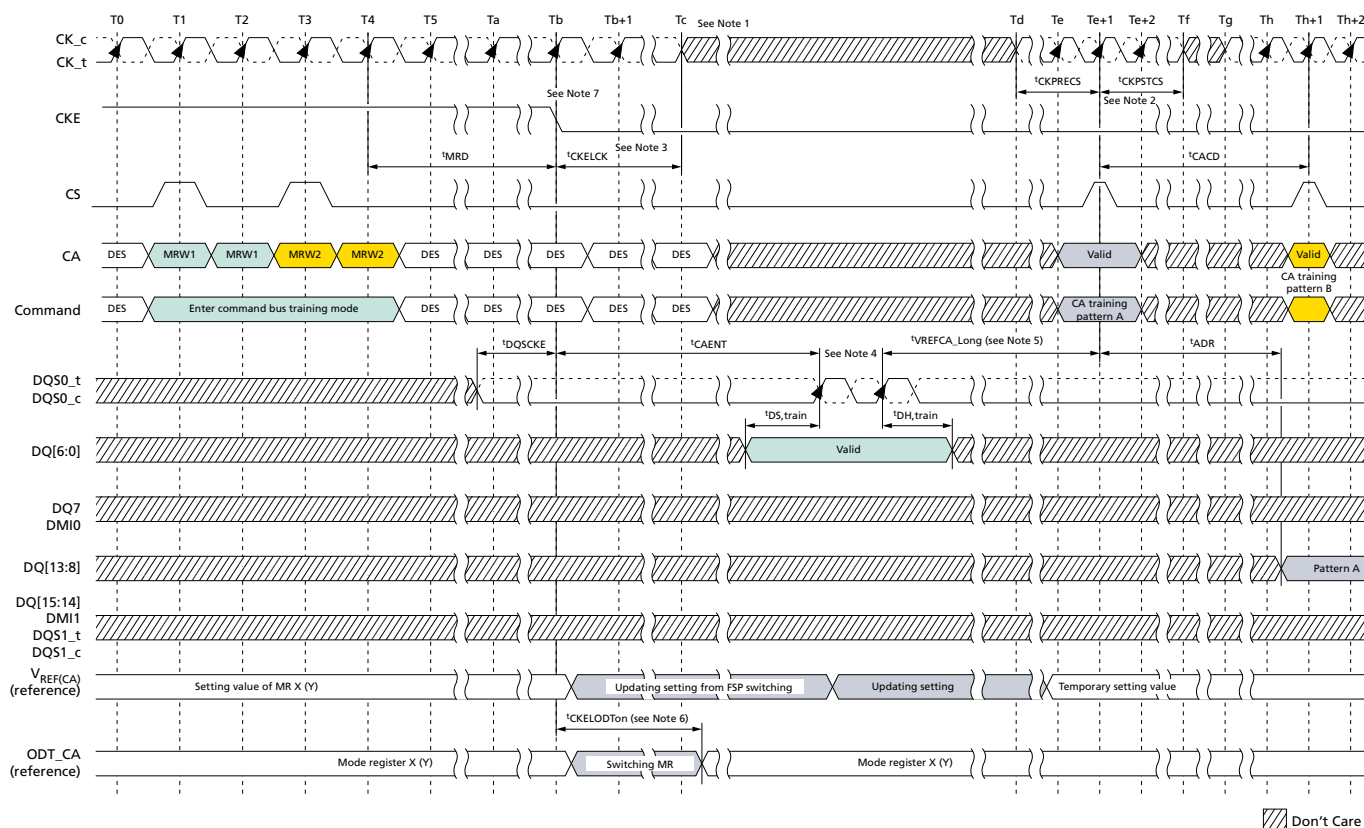
Figure 118: Command Bus Training Mode Entry – CA Training Pattern I/O with V_{REF(CA)} Value Update
