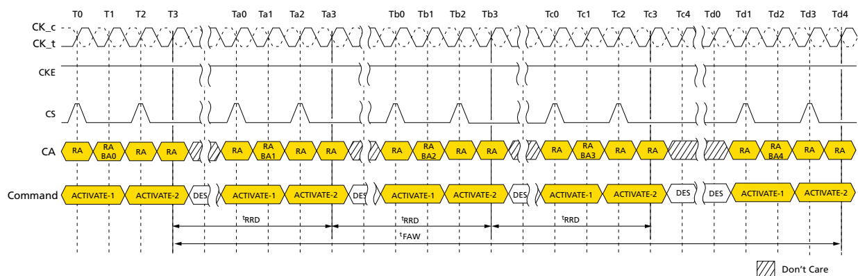
Figure 19: t_{FAW} Timing
