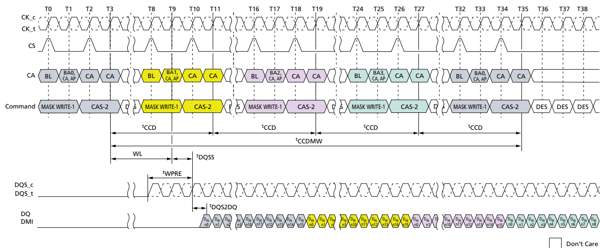
Figure 38: MASK WRITE Command – Different Bank
