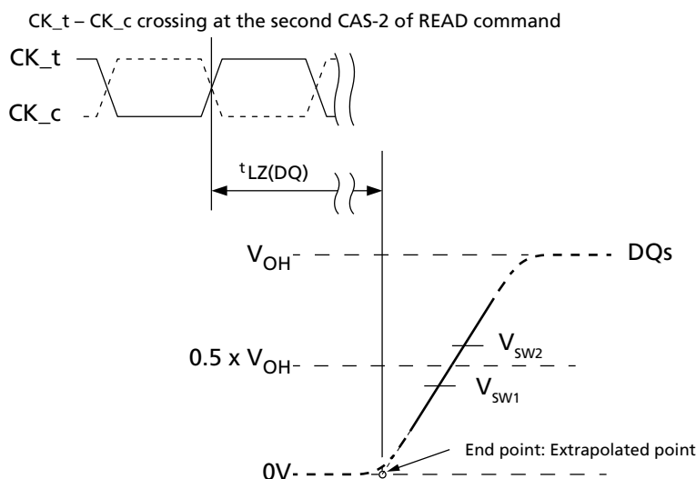
Figure 30: t_{LZ}(DQ) Method for Calculating Transitions and Endpoint
