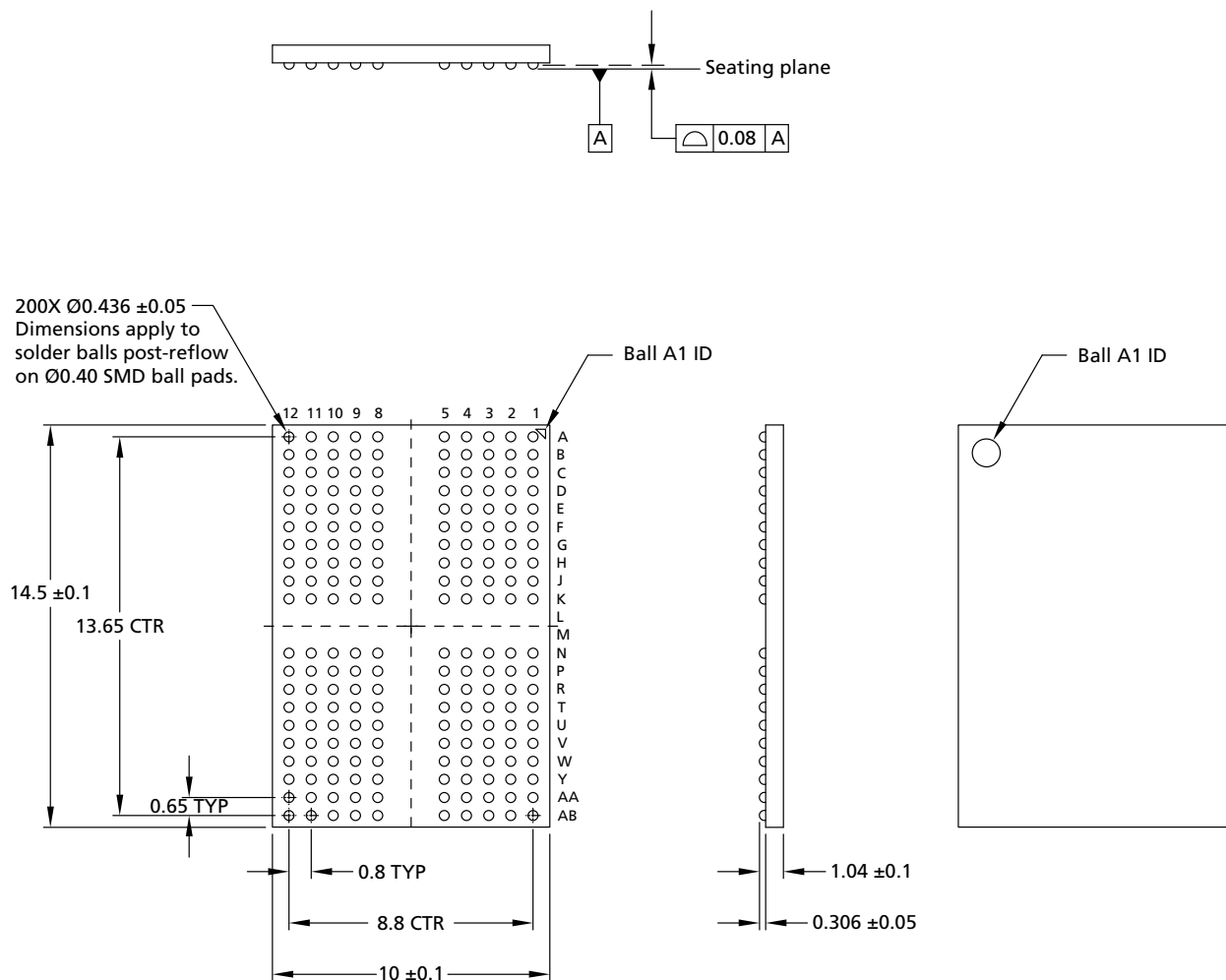
Figure 13: 200-Ball TFBGA – 10mm x 14.5mm x 1.14mm (Package Code: DE)
