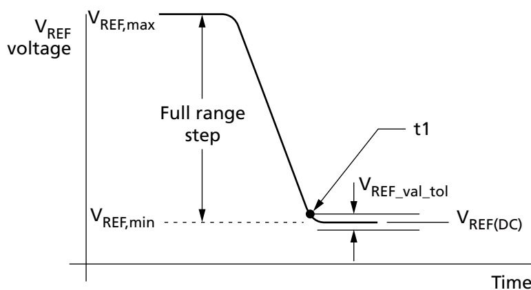
Figure 117: V_{REF(DQ)} Full Step from V_{REF,max} to V_{REF,min}
