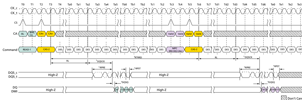
Figure 129: Read DQ Calibration Training Timing: Read-to-Read DQ Calibration
