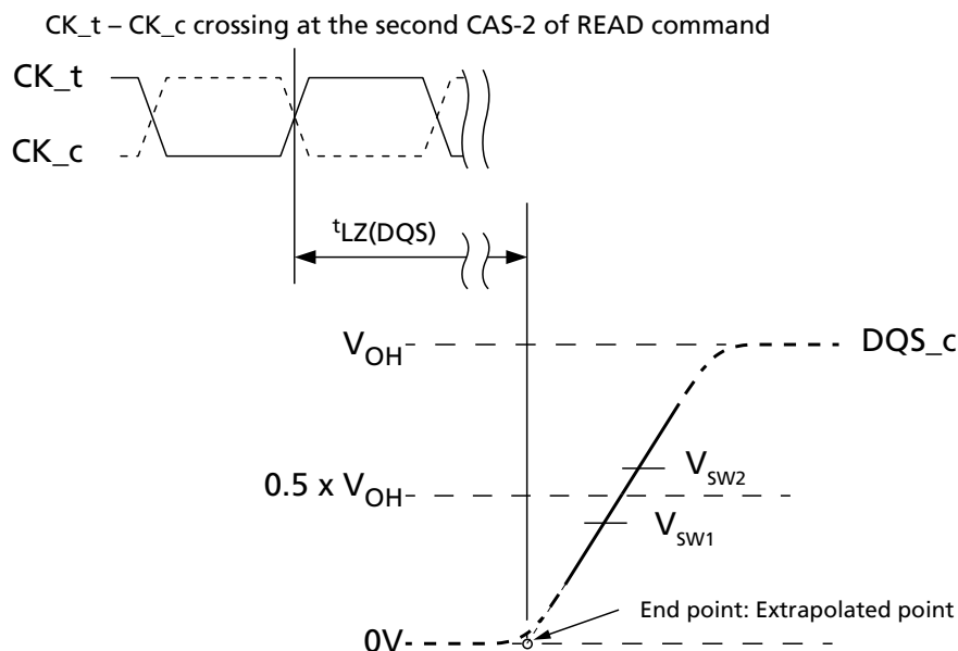
Figure 184: t_{LZ}(DQS) Method for Calculating Transitions and Endpoint
