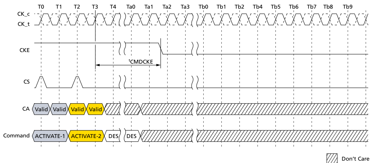
Figure 92: ACTIVATE Command to Power-Down Entry
