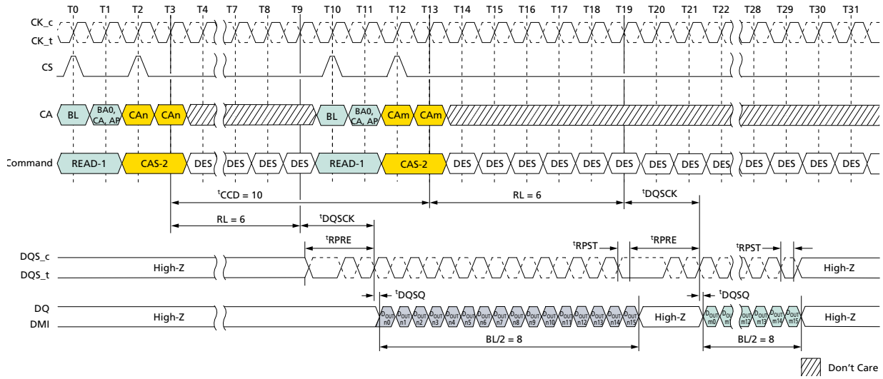
Figure 51: Consecutive READ: t_{CCD} = \text{MIN} + 2 , Preamble = Toggle, 0.5n\text{CK} Postamble
