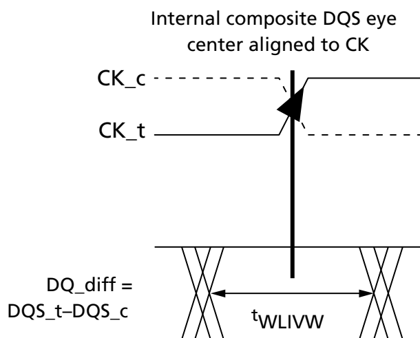
Figure 125: DQS_t/DQS_c to CK_t/CK_c Timings at the Pins Referenced from the Internal Latch
