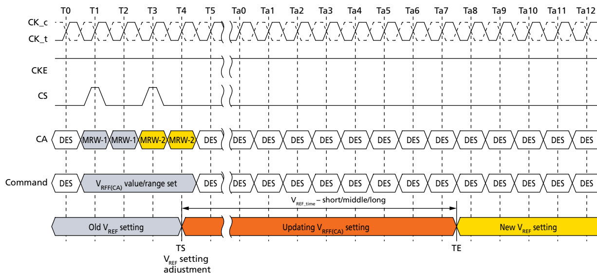
Figure 106: t_{V_{ref}} for Short, Middle, and Long Timing Diagram
