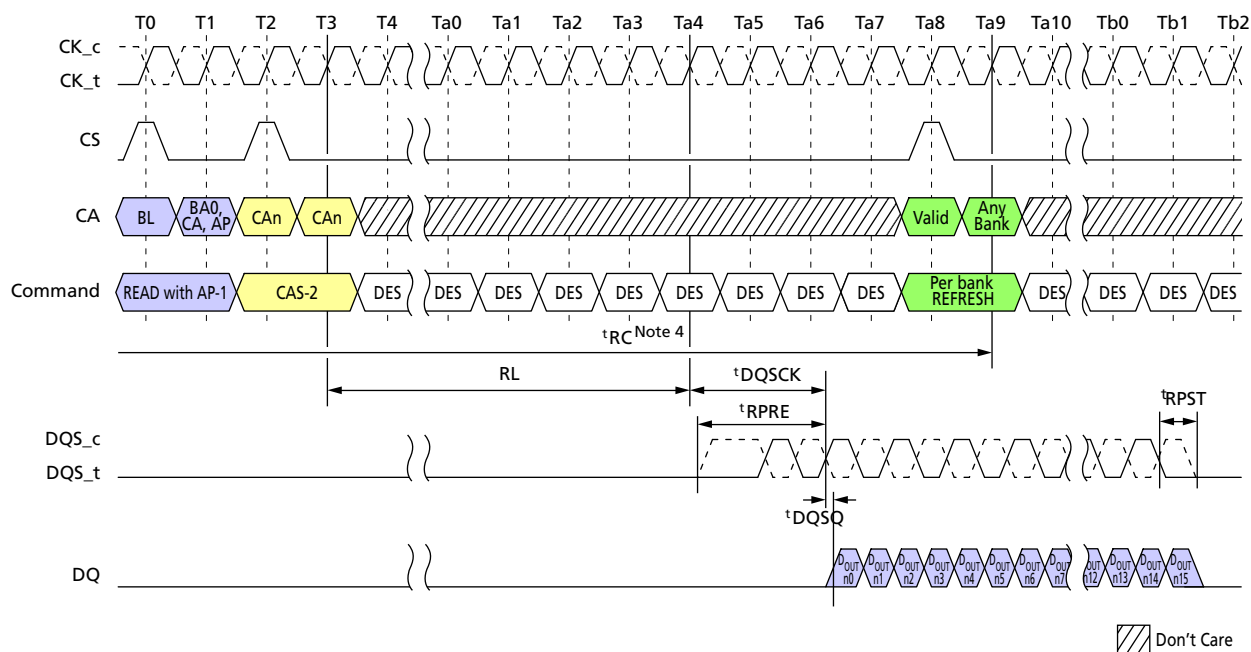
Figure 81: Burst READ With AUTO PRECHARGE Operation Followed by Per-Bank Refresh
