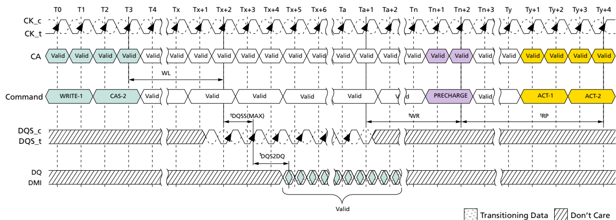
Figure 70: Burst WRITE Followed by PRECHARGE – BL16, 2nCK Preamble, 0.5nCK Postamble
