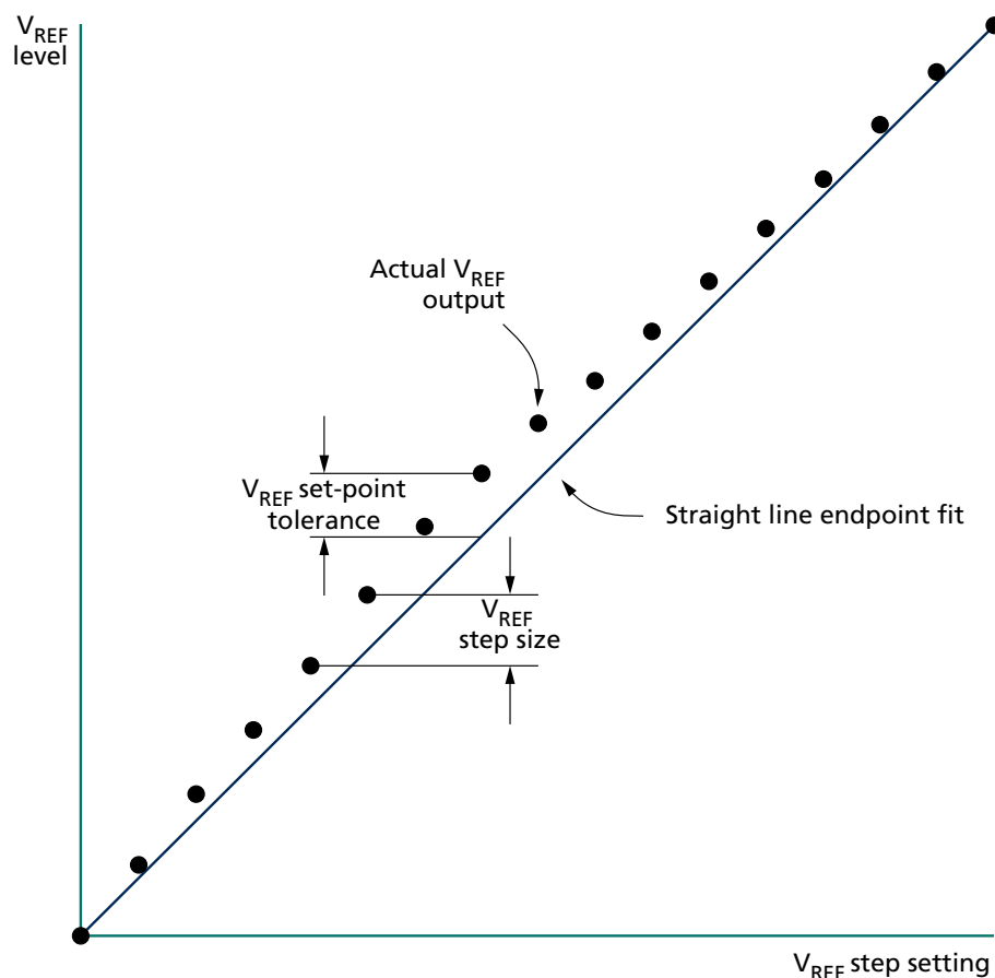
Figure 112: V_{REF} Set Tolerance and Step Size
