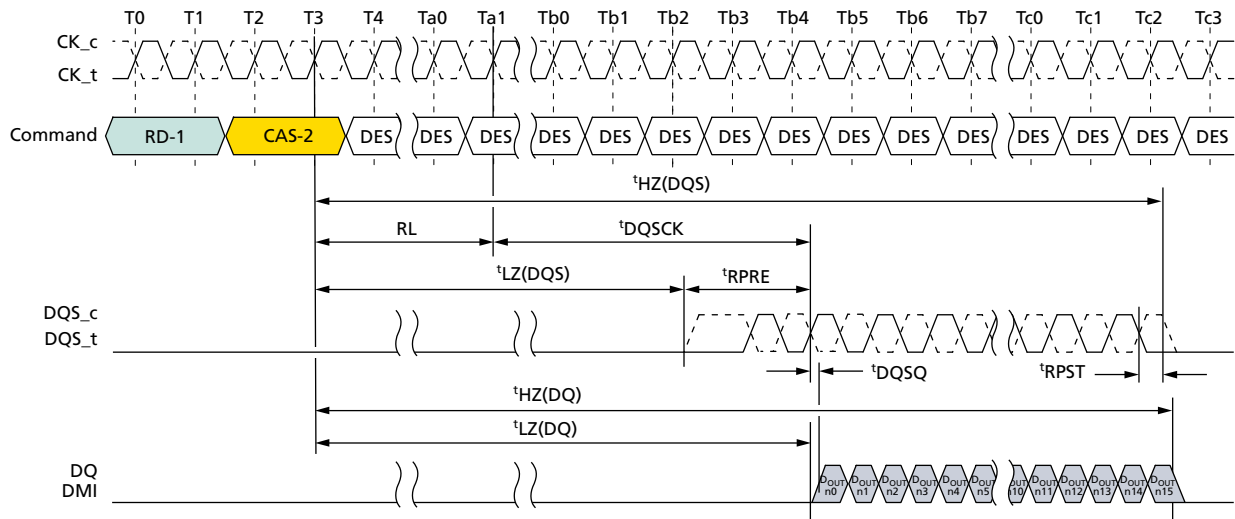
Figure 27: Read Timing
