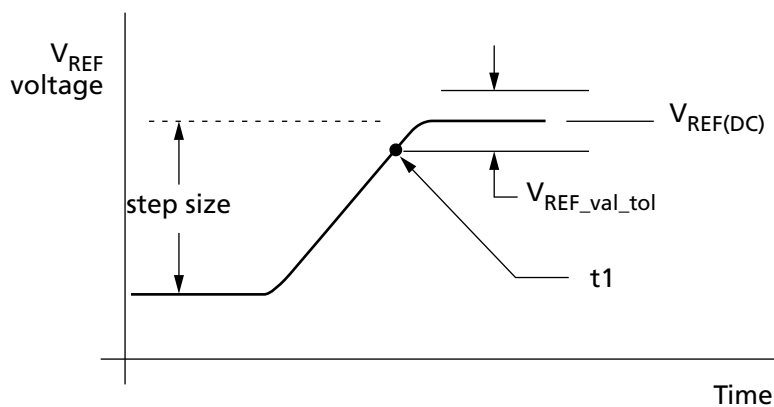
Figure 114: V_{REF(DQ)} Single-Step Size Increment
