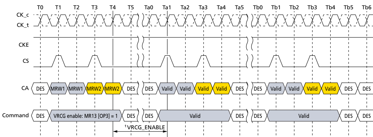
Figure 102: VRCG Enable Timing
