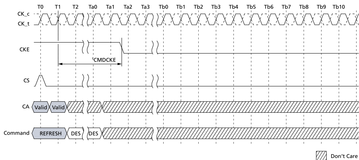
Figure 91: Refresh Entry to Power-Down Entry
