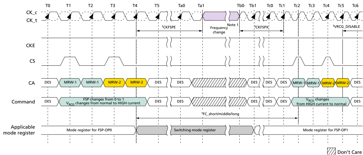
Figure 142: Frequency Set Point Switching Timing
