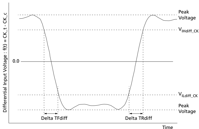
Figure 158: Differential Input Slew Rate Definition for CK_t, CK_c
