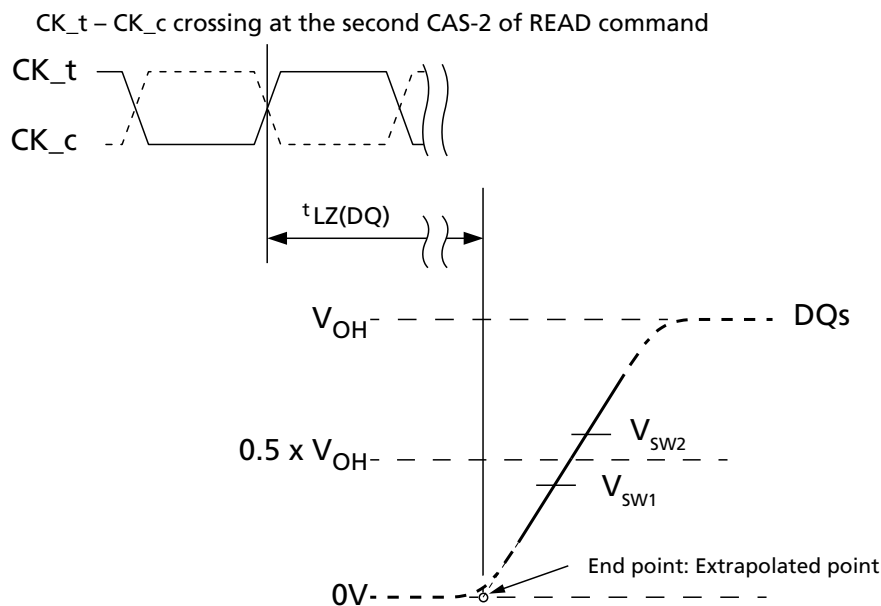
Figure 186: t_{LZ}(DQ) Method for Calculating Transitions and Endpoint
