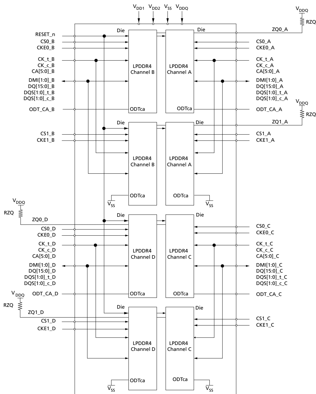
Figure 6: Eight-Die, Quad-Channel Package Block Diagram
