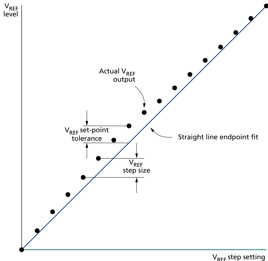
Figure 105: V_{REF} Set-Point Tolerance and Step Size
