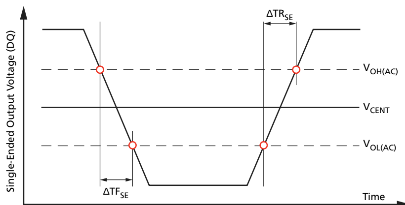
Figure 165: Single-Ended Output Slew Rate Definition
