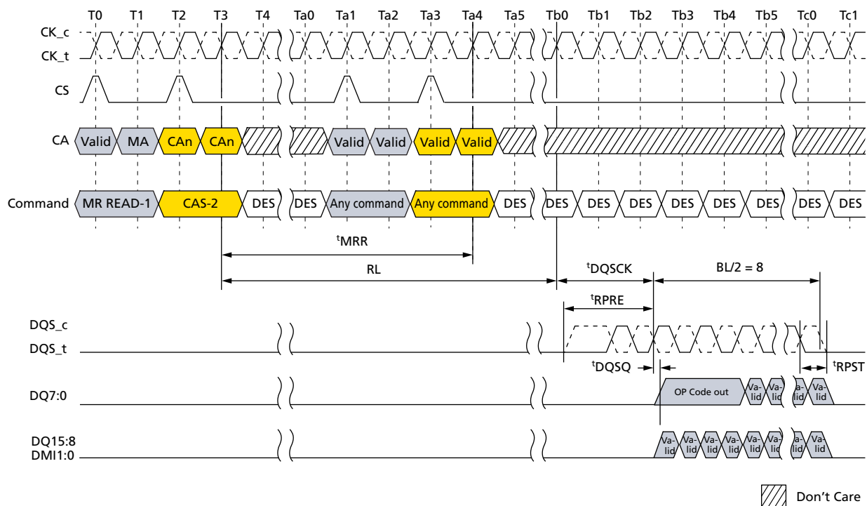
Figure 97: MODE REGISTER READ Operation
