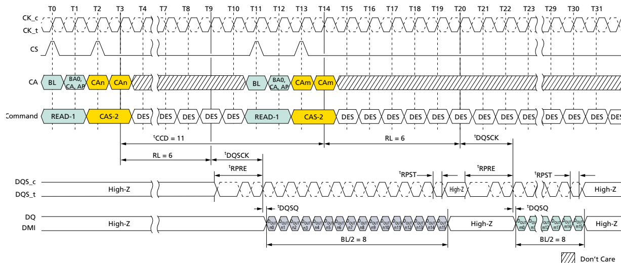
Figure 55: Consecutive READ: t_{CCD} = \text{MIN} + 3 , Preamble = Toggle, 0.5nCK Postamble
