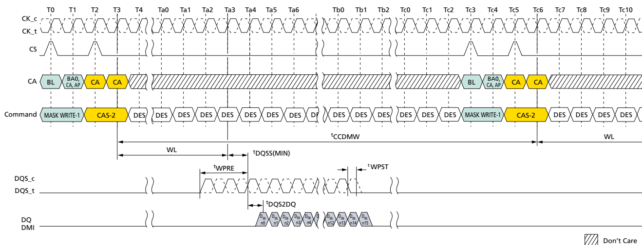
Figure 37: MASK WRITE Command – Same Bank
