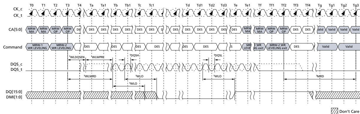
Figure 123: Write Leveling Timing – t_{DQSL}(\text{MIN})
