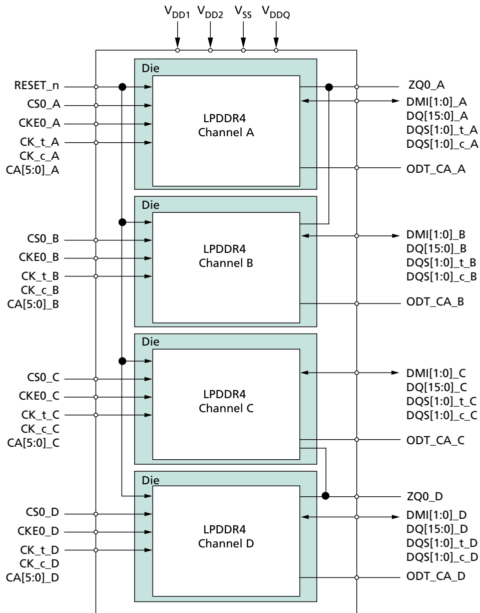
Figure 5: Quad-Die, Quad-Channel Package Block Diagram
