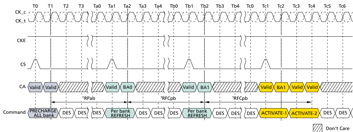
Figure 77: Per-Bank REFRESH Operation
