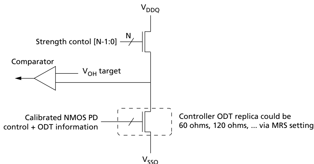
Figure 170: Pull-Up Calibration
