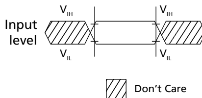
Figure 154: Input Timing Definition for RESET_n
