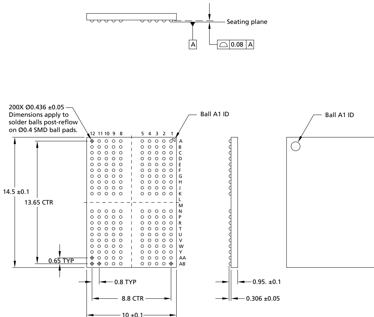
Figure 12: 200-Ball TFBGA – 10mm x 14.5mm x 1.05mm (Package Code: ZW)
