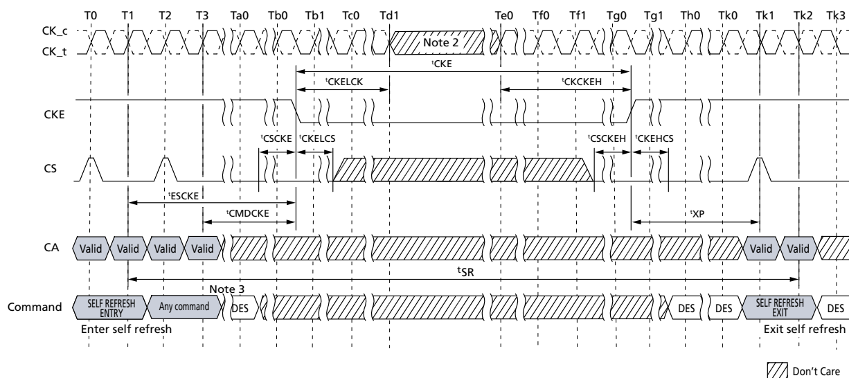
Figure 83: Self Refresh Entry/Exit Timing with Power-Down Entry/Exit
