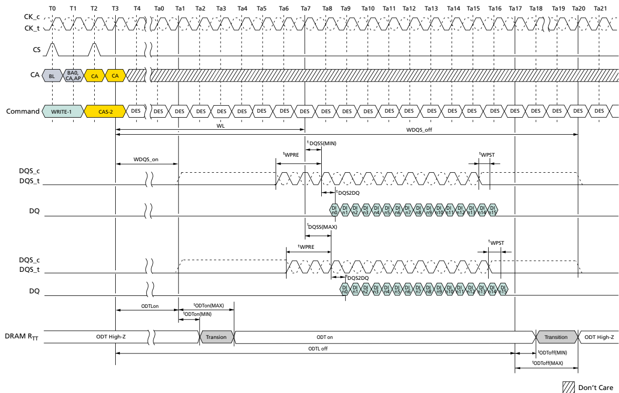
Figure 42: Burst WRITE Operation
