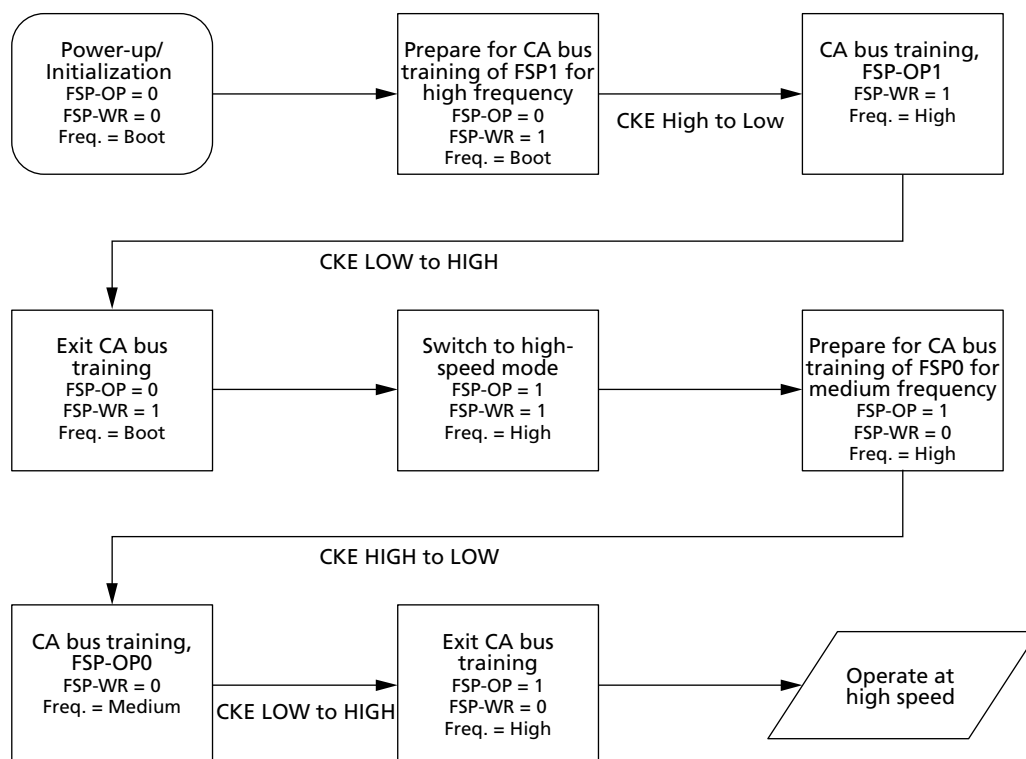
Figure 143: Training for Two Frequency Set Points
