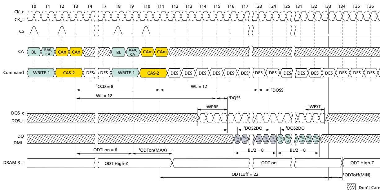
Figure 59: Seamless WRITE: t_{CCD} = \text{MIN} , 1.5nCK Postamble, 533 \text{ MHz} < \text{Clock Frequency} \leq 800 \text{ MHz} , ODT Worst Timing Case
