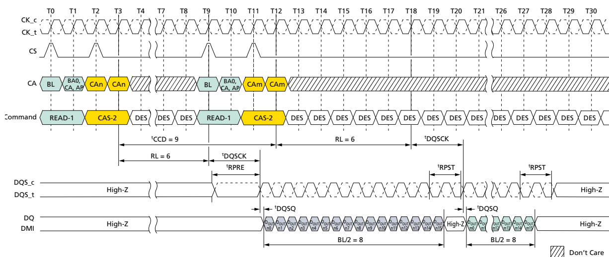
Figure 48: Consecutive READ: t_{CCD} = \text{MIN} + 1 , Preamble = Static, 1.5n\text{CK} Postamble
