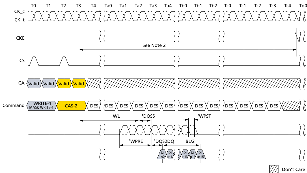
Figure 90: Write With Auto Precharge and Mask Write With Auto Precharge to Power-Down Entry
