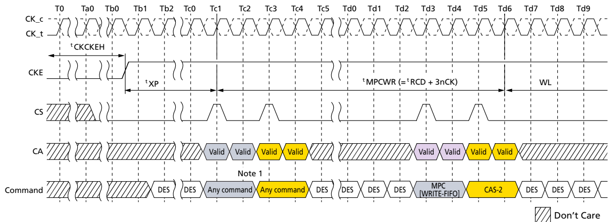
Figure 136: Power-Down Exit to MPC[WRITE-FIFO] Timing
