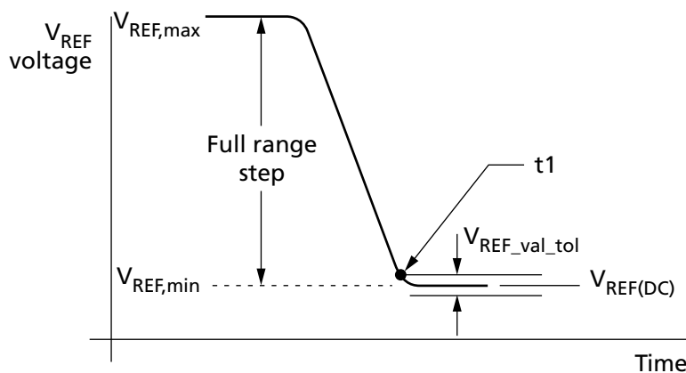
Figure 110: V_{REF(CA)} Full Step from V_{REF,max} to V_{REF,min}
