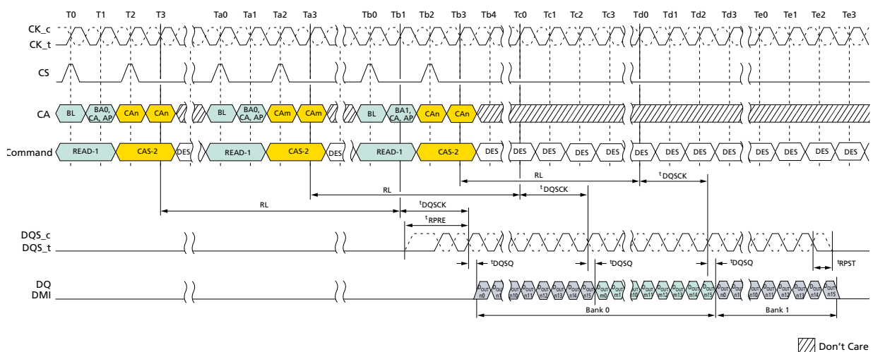
Figure 26: Seamless Burst Read
