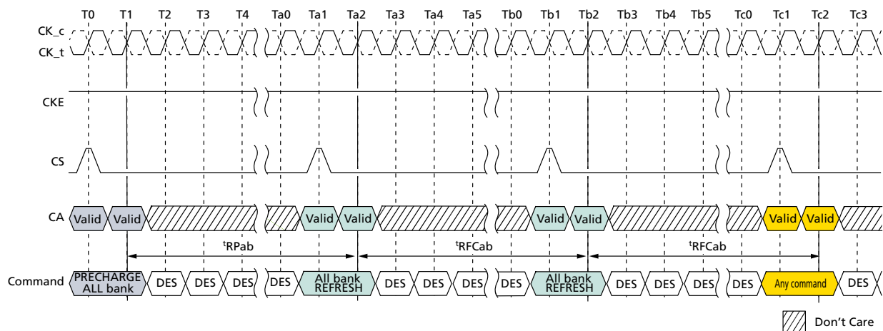
Figure 76: All-Bank REFRESH Operation
