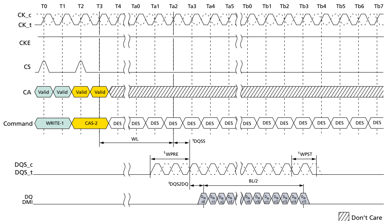
Figure 23: DQS Write Preamble and Postamble – 1.5nCK Postamble
