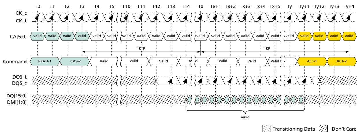
Figure 72: Burst READ With Auto Precharge – BL32, Toggling Preamble, 1.5nCK Postamble
