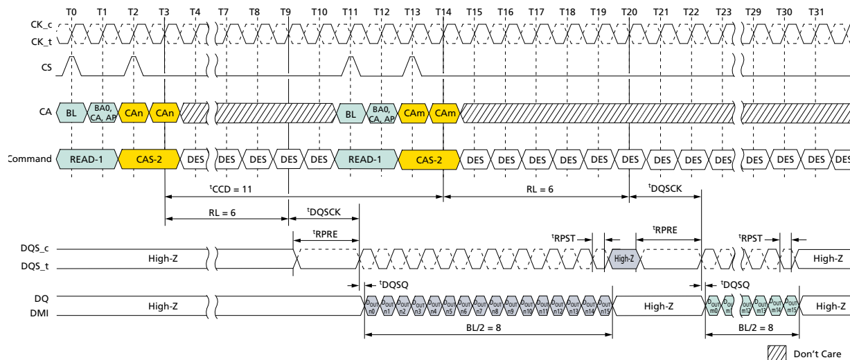
Figure 57: Consecutive READ: t_{CCD} = \text{MIN} + 3 , Preamble = Static, 0.5n\text{CK} Postamble
