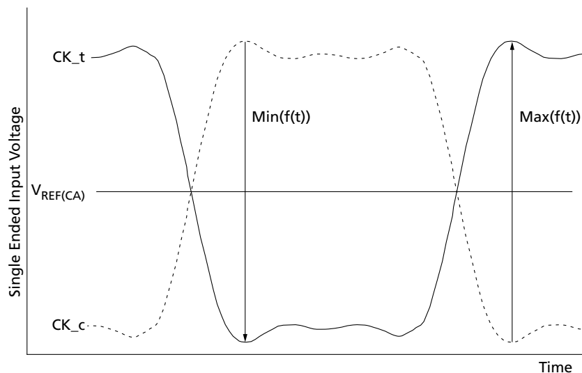
Figure 156: Definition of Differential Clock Peak Voltage
