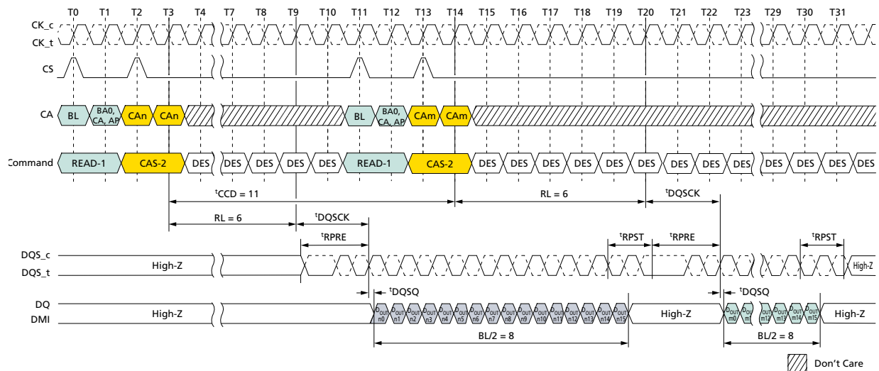
Figure 54: Consecutive READ: t_{CCD} = \text{MIN} + 3 , Preamble = Toggle, 1.5n\text{CK} Postamble
