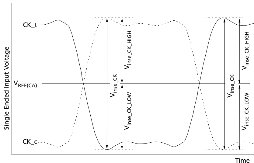
Figure 157: Clock Single-Ended Input Voltage
