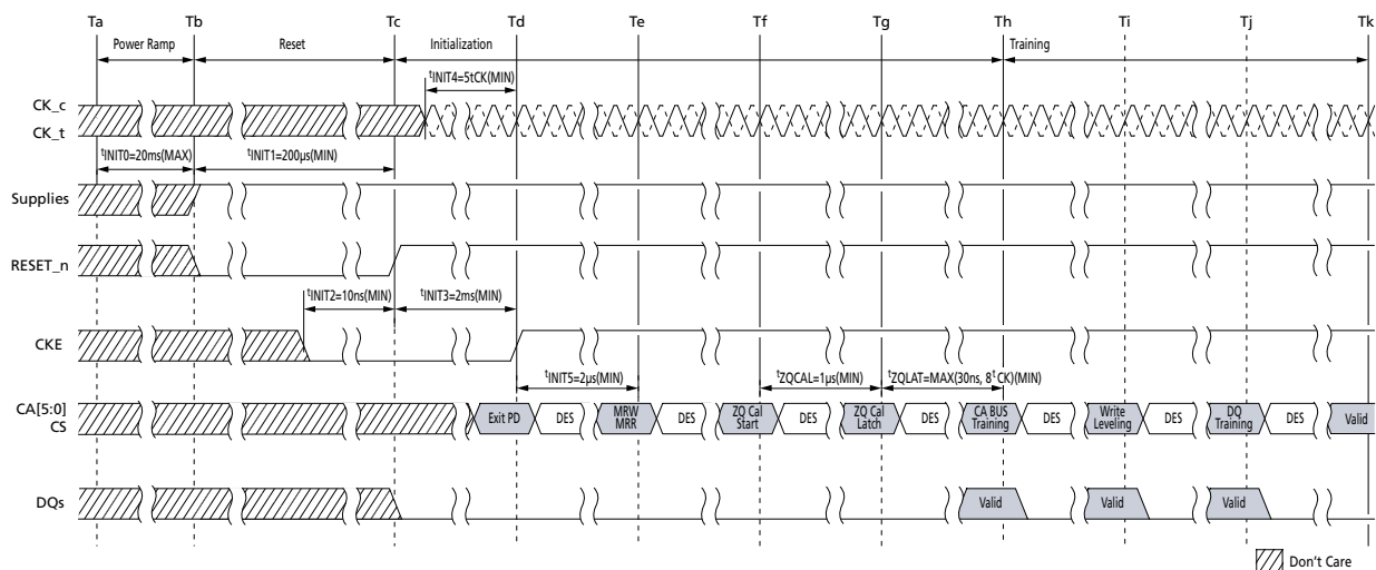
Figure 17: Voltage Ramp and Initialization Sequence
