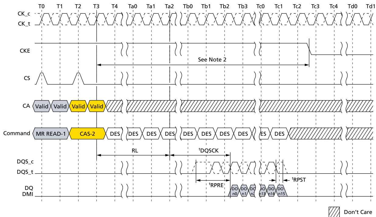
Figure 94: Mode Register Read to Power-Down Entry
