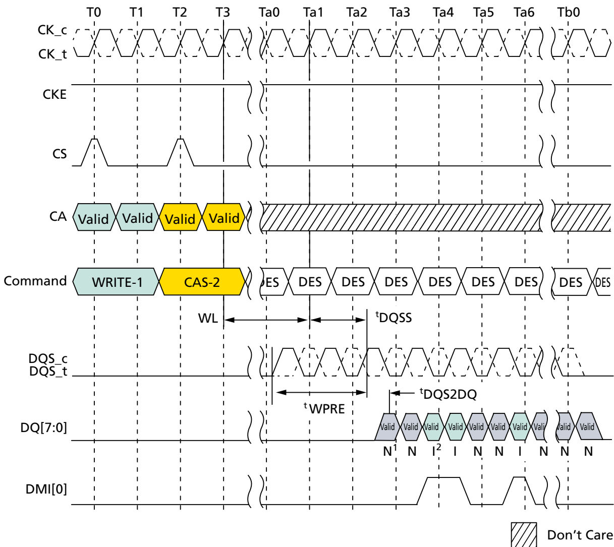
Figure 40: WRITE Command with Write DBI Enabled; DM Disabled
