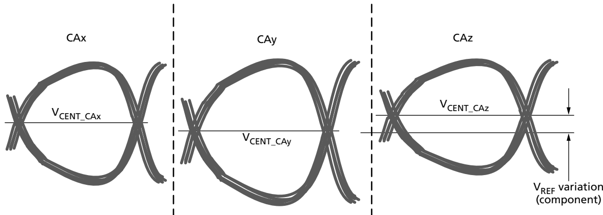
Figure 174: Across Pin V_{REF} (CA) Voltage Variation
