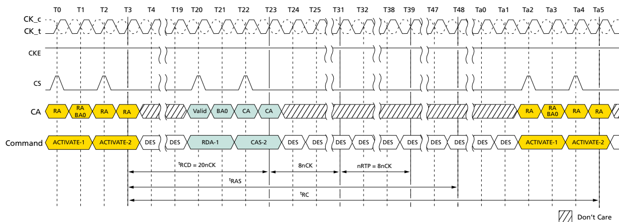
Figure 74: Command Input Timing with RAS Lock
