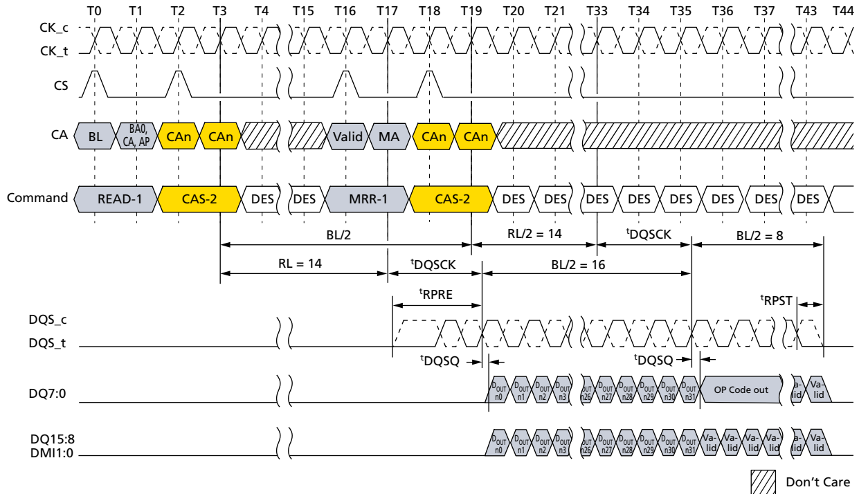
Figure 98: READ-to-MRR Timing
