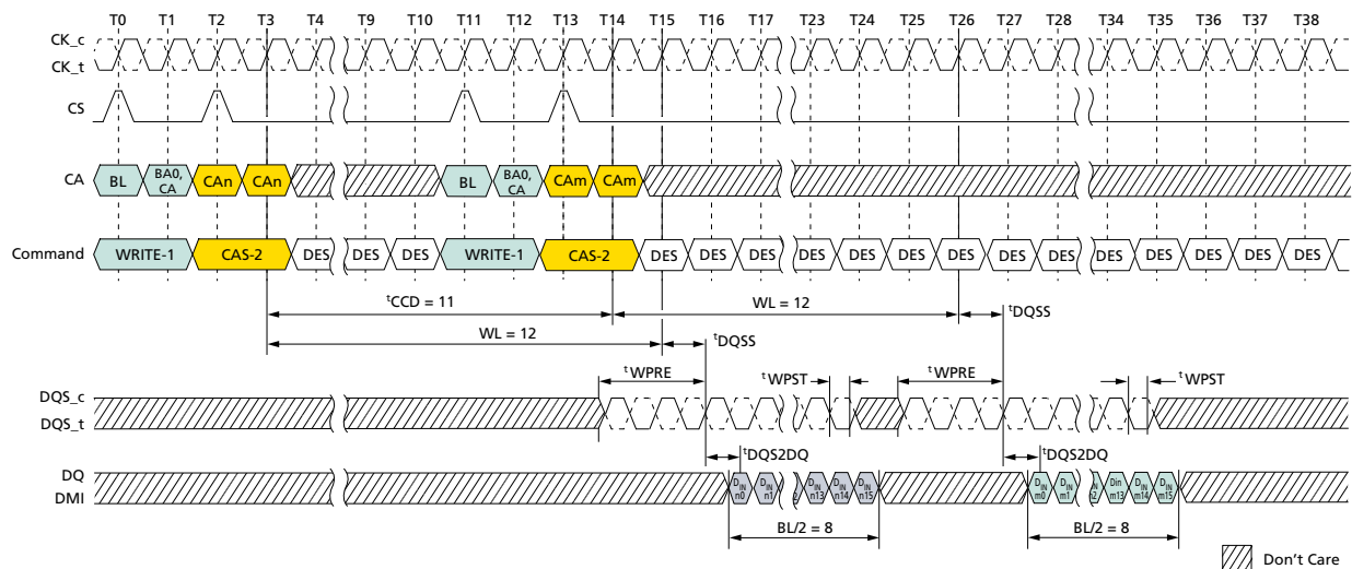
Figure 65: Consecutive WRITE: t_{CCD} = \text{MIN} + 3, 0.5n\text{CK} Postamble
