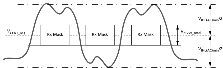
Figure 189: DQ V_{IHL(AC)} Definition (for Each Input Pulse)
