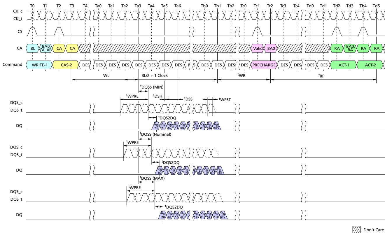
Figure 38: Burst WRITE Operation
