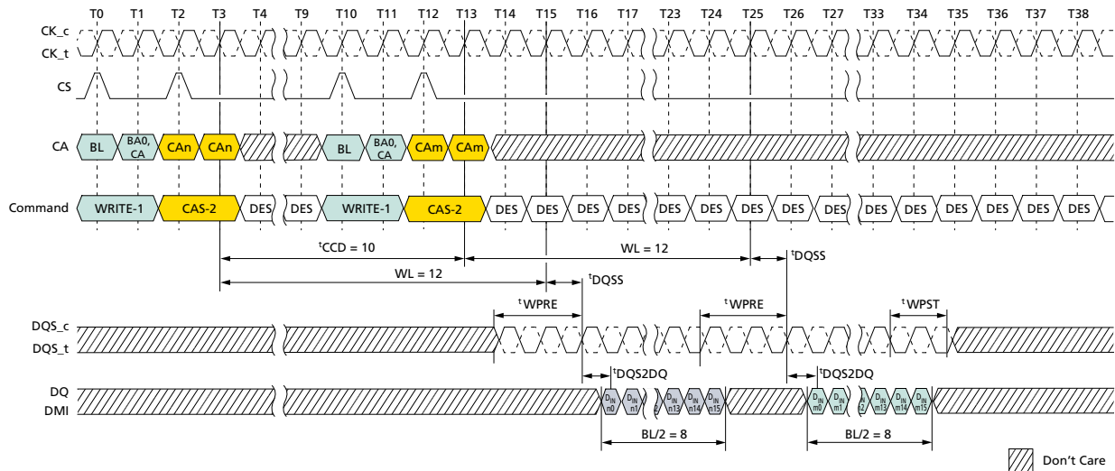
Figure 70: Consecutive WRITE: t_{CCD} = \text{MIN} + 2, 1.5n\text{CK} Postamble
