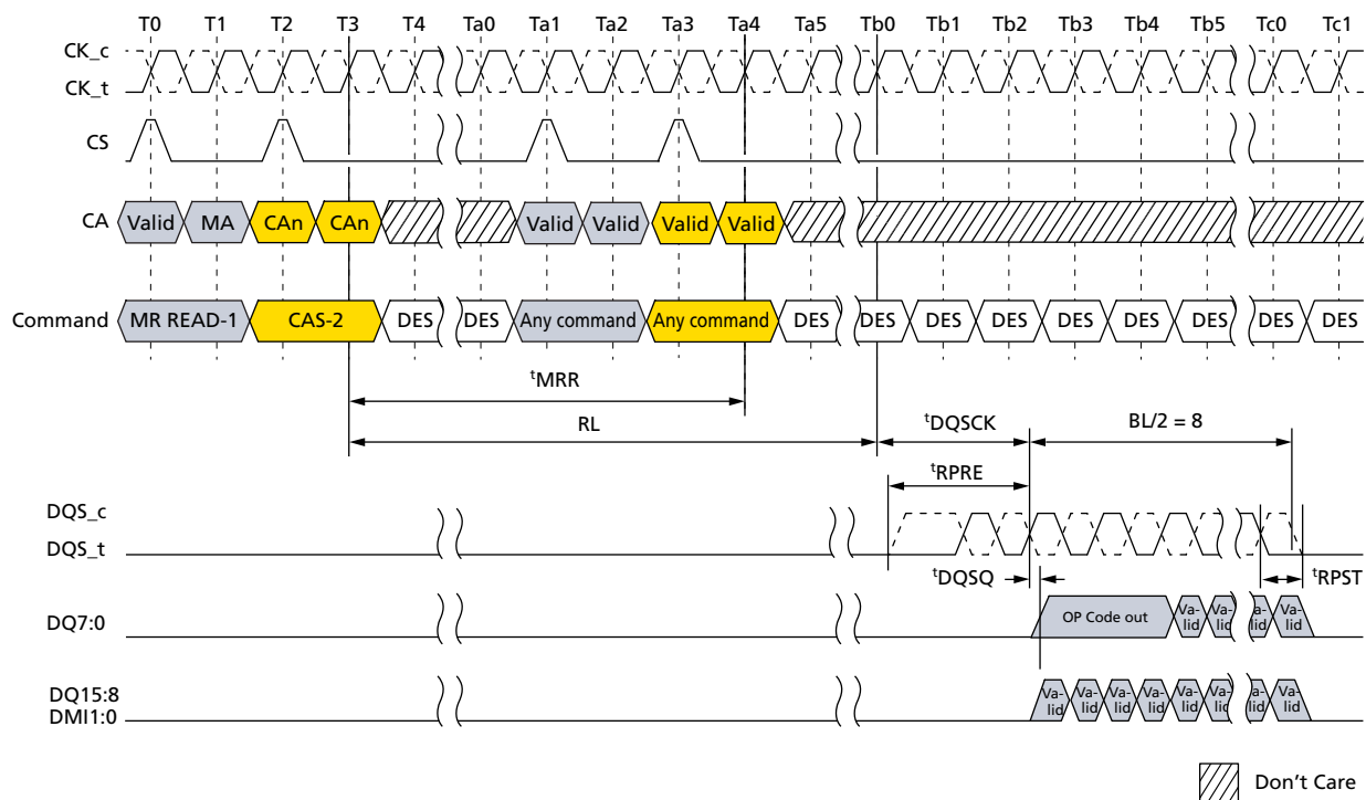
Figure 103: MODE REGISTER READ Operation
