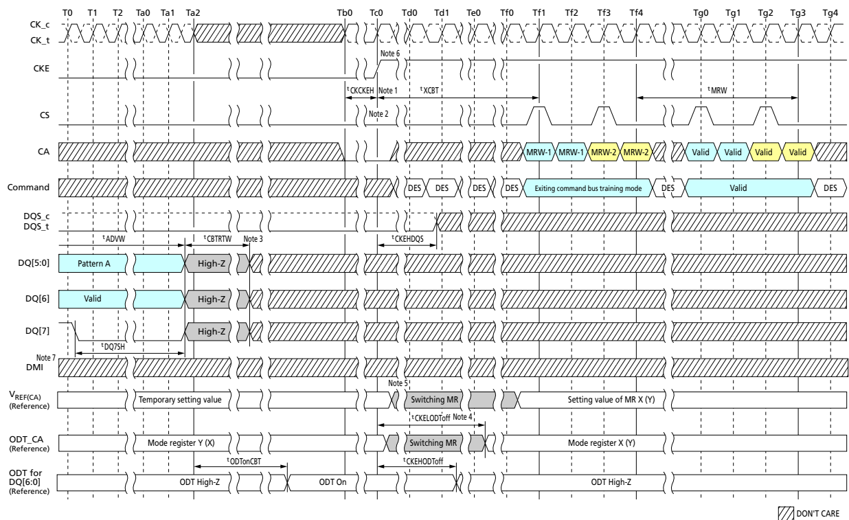
Figure 206: Exiting Command Bus Training Mode
