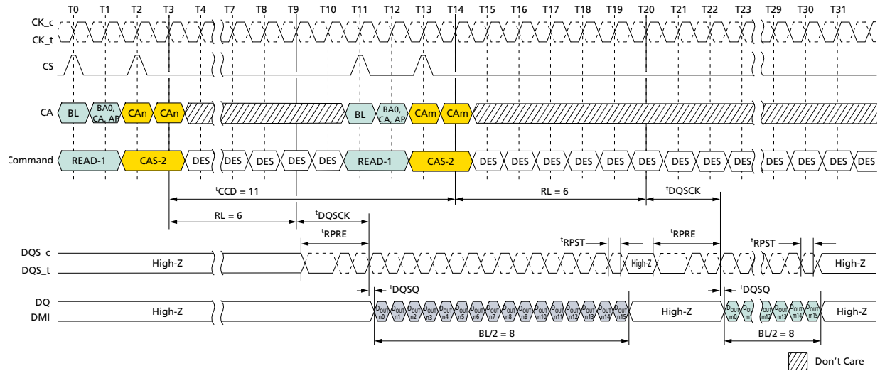
Figure 61: Consecutive READ: t_{CCD} = \text{MIN} + 3 , Preamble = Toggle, 0.5n\text{CK} Postamble
