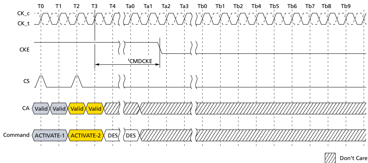
Figure 98: ACTIVATE Command to Power-Down Entry
