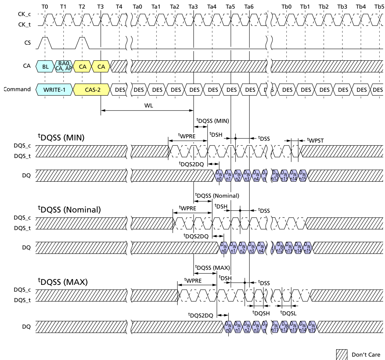
Figure 40: Write Timing
