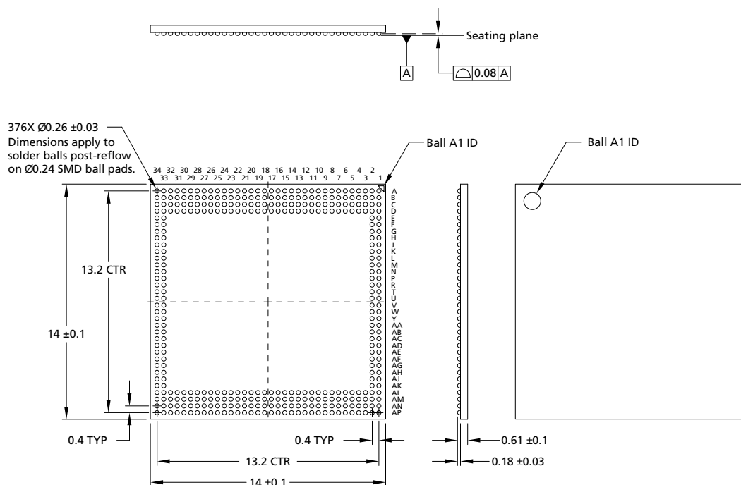
Figure 18: 376-Ball WFBGA – 14.0mm x 14.0mm x 0.71mm (Package Code: NZ)
