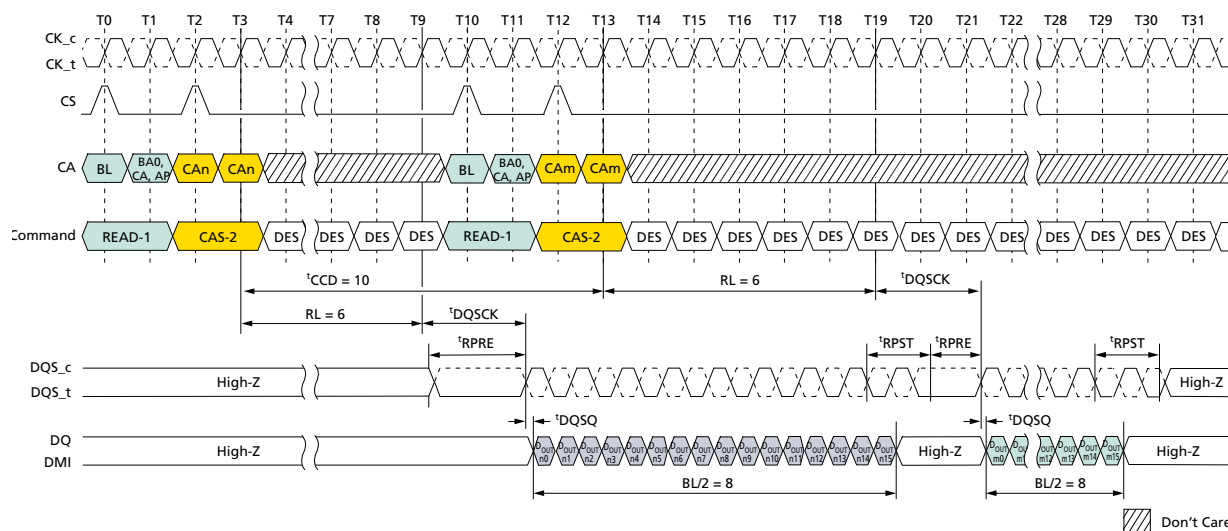
Figure 58: Consecutive READ: t_{CCD} = \text{MIN} + 2 , Preamble = Static, 1.5n\text{CK} Postamble
