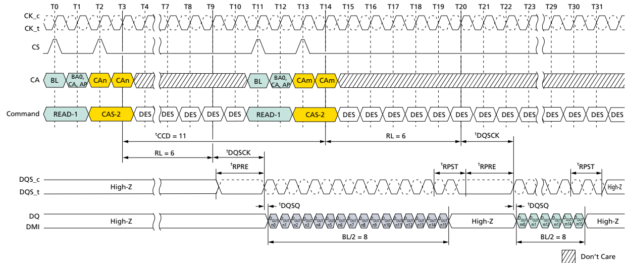
Figure 62: Consecutive READ: t_{CCD} = \text{MIN} + 3 , Preamble = Static, 1.5n\text{CK} Postamble
