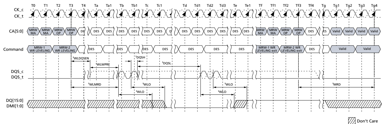
Figure 128: Write Leveling Timing – t_{DQSL(MAX)}
