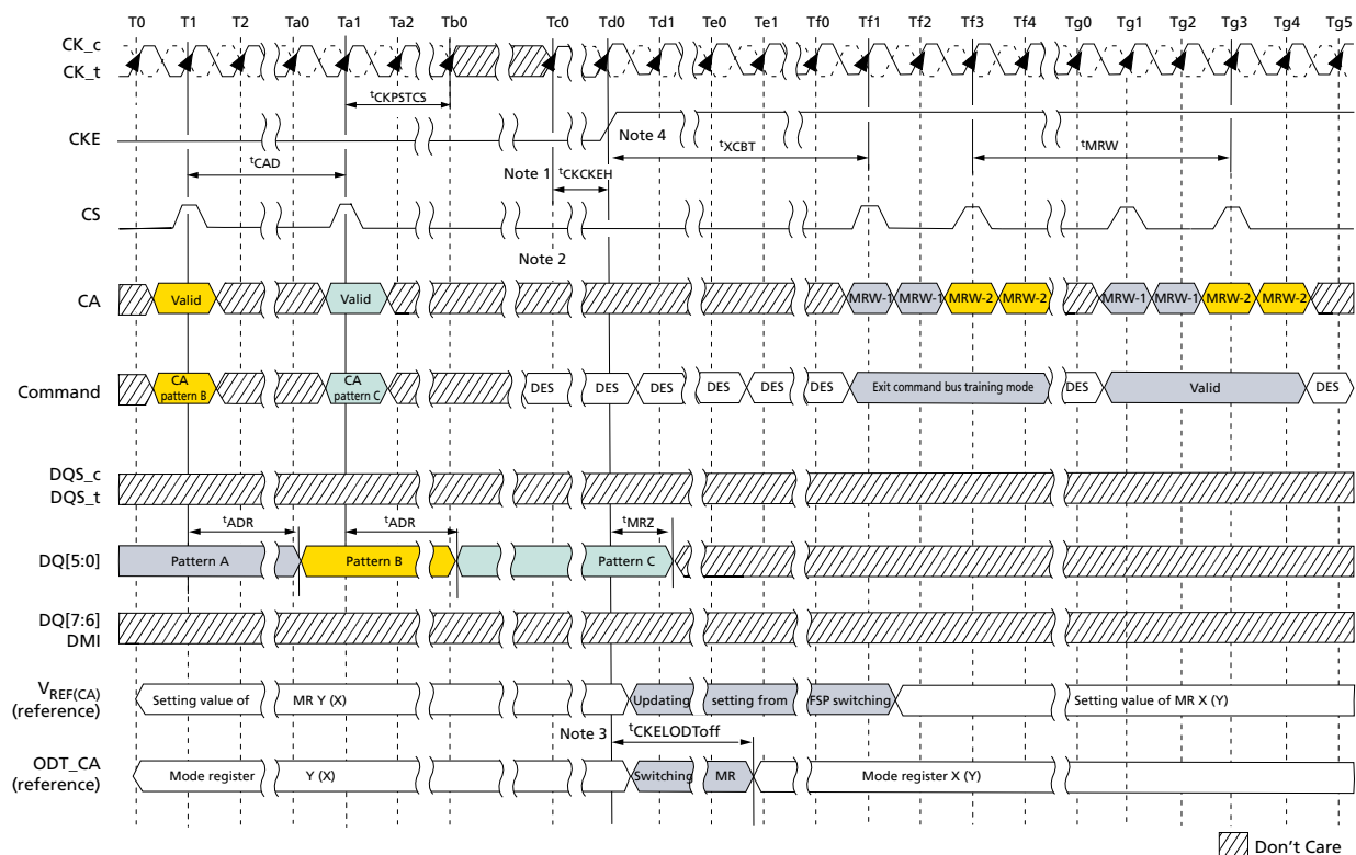
Figure 201: Exiting CBT Mode with Valid Command
