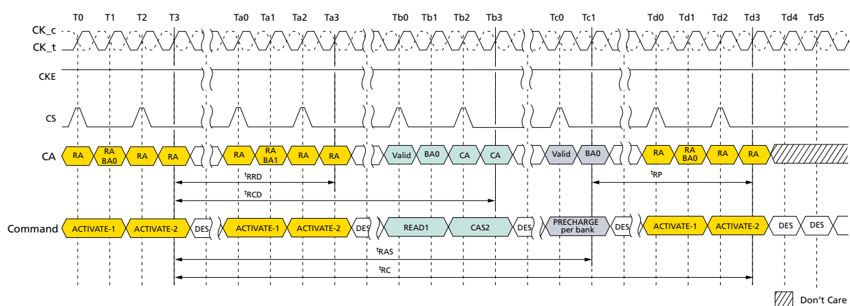
Figure 24: ACTIVATE Command
