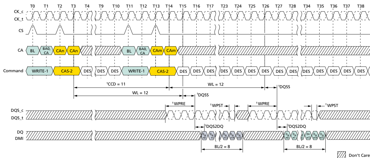
Figure 71: Consecutive WRITE: t_{CCD} = \text{MIN} + 3, 0.5nCK Postamble
