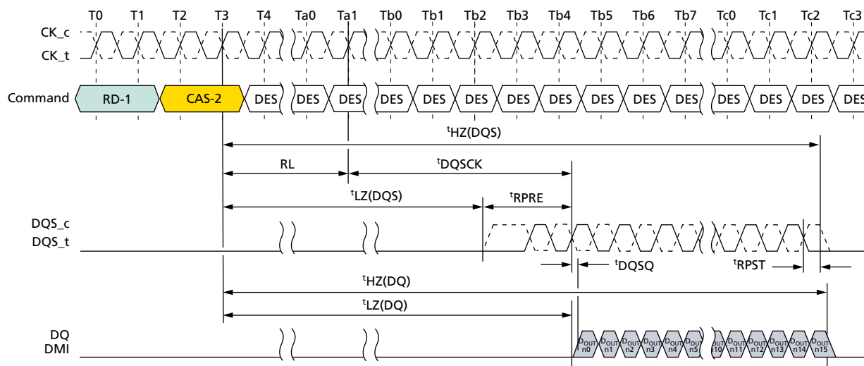
Figure 33: Read Timing
