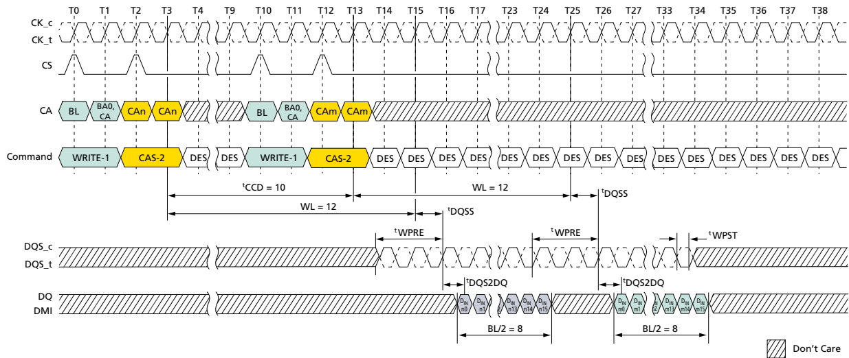
Figure 69: Consecutive WRITE: t_{CCD} = \text{MIN} + 2, 0.5n\text{CK} Postamble
