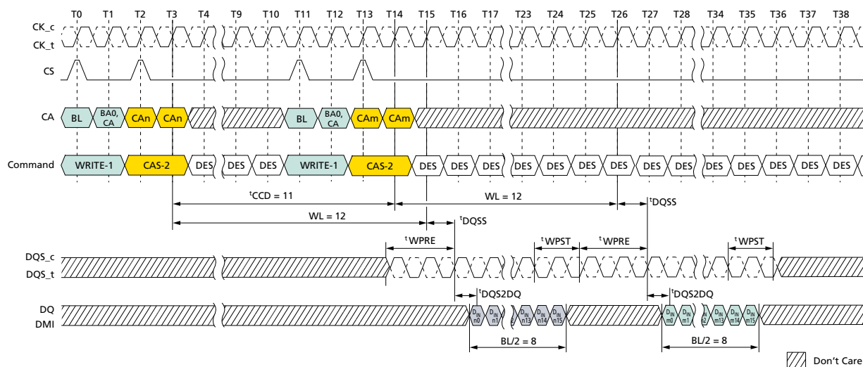
Figure 72: Consecutive WRITE: t_{CCD} = \text{MIN} + 3, 1.5nCK Postamble
