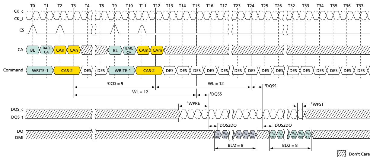
Figure 67: Consecutive WRITE: t_{CCD} = \text{MIN} + 1, 0.5nCK Postamble
