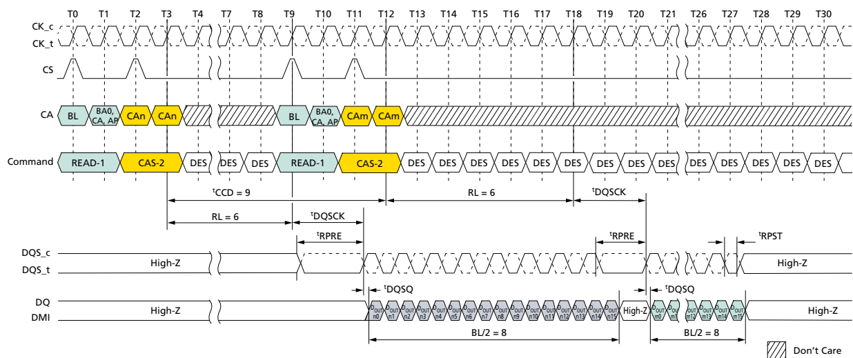
Figure 55: Consecutive READ: t_{CCD} = MIN + 1 , Preamble = Static, 0.5nCK Postamble
