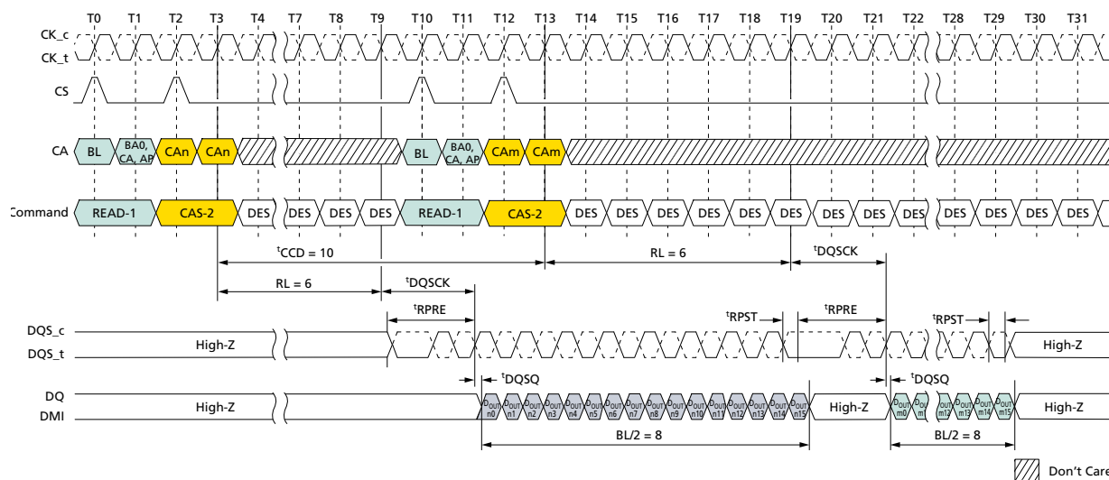
Figure 57: Consecutive READ: t_{CCD} = \text{MIN} + 2 , Preamble = Toggle, 0.5n\text{CK} Postamble
