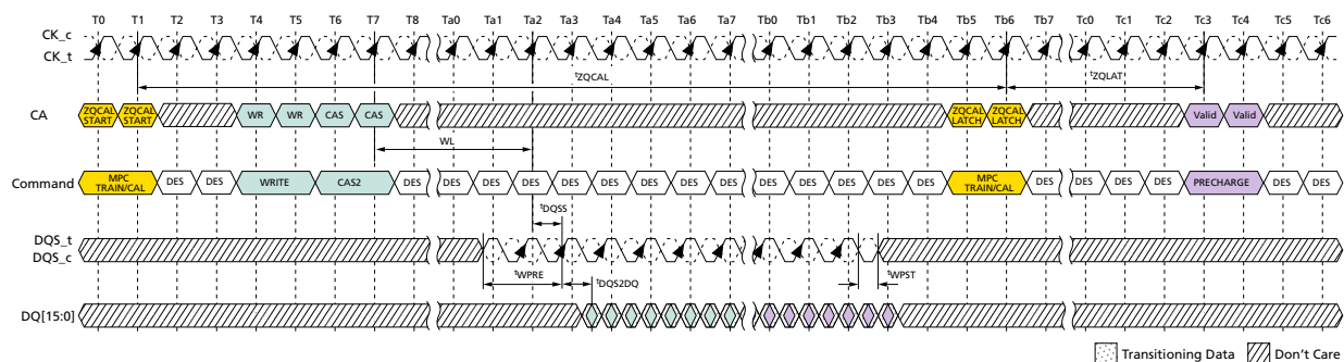
Figure 147: ZQCAL Timing
