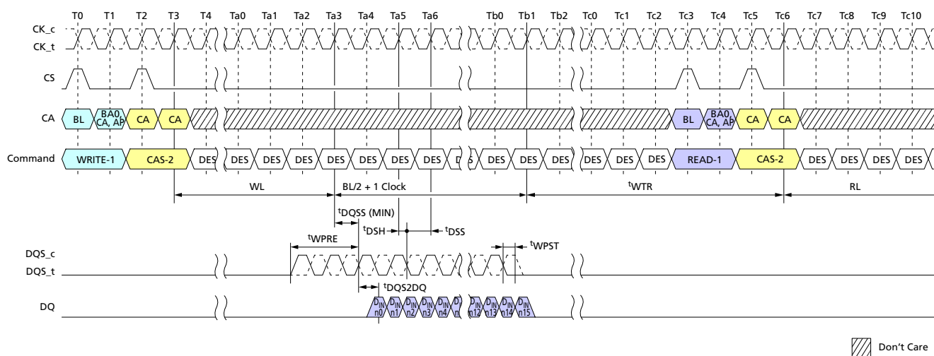
Figure 39: Burst Write Followed by Burst Read
