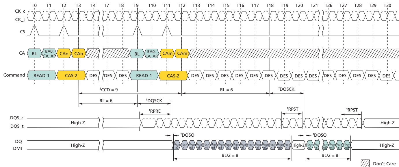
Figure 39: Seamless READ: t_{CCD} = \text{MIN} + 1 , Preamble = Toggle, 1.5nCK Postamble
