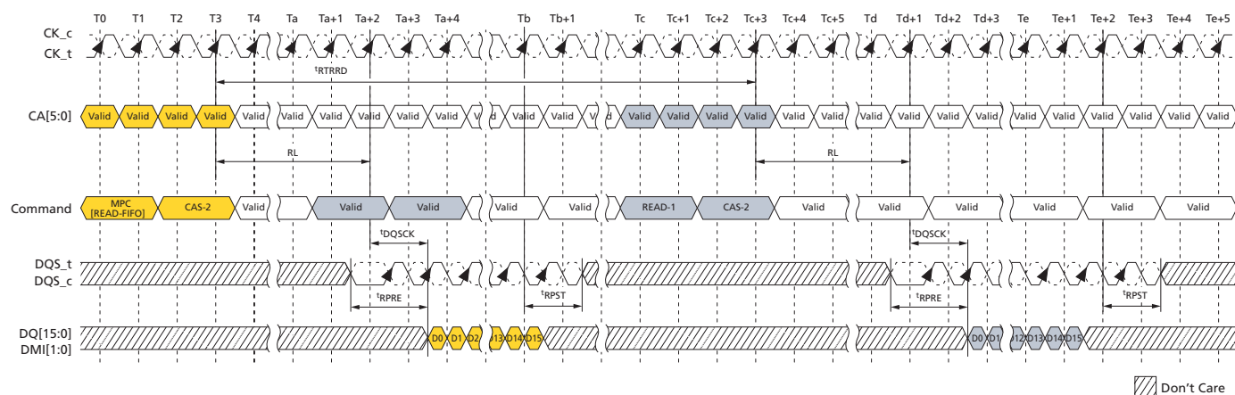
Figure 121: READ-FIFO – t_{\text{RPRE}} = \text{Toggle} , t_{\text{RPST}} = 1.5n\text{CK}
