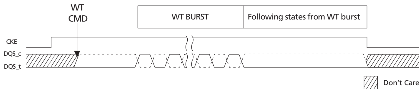
Figure 34: WDQS Control Mode 1
