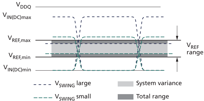
Figure 104: V_{REF} Operating Range ( V_{REF,max} , V_{REF,min} )
