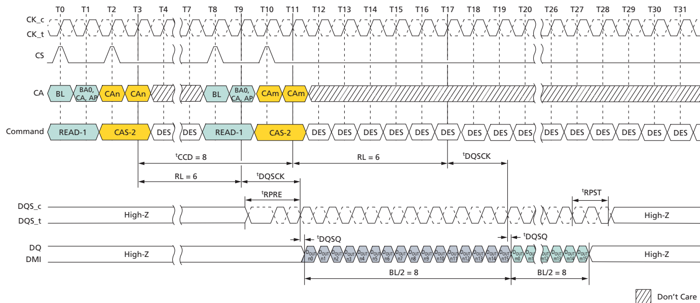
Figure 38: READ Operations: t_{CCD} = \text{MIN} , Preamble = Toggle, 1.5nCK Postamble
