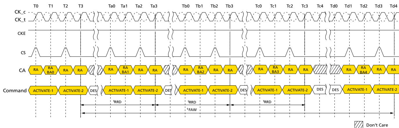
Figure 17: t_{FAW} Timing
