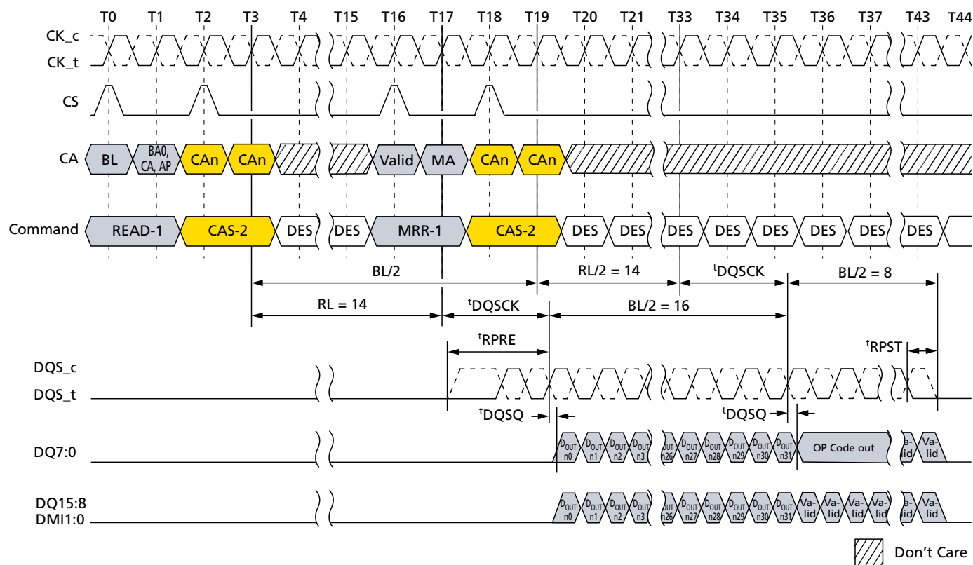
Figure 96: READ-to-MRR Timing
