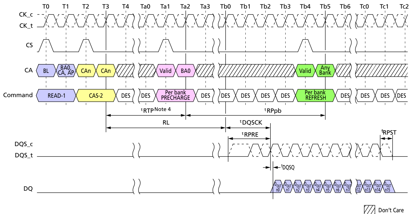
Figure 78: Burst READ Operation Followed by Per-Bank Refresh
