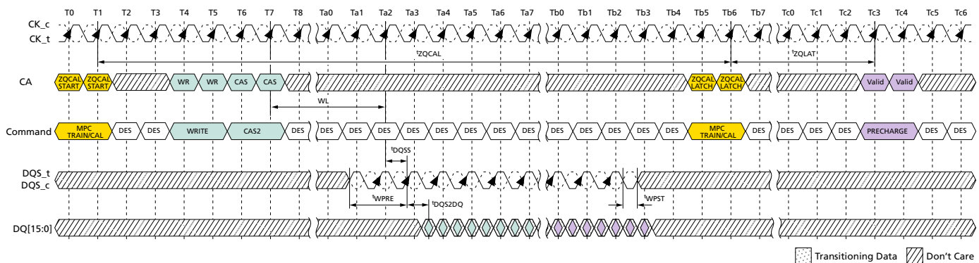
Figure 134: ZQCAL Timing
