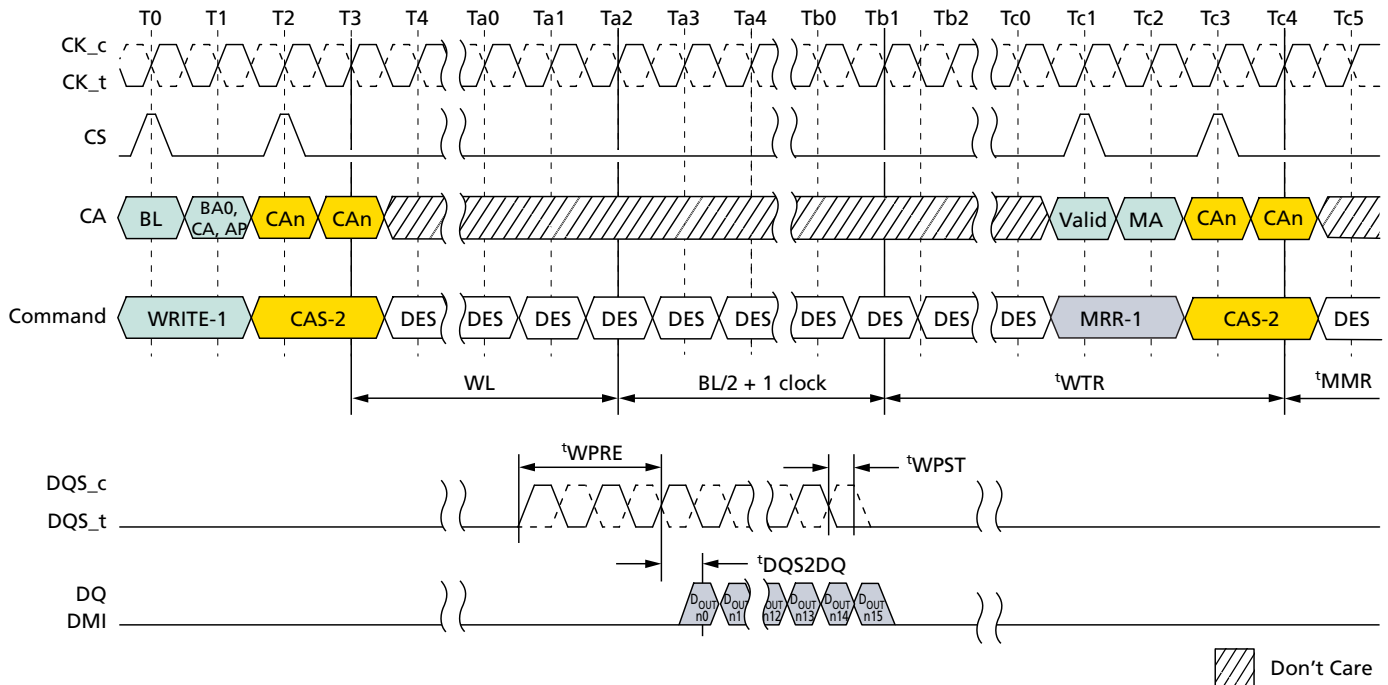
Figure 92: WRITE-to-MRR Timing
