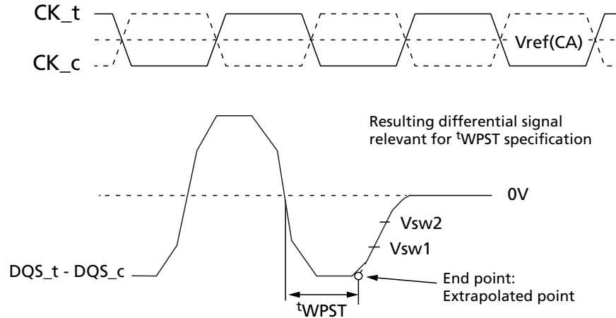
Figure 29: Method for Calculating t_{WPST} Transitions and Endpoints
