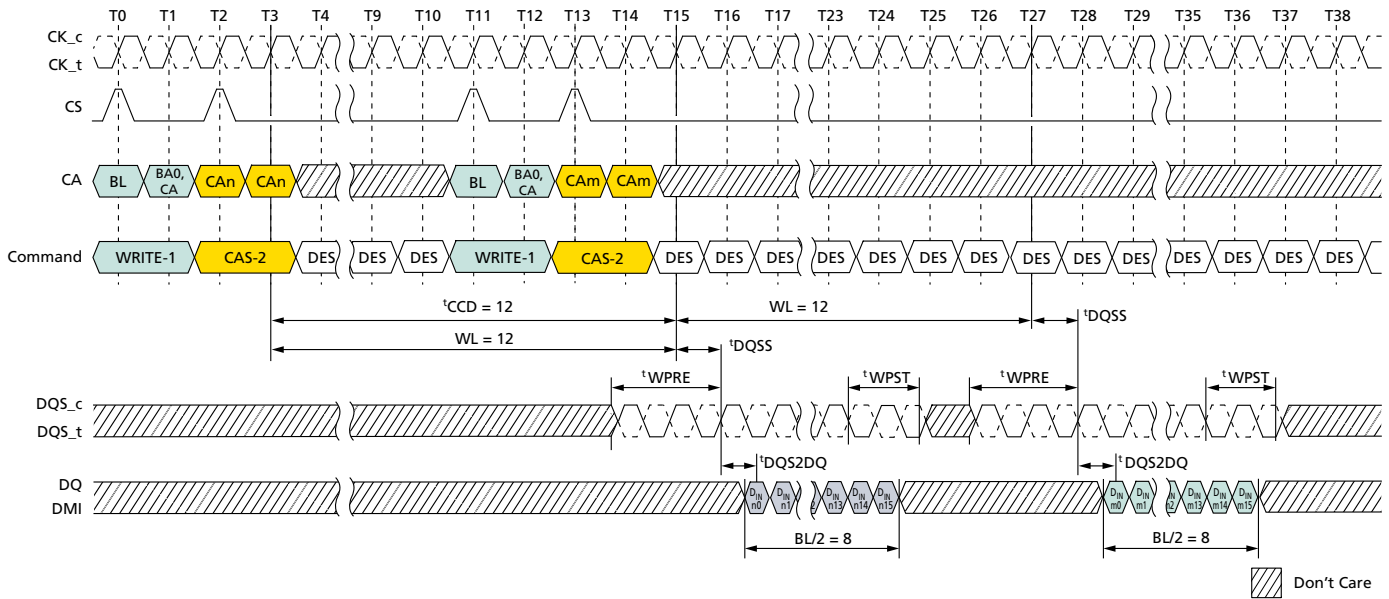
Figure 60: Consecutive WRITE: t_{CCD} = \text{MIN} + 4, 1.5nCK Postamble
