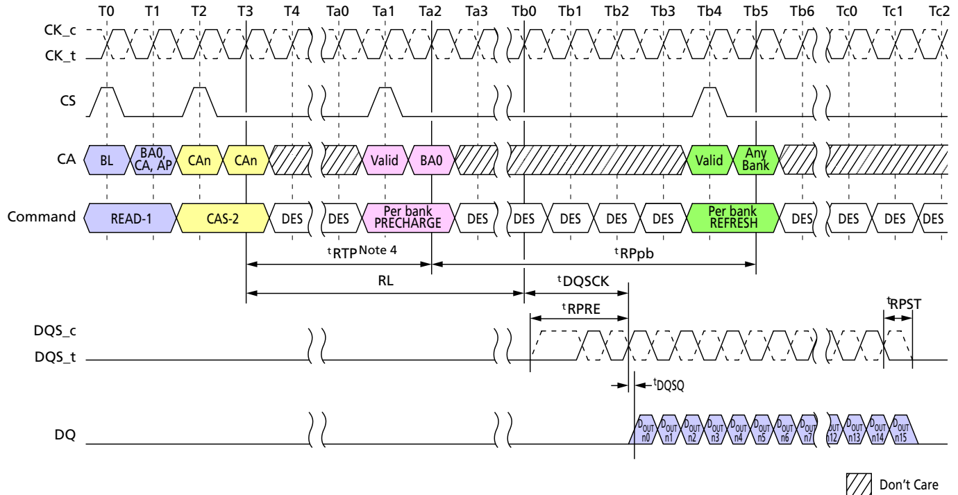
Figure 73: Burst READ Operation Followed by Per-Bank Refresh
