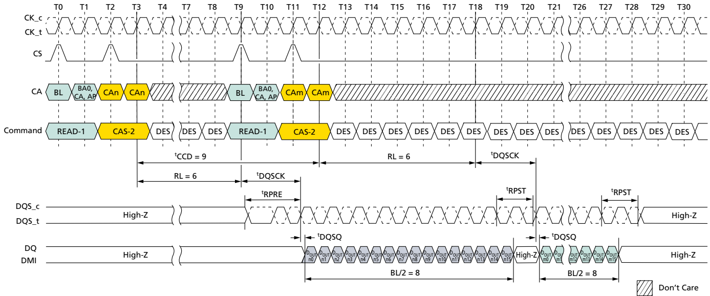
Figure 39: Seamless READ: t_{CCD} = \text{MIN} + 1 , Preamble = Toggle, 1.5n\text{CK} Postamble
