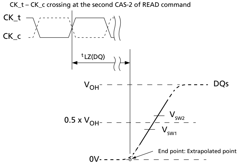
Figure 23: t_{LZ}(DQ) Method for Calculating Transitions and Endpoint
