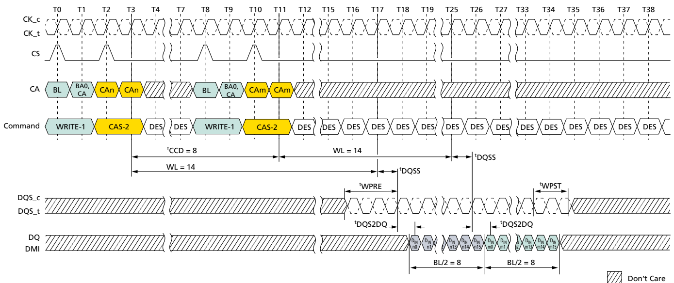
Figure 53: Seamless WRITE: t_{CCD} = \text{MIN} , 1.5nCK Postamble
