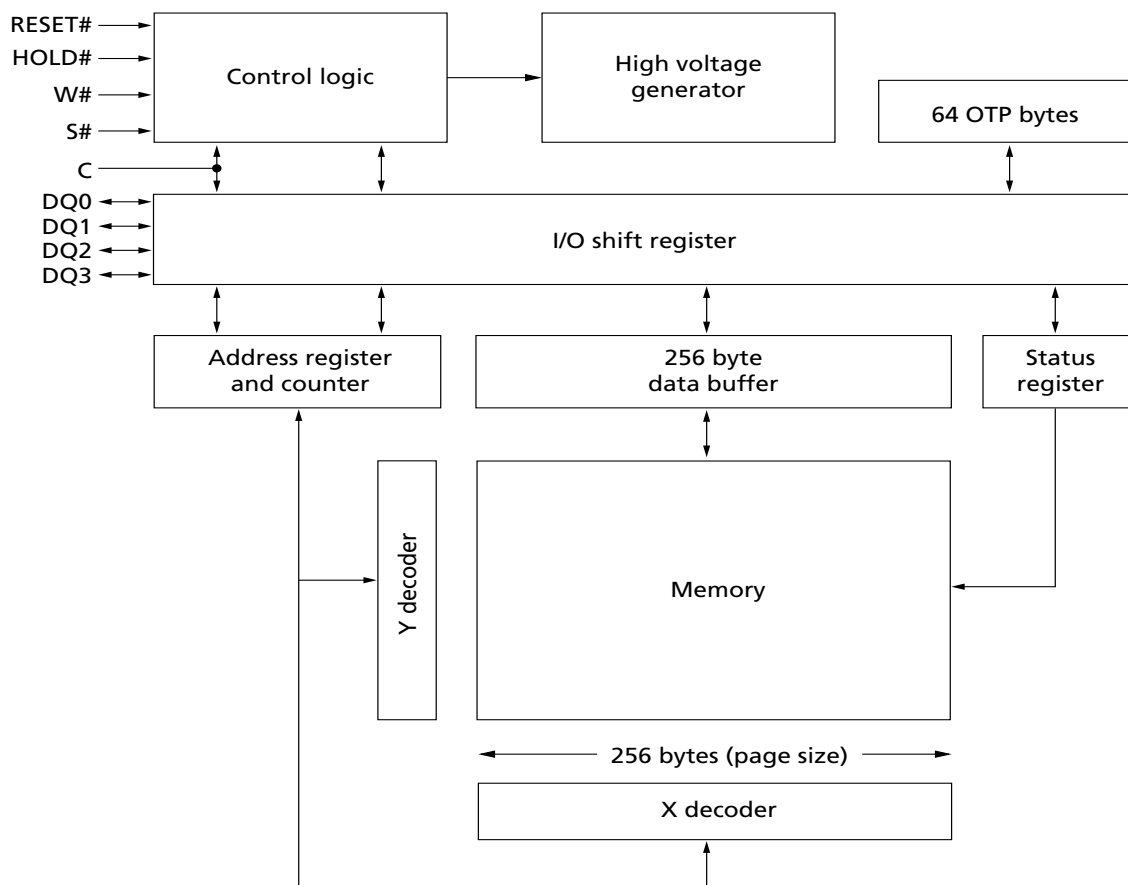
Figure 2: Block Diagram
