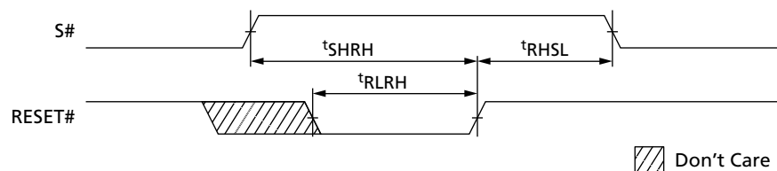
Figure 46: Reset Enable and Reset Memory Timing
