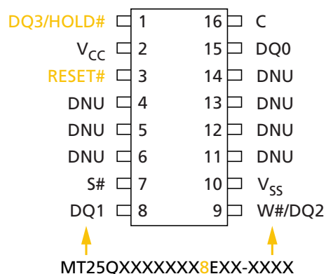
Figure 5: 16-Pin, Plastic Small Outline – SO16 (Top View)
