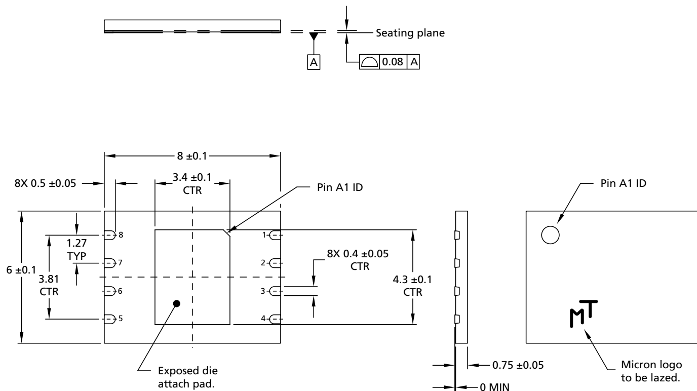
Figure 9: W-PDFN-8 (MLP8) – 8mm x 6mm
