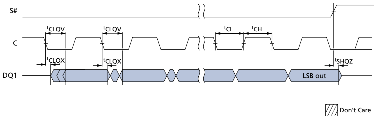
Figure 51: Output Timing for STR
