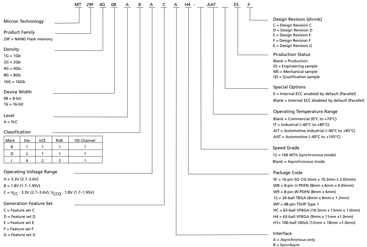
Figure 1: Part Numbering
