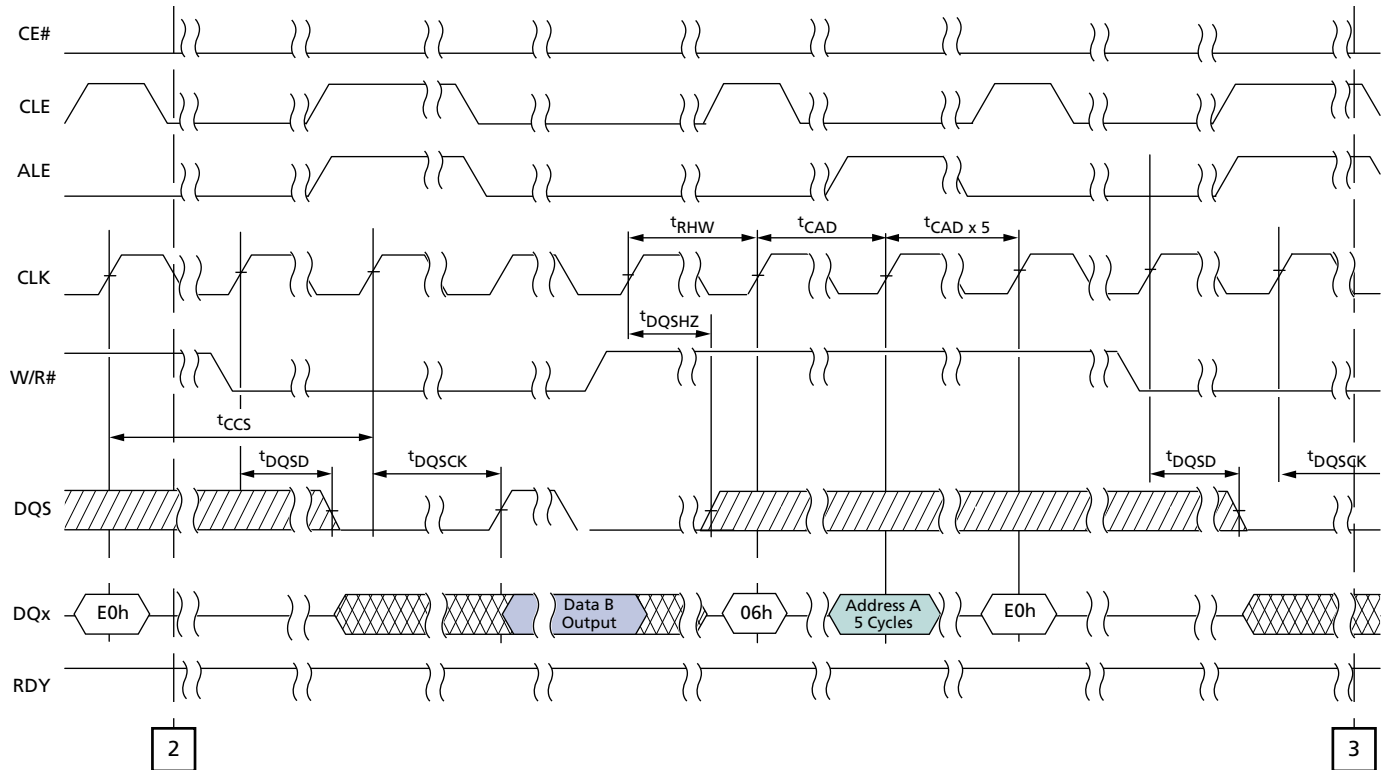
Figure 95: Multi-Plane Read Page (2 of 2)
