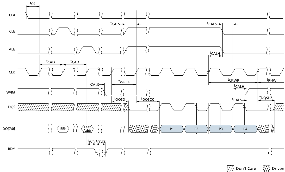
Figure 83: GET FEATURES Operation
