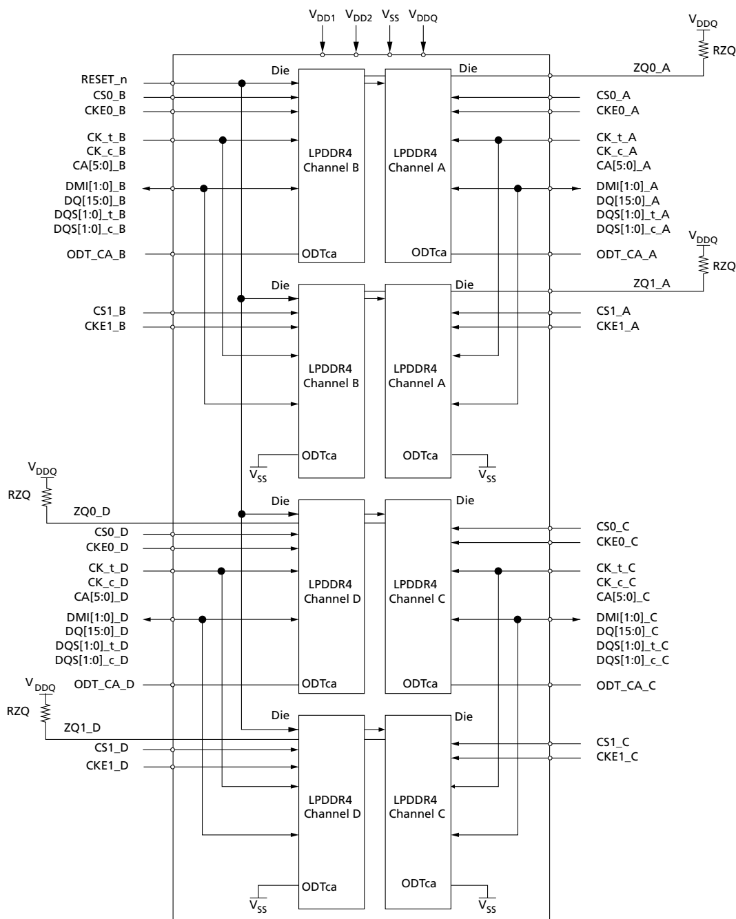
Figure 3: Eight-Die, Quad-Channel Package Block Diagram
