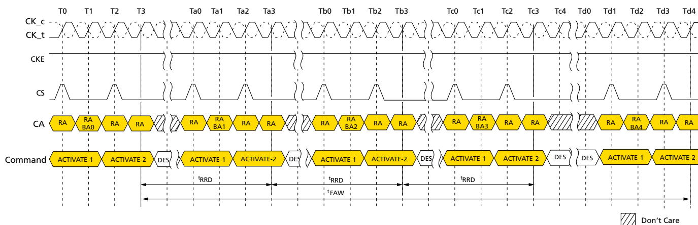
Figure 12: t_{FAW} Timing
