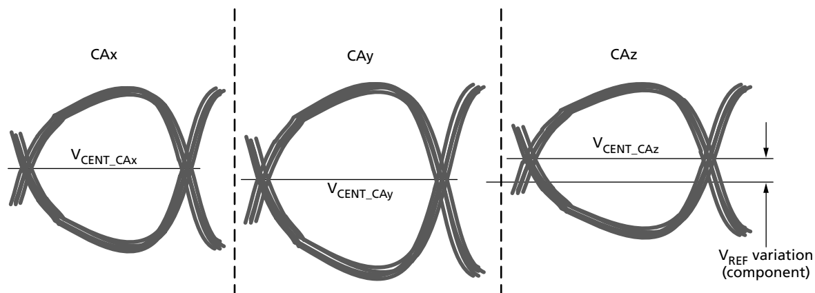
Figure 167: Across Pin V_{REF} (CA) Voltage Variation
