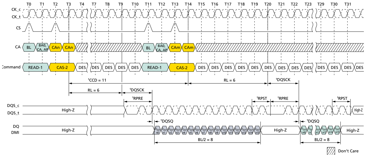
Figure 45: Consecutive READ: t_{CCD} = \text{MIN} + 3 , Preamble = Toggle, 1.5n\text{CK} Postamble
