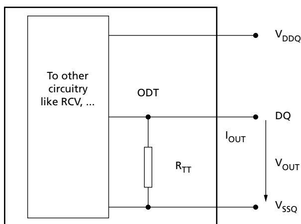
Figure 139: Functional Representation of DQ ODT
