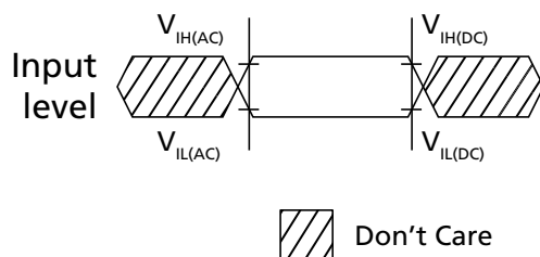
Figure 144: Input Timing Definition for CKE
