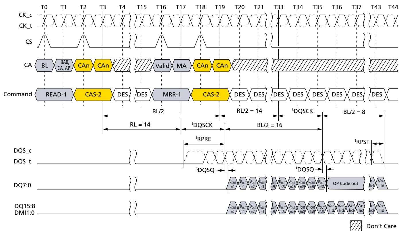
Figure 89: READ-to-MRR Timing
