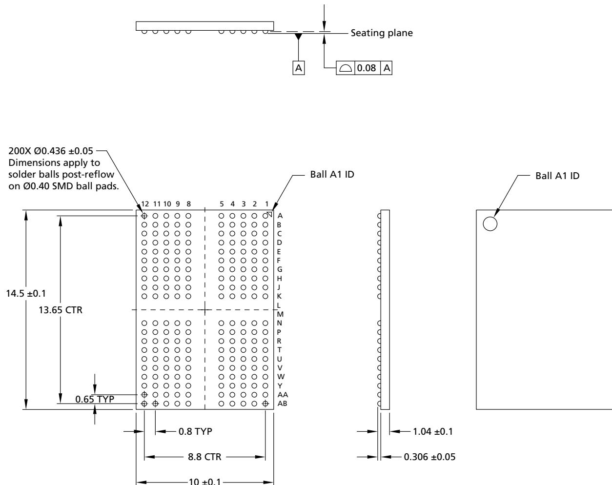
Figure 4: 200-Ball TFBGA – 10mm x 14.5mm x 1.14mm (Package Code: DE)
