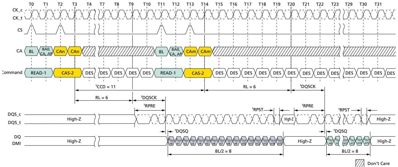
Figure 46: Consecutive READ: t_{CCD} = \text{MIN} + 3 , Preamble = Toggle, 0.5n\text{CK} Postamble
