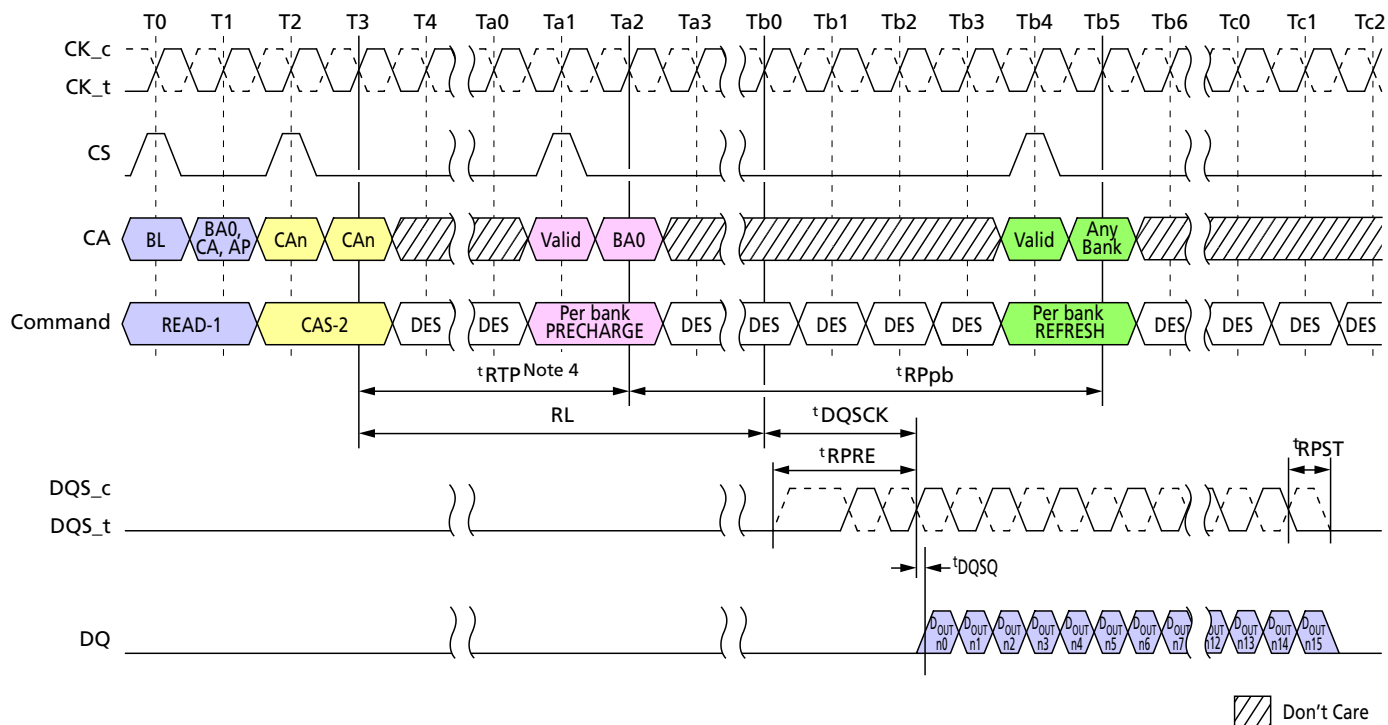
Figure 71: Burst READ Operation Followed by Per-Bank Refresh
