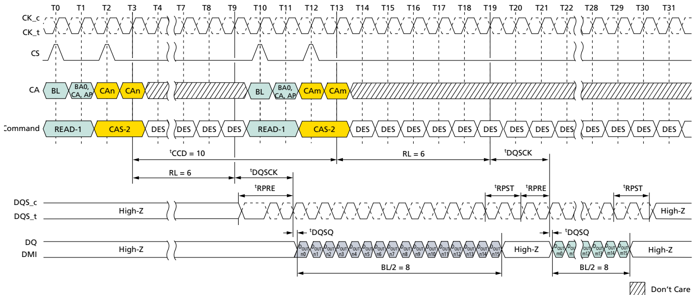
Figure 41: Consecutive READ: t_{CCD} = \text{MIN} + 2 , Preamble = Toggle, 1.5n\text{CK} Postamble
