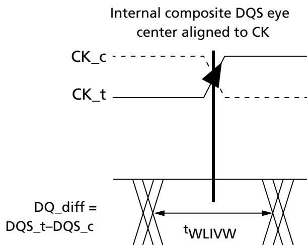
Figure 118: DQS_t/DQS_c to CK_t/CK_c Timings at the Pins Referenced from the Internal Latch
