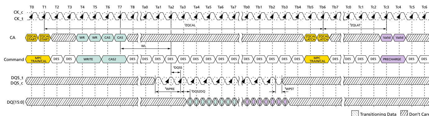
Figure 134: ZQCAL Timing
