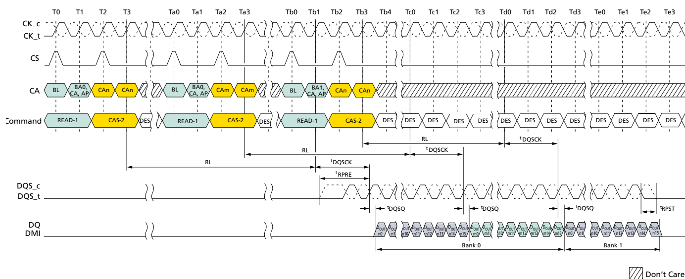
Figure 19: Seamless Burst Read
