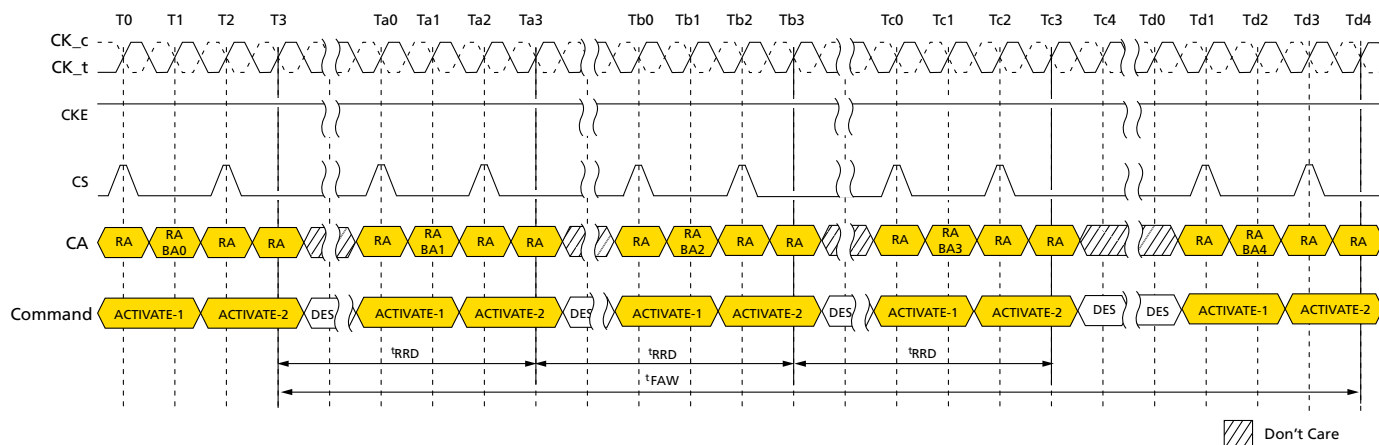
Figure 12: t_{FAW} Timing
