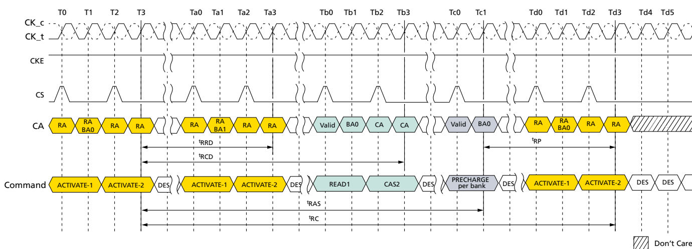
Figure 11: ACTIVATE Command
