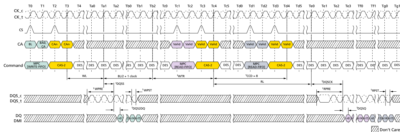
Figure 126: MPC[WRITE-FIFO]-to-MPC[READ-FIFO] Timing
