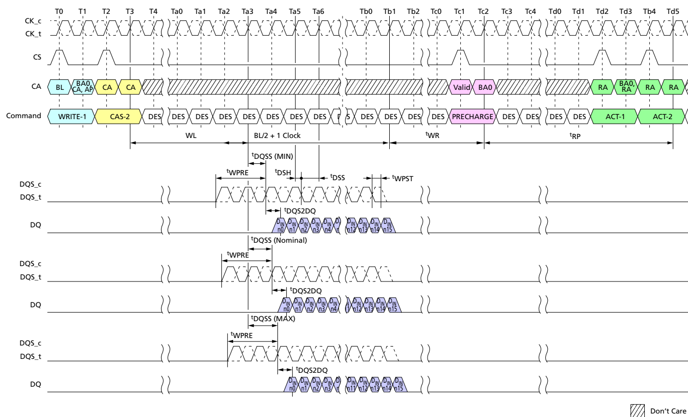
Figure 25: Burst WRITE Operation
