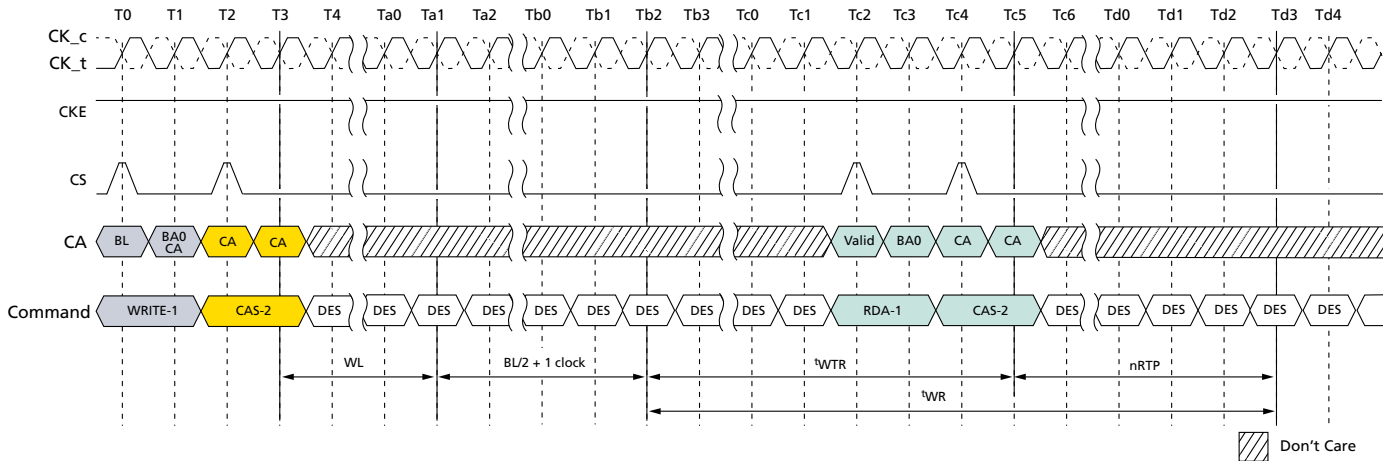
Figure 65: Delay Time From WRITE-to-READ with Auto Precharge
