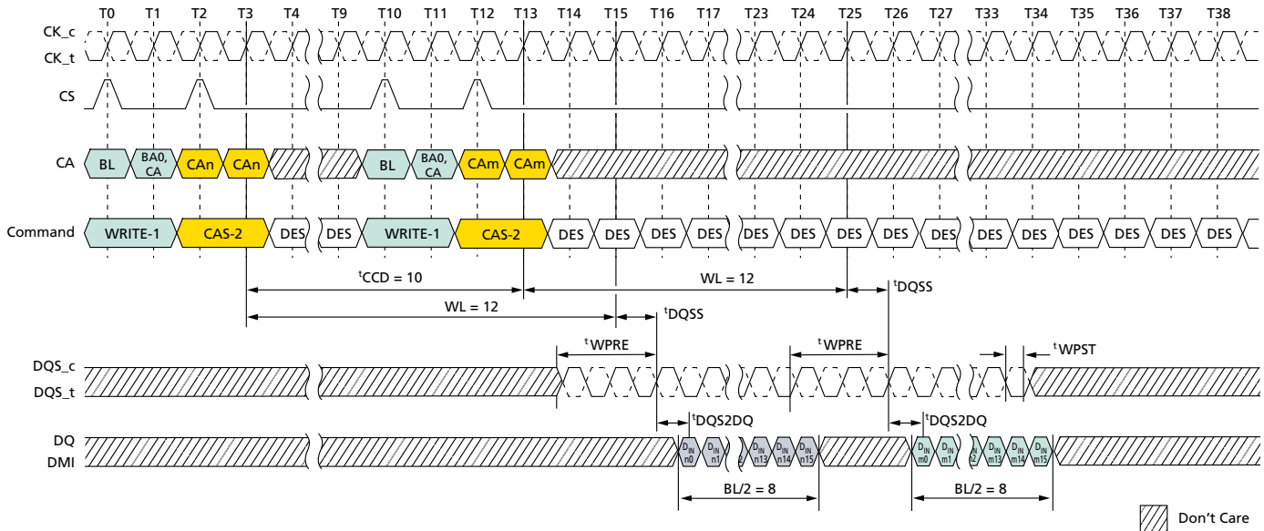
Figure 53: Consecutive WRITE: t_{CCD} = MIN + 2, 0.5nCK Postamble
