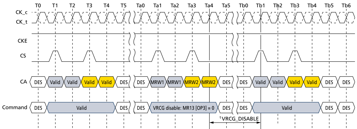
Figure 93: VRCG Disable Timing
