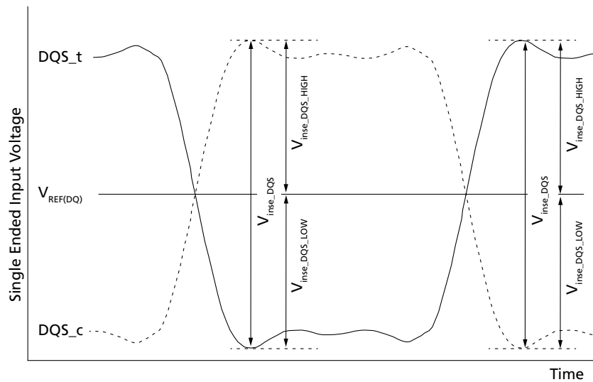
Figure 137: DQS Single-Ended Input Voltage
