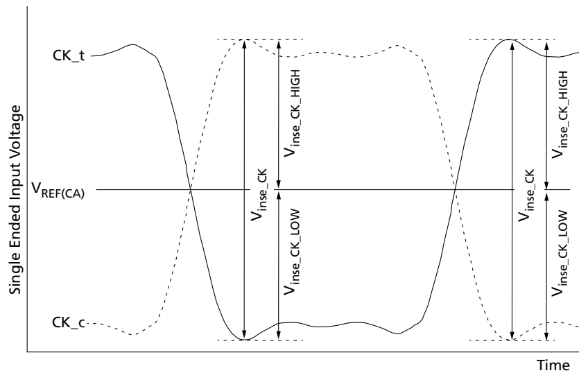
Figure 132: Clock Single-Ended Input Voltage
