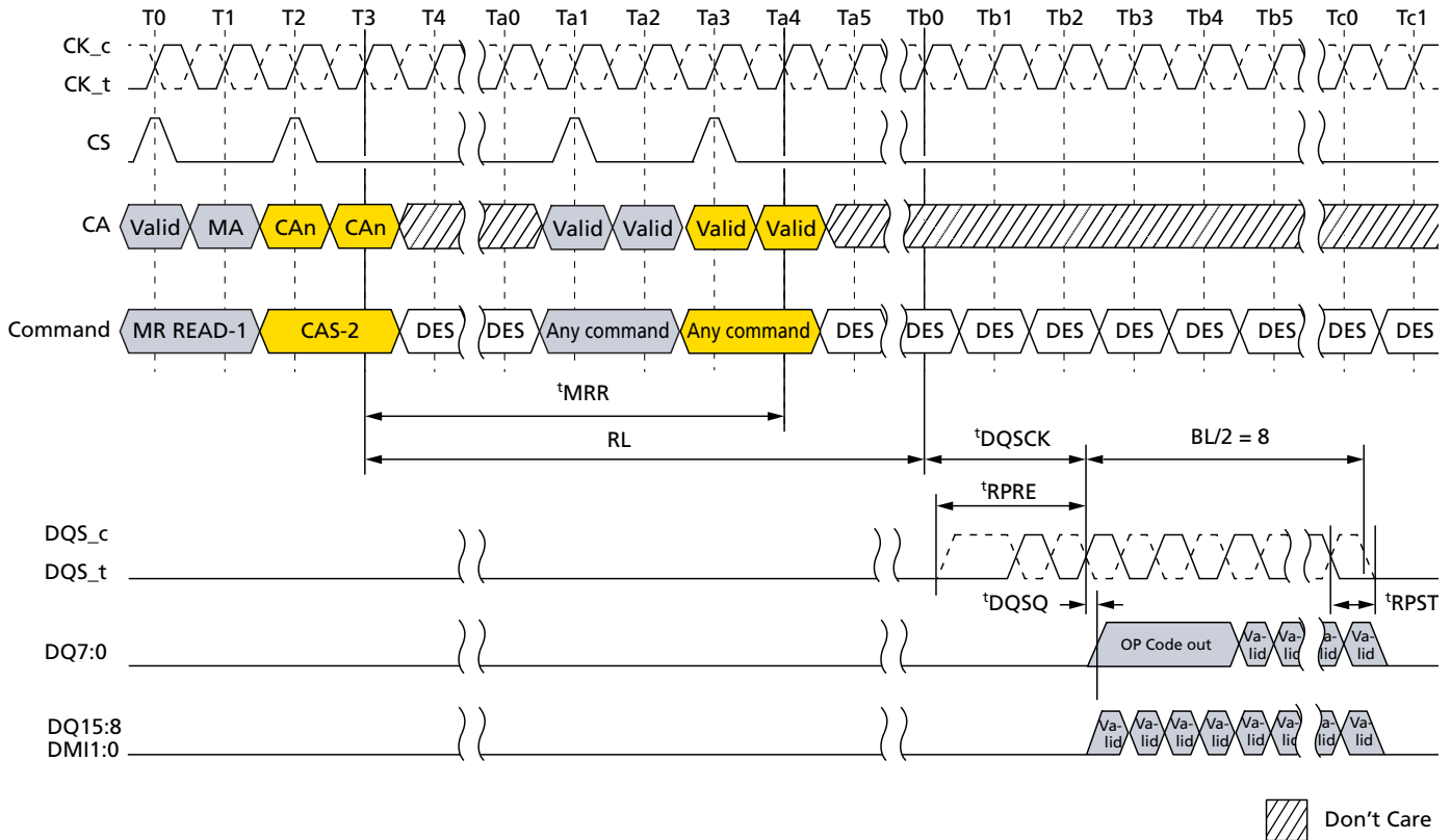
Figure 87: MODE REGISTER READ Operation
