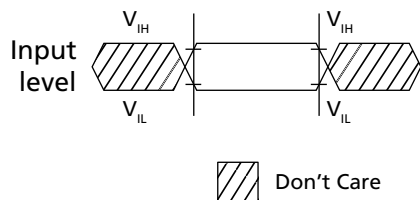
Figure 129: Input Timing Definition for RESET_n
