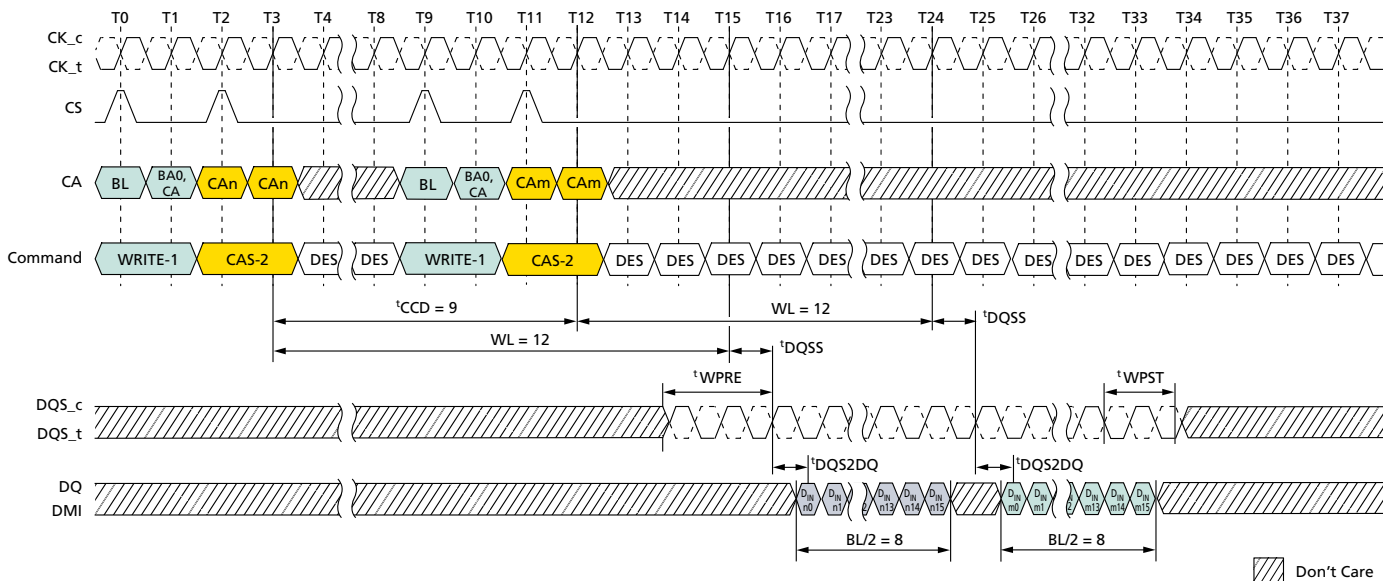
Figure 52: Consecutive WRITE: t_{CCD} = \text{MIN} + 1, 1.5nCK Postamble
