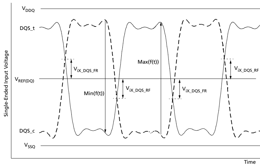
Figure 139: V_{IX} Definition (DQS)
