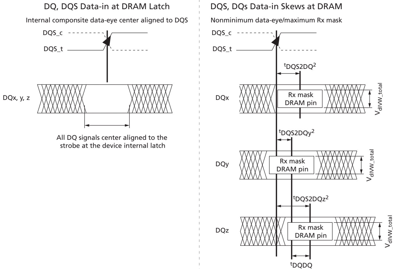
Figure 156: DQ-to-DQS t_{DQS2DQ} and t_{DQDQ}
