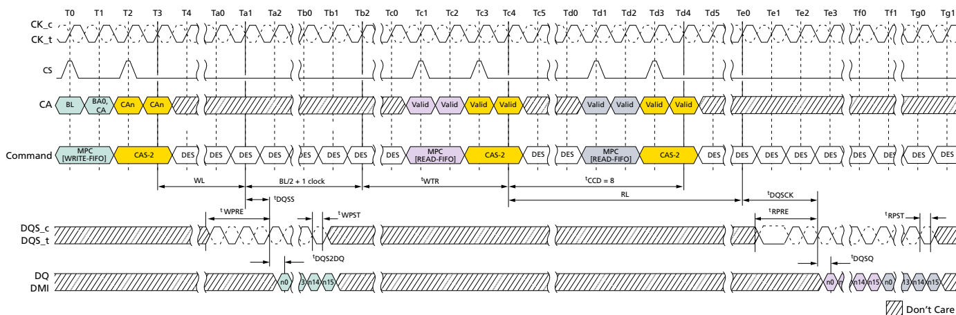
Figure 109: MPC[WRITE-FIFO]-to-MPC[READ-FIFO] Timing
