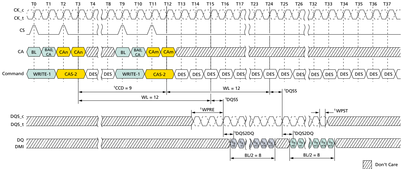
Figure 51: Consecutive WRITE: t_{CCD} = \text{MIN} + 1, 0.5nCK Postamble
