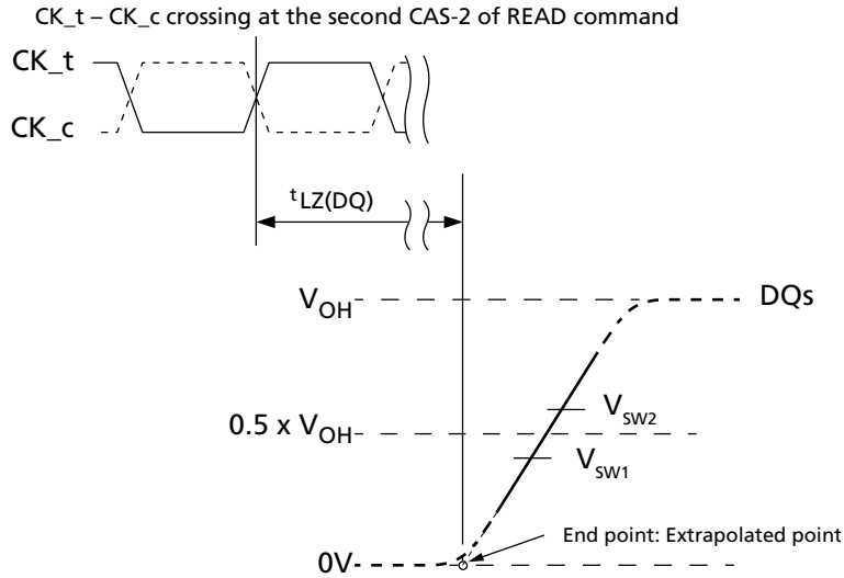
Figure 20: t_{LZ}(DQ) Method for Calculating Transitions and Endpoint
