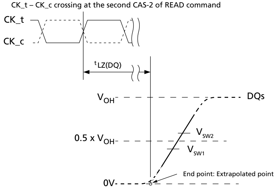
Figure 161: t_{LZ}(DQ) Method for Calculating Transitions and Endpoint
