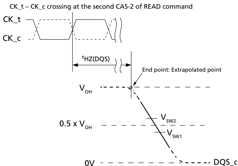
Figure 19: t_{HZ}(DQS) Method for Calculating Transitions and Endpoint
