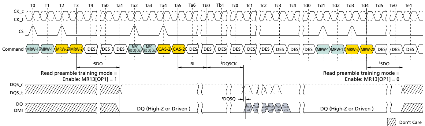
Figure 127: Read Preamble Training
