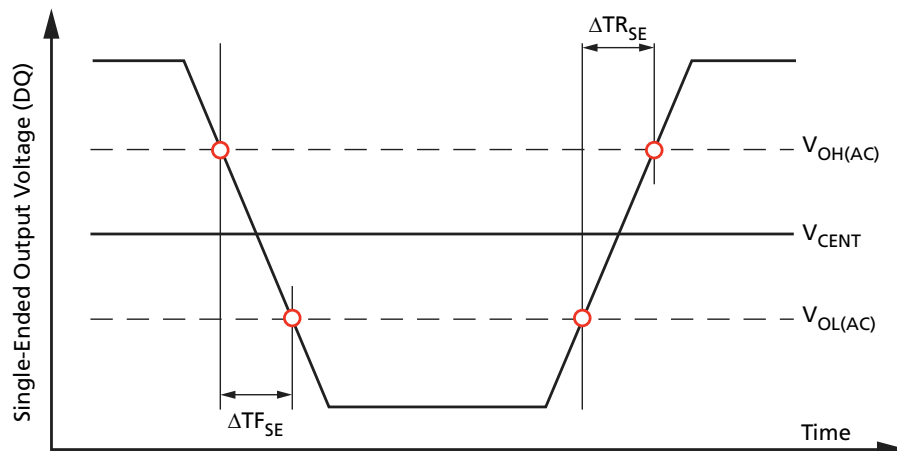
Figure 165: Single-Ended Output Slew Rate Definition
