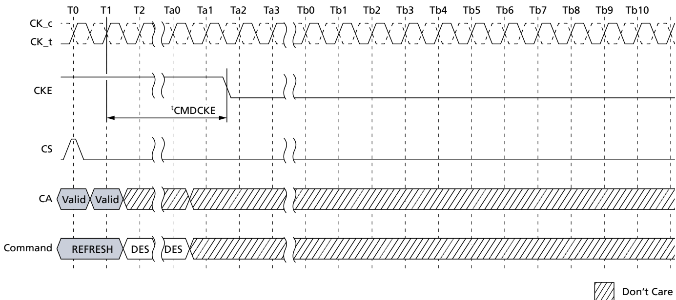
Figure 81: Refresh Entry to Power-Down Entry
