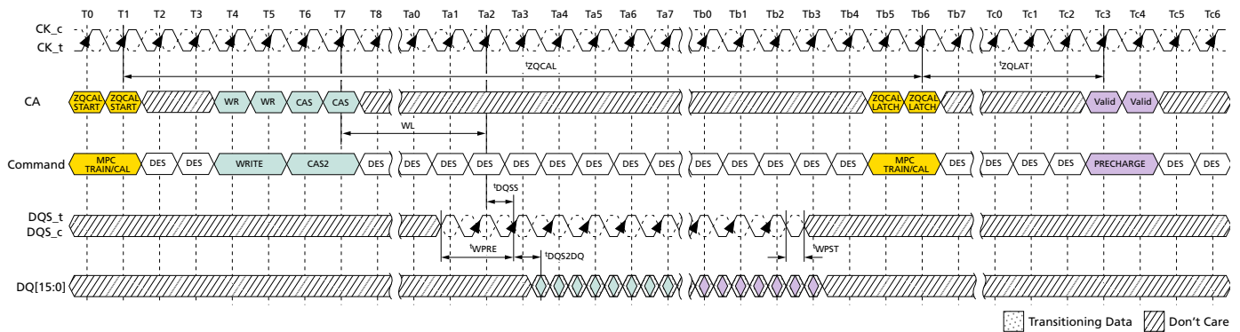
Figure 116: ZQCAL Timing
