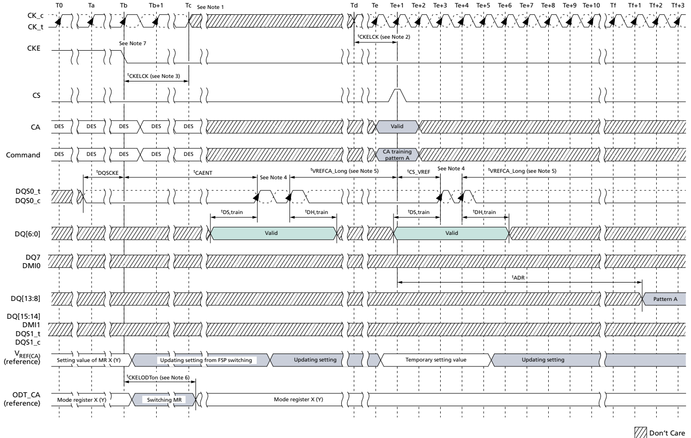
Figure 95: Consecutive V_{REF(CA)} Value Update
