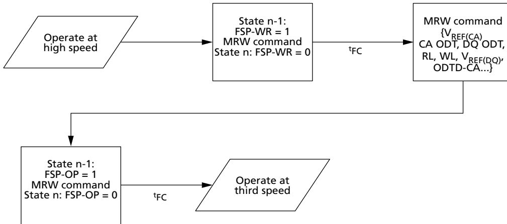
Figure 120: Example of Switching to a Third Trained Frequency Set Point
