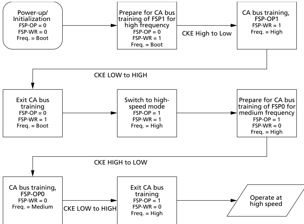
Figure 118: Training for Two Frequency Set Points
