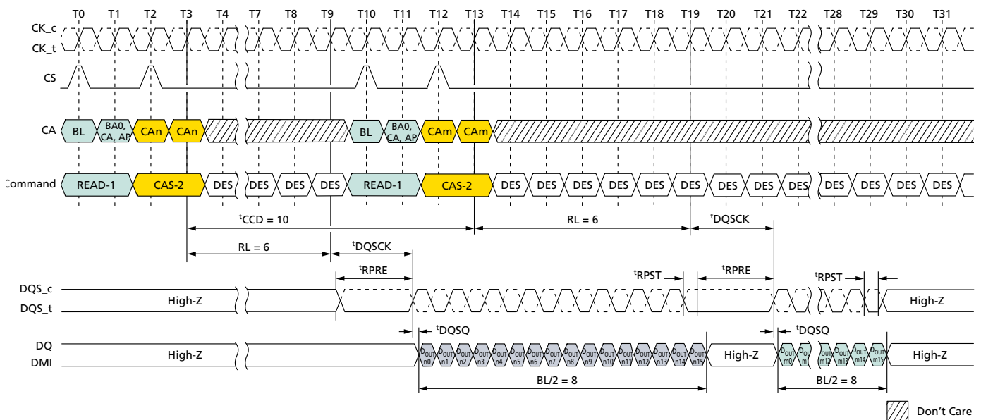
Figure 43: Consecutive READ: t_{CCD} = \text{MIN} + 2 , Preamble = Static, 0.5nCK Postamble
