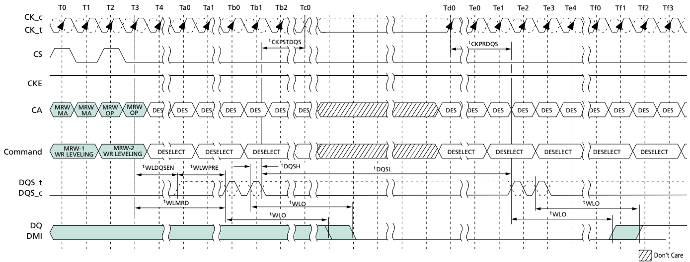
Figure 100: Clock Stop and Timing During Write Leveling
