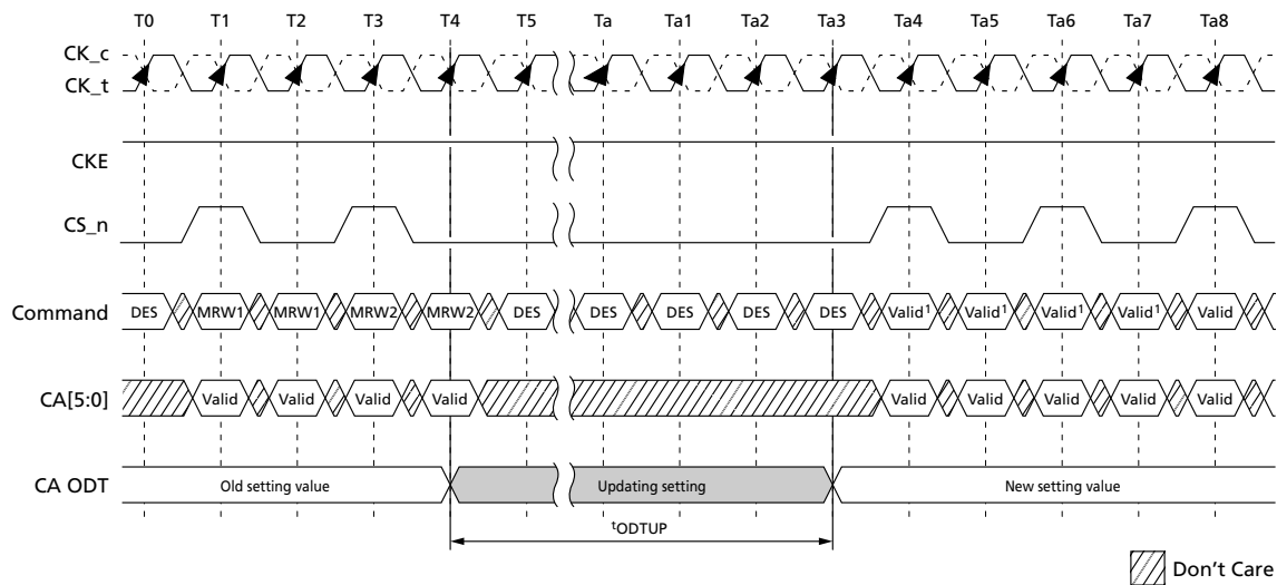
Figure 122: ODT for CA Setting Update Timing in 4-Clock Cycle Command
