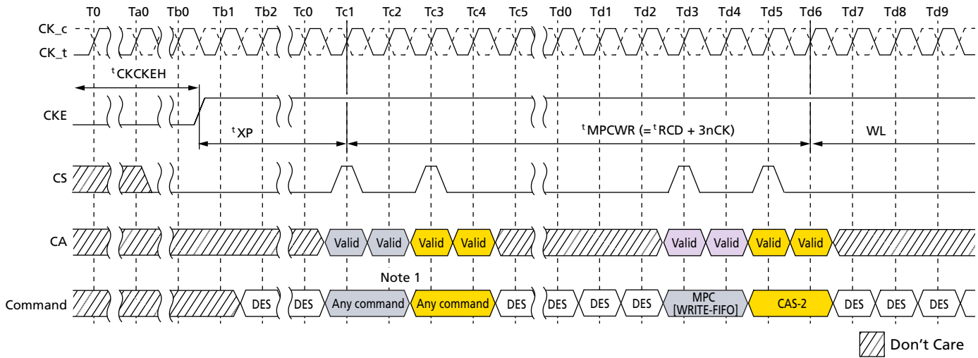
Figure 112: Power-Down Exit to MPC[WRITE-FIFO] Timing
