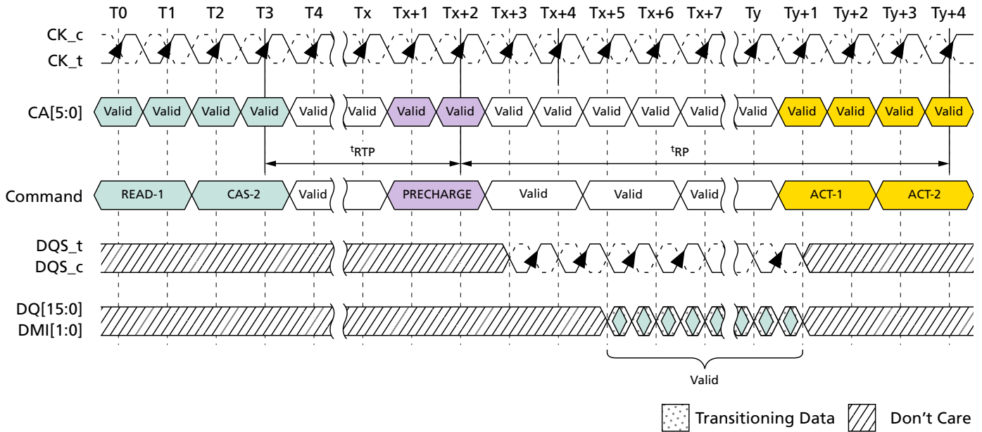
Figure 59: Burst READ Followed by Precharge – BL32, 2 t CK, 0.5nCK Postamble
