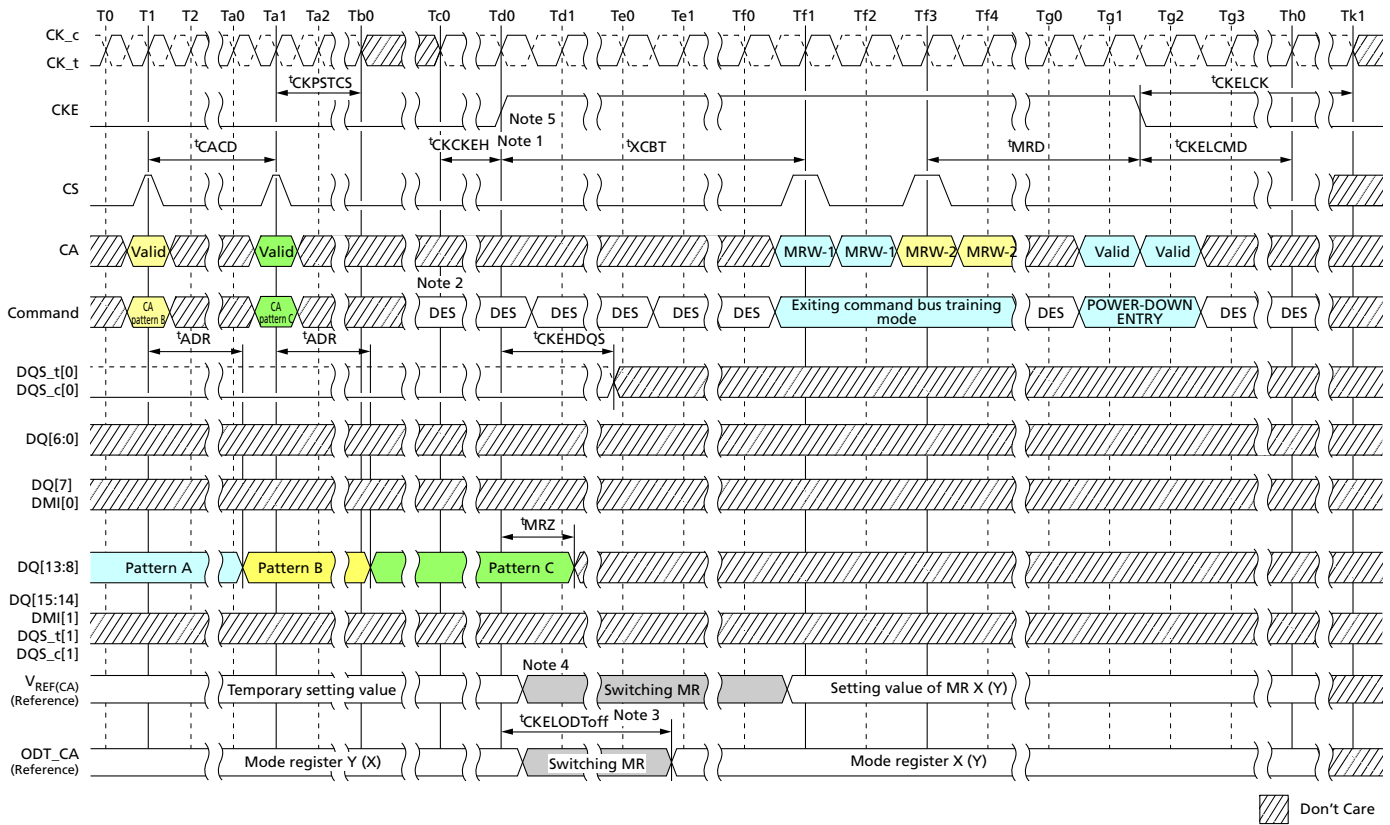
Figure 97: Command Bus Training Mode Exit with Power-Down Entry
