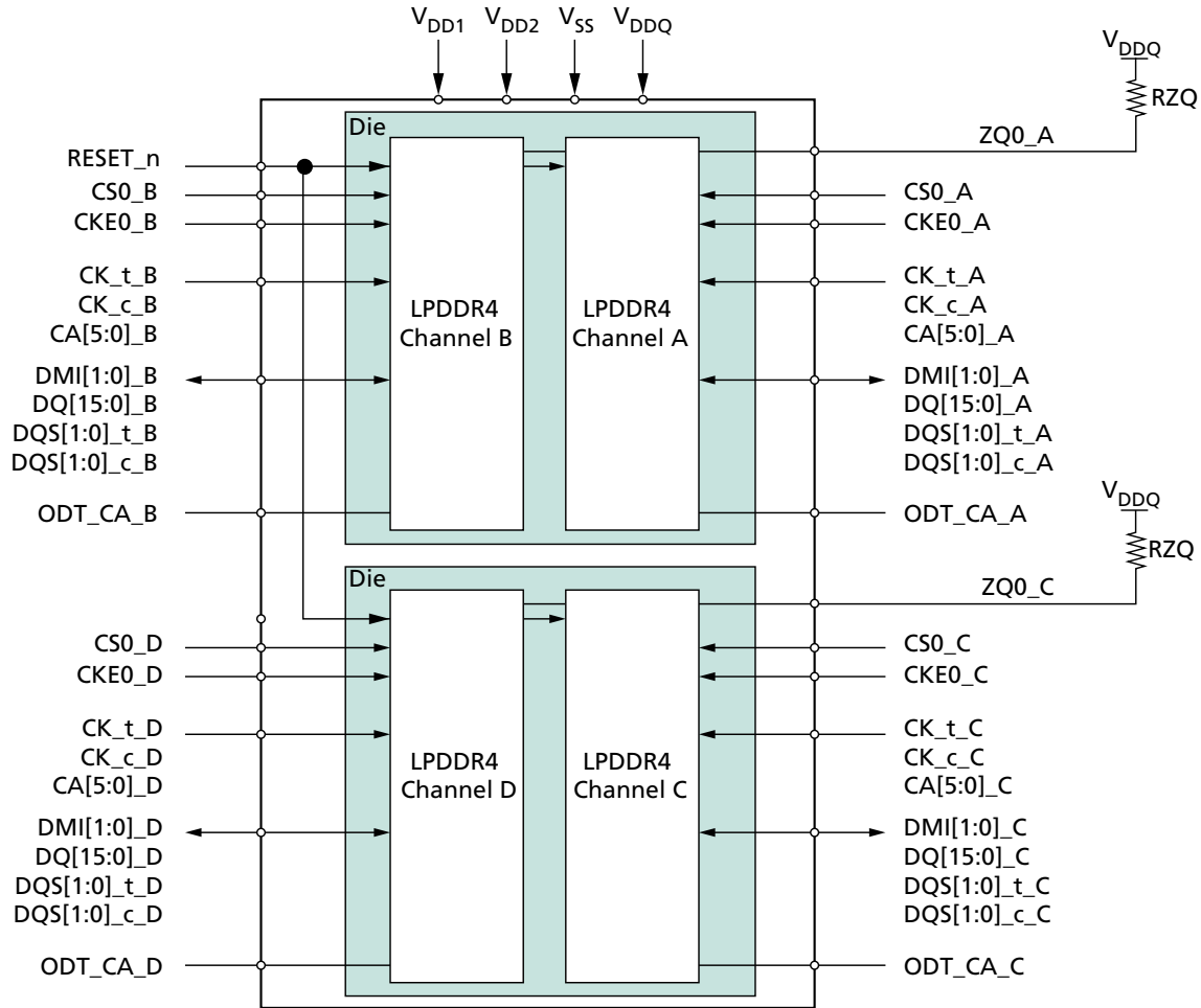
Figure 2: Dual-Die, Quad-Channel Package Block Diagram
