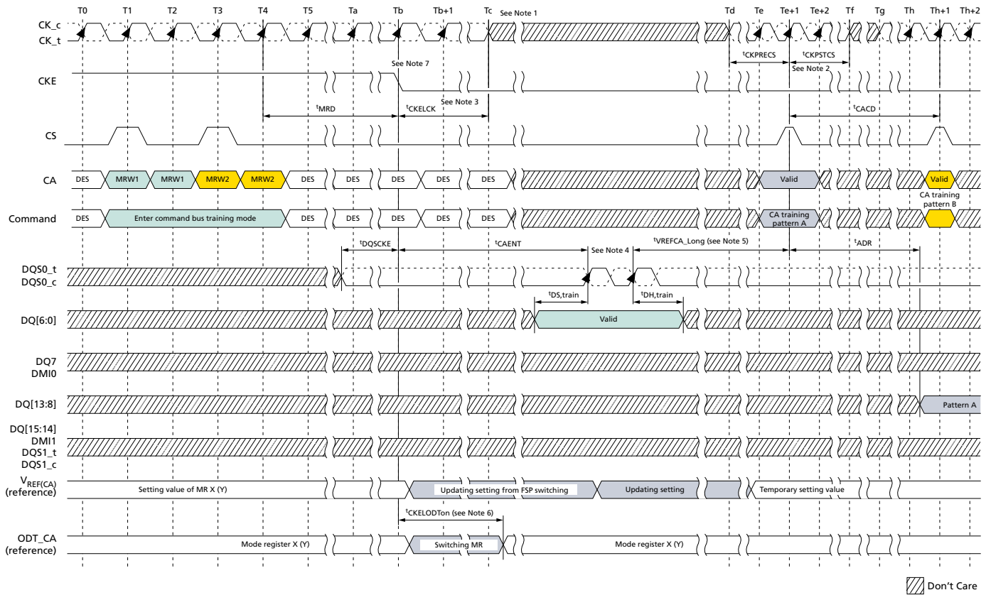
Figure 94: Command Bus Training Mode Entry – CA Training Pattern I/O with V_{REF(CA)} Value Update
