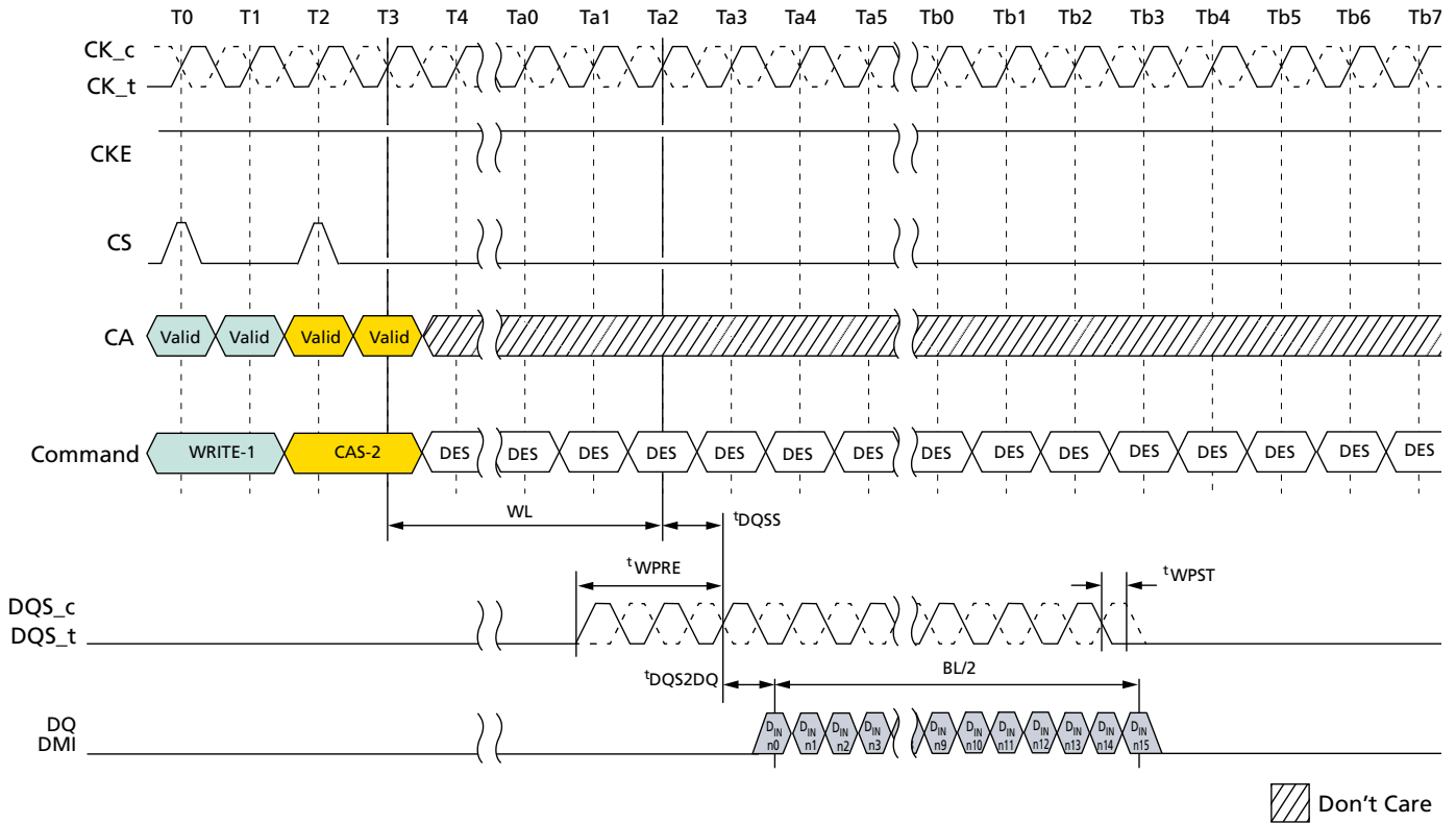
Figure 12: DQS Write Preamble and Postamble – 0.5nCK Postamble
