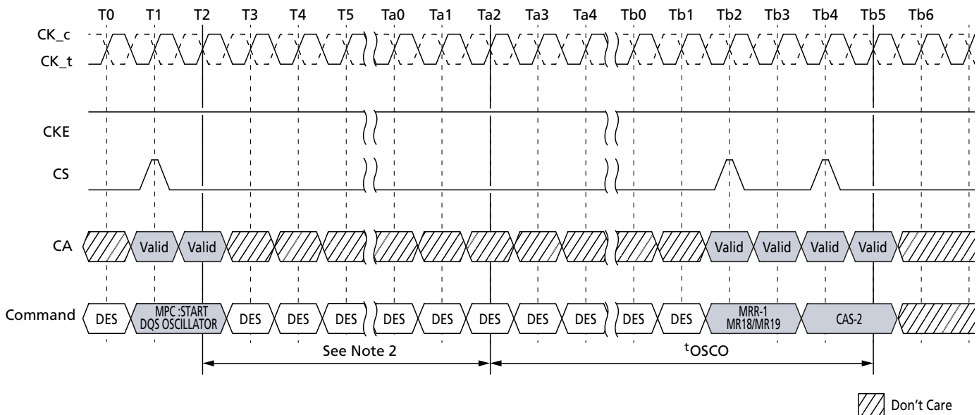
Figure 115: In Case of DQS Interval Oscillator is Stopped by DQS Interval Timer
