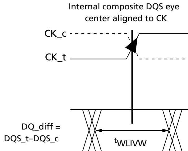
Figure 101: DQS_t/DQS_c to CK_t/CK_c Timings at the Pins Referenced from the Internal Latch
