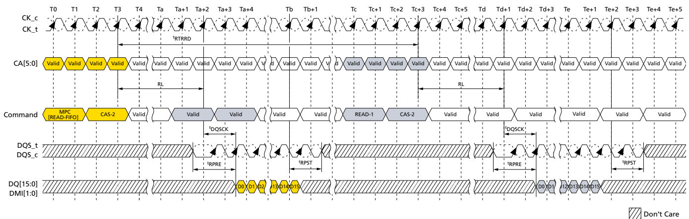
Figure 104: READ-FIFO – t_{RPRE} = \text{Toggle} , t_{RPST} = 1.5nCK
