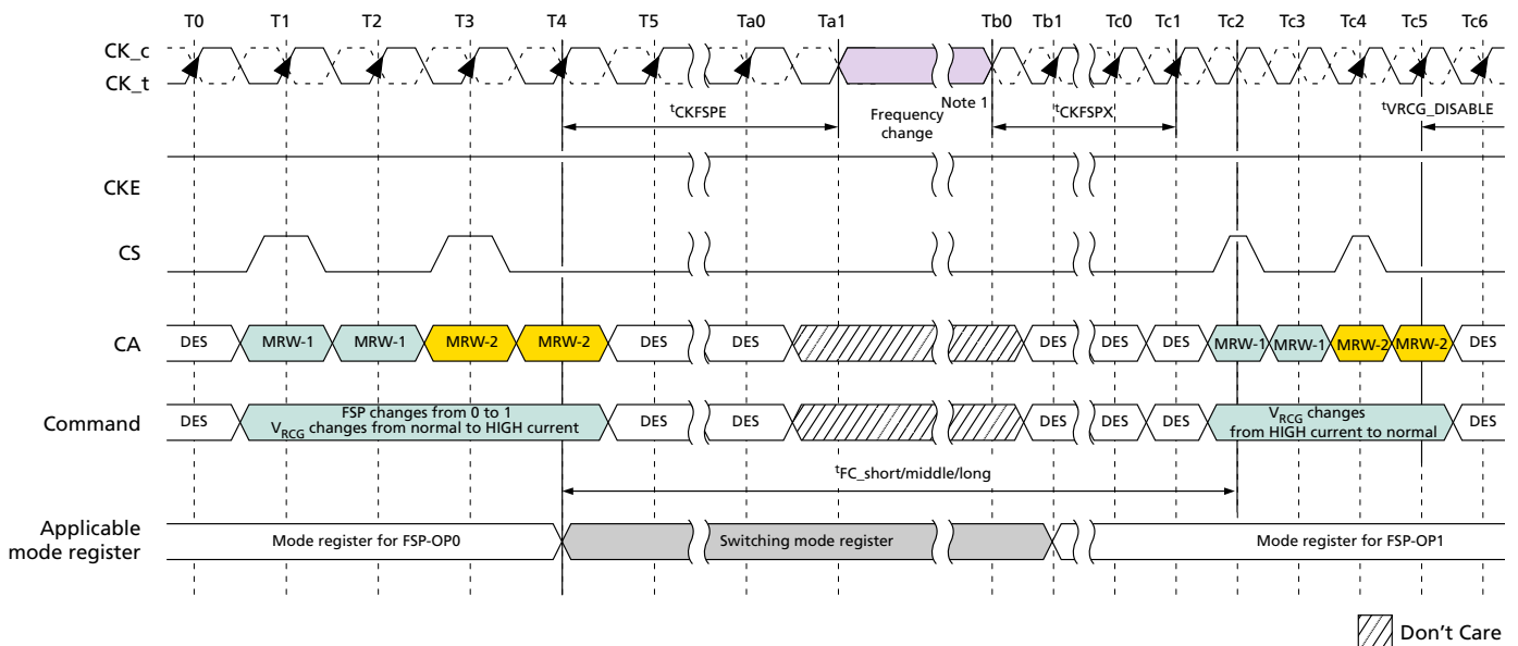
Figure 117: Frequency Set Point Switching Timing
