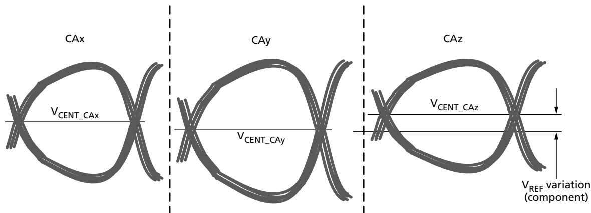
Figure 149: Across Pin V_{REF} (CA) Voltage Variation
