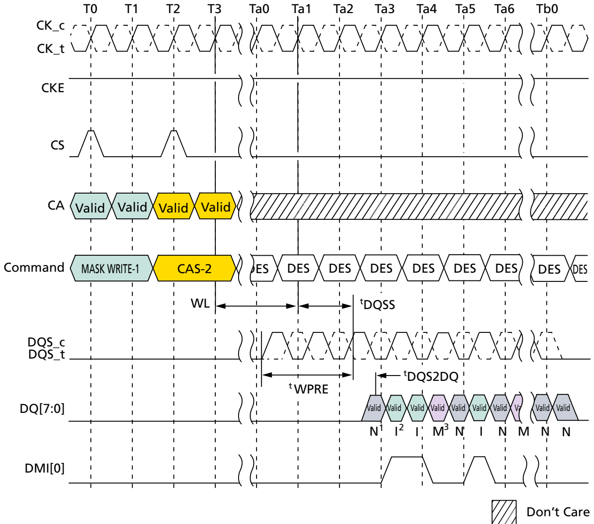
Figure 29: MASKED WRITE Command with Write DBI Enabled; DM Enabled
