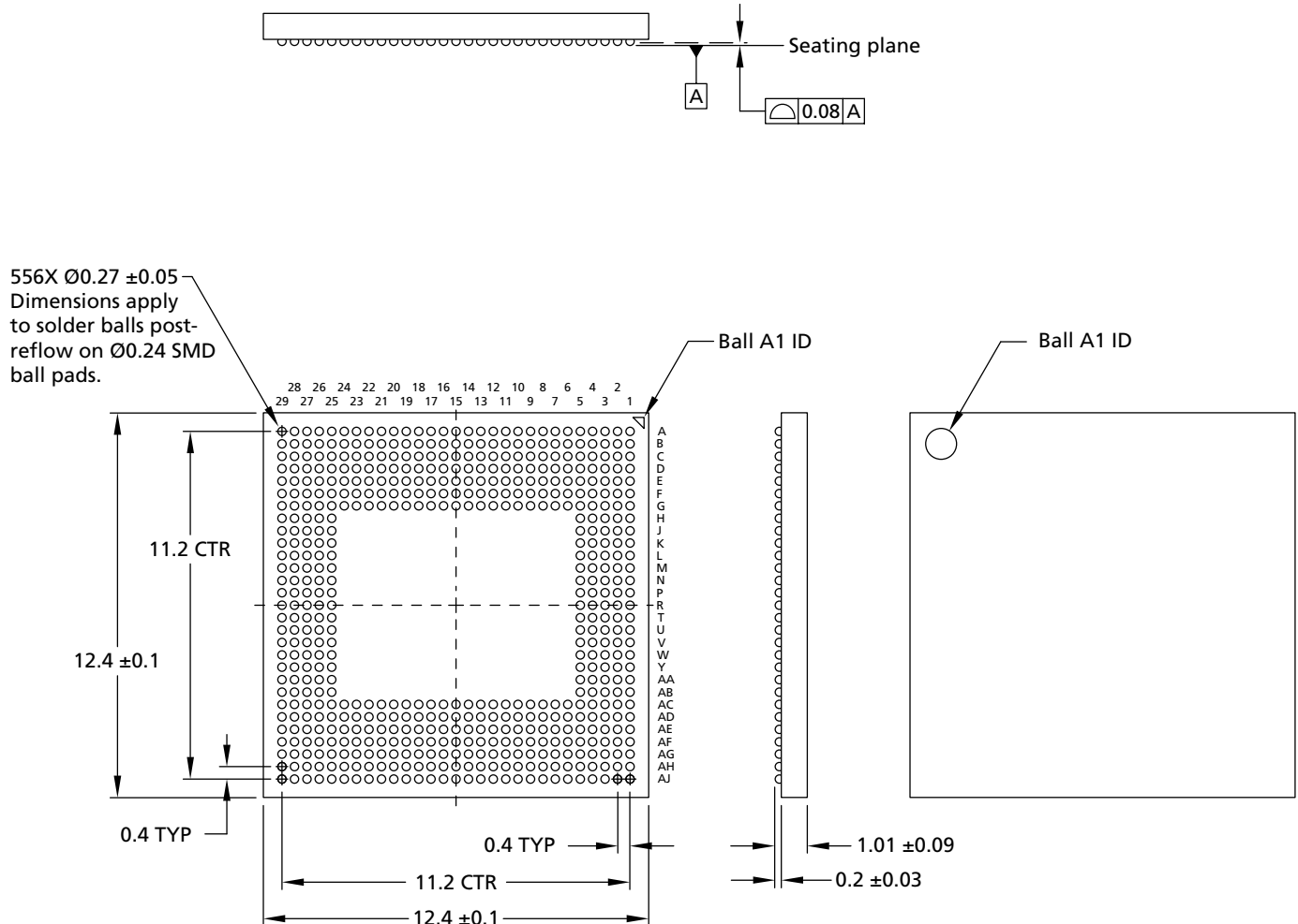
Figure 4: 556-Ball TFBGA – 12.4mm x 12.4mm x 1.1mm (Package Code: HJ)
