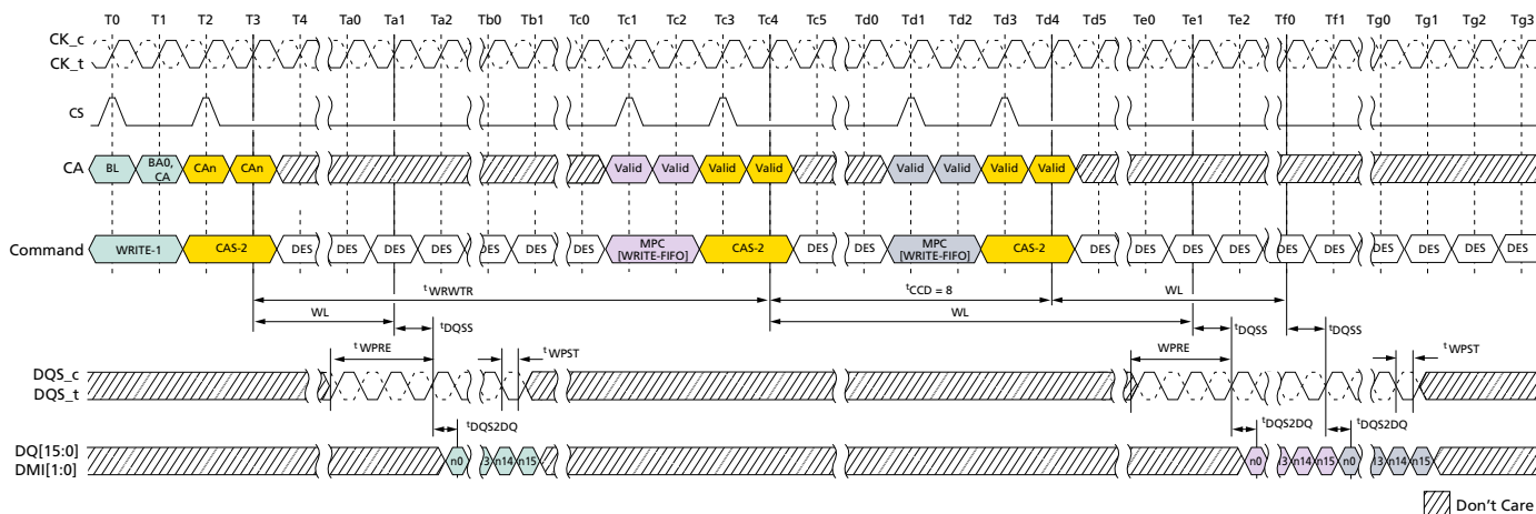
Figure 108: WRITE-to-MPC[WRITE-FIFO] Operation Timing
