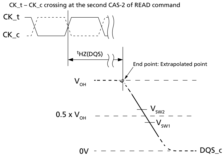
Figure 160: t_{HZ}(DQS) Method for Calculating Transitions and Endpoint
