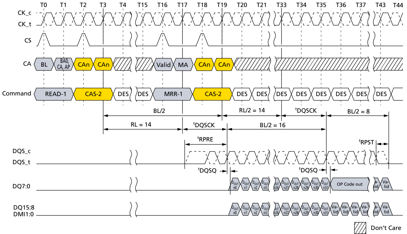
Figure 88: READ-to-MRR Timing
