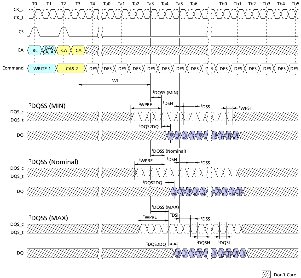
Figure 24: Write Timing
