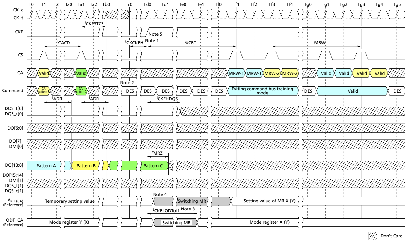
Figure 96: Command Bus Training Mode Exit with Valid Command
