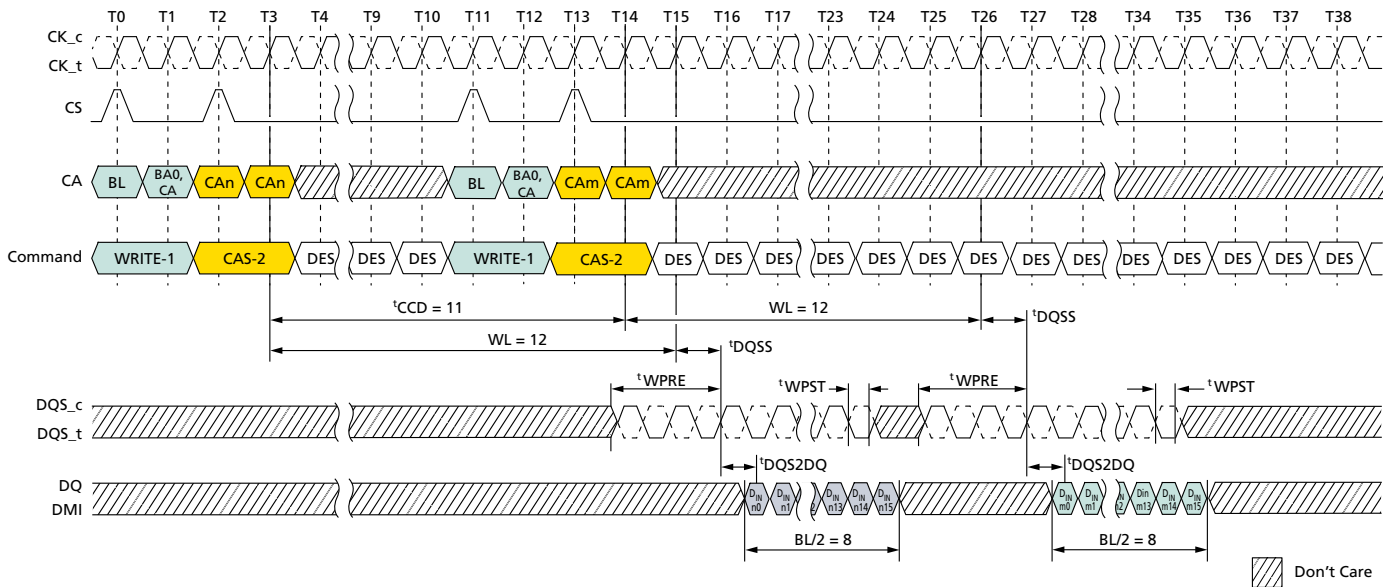
Figure 55: Consecutive WRITE: t_{CCD} = \text{MIN} + 3, 0.5nCK Postamble
