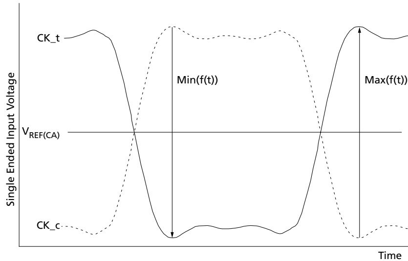
Figure 131: Definition of Differential Clock Peak Voltage
