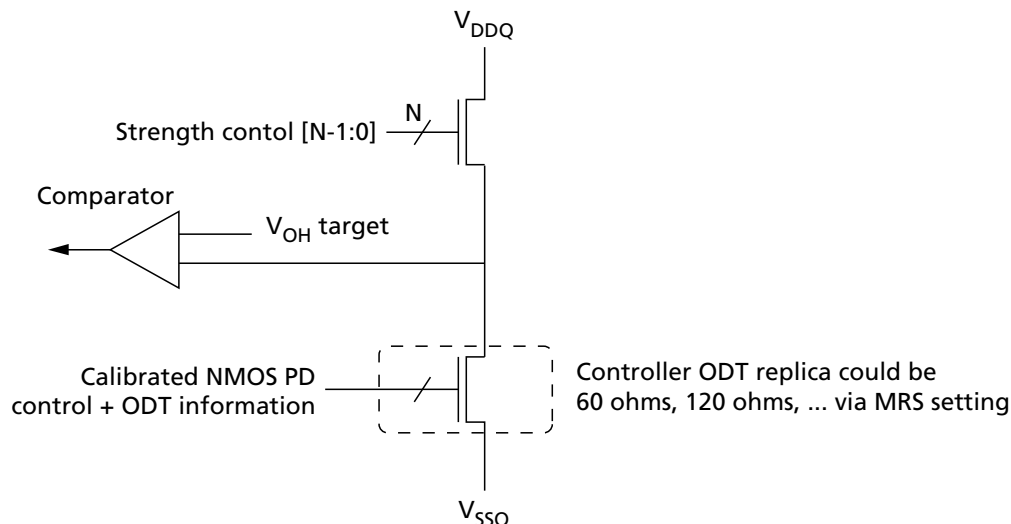
Figure 145: Pull-Up Calibration
