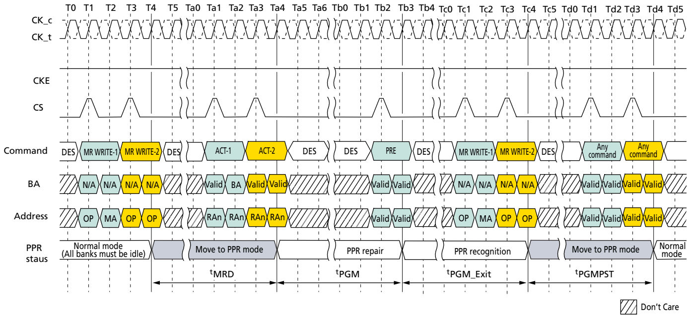
Figure 126: Post-Package Repair Timing
