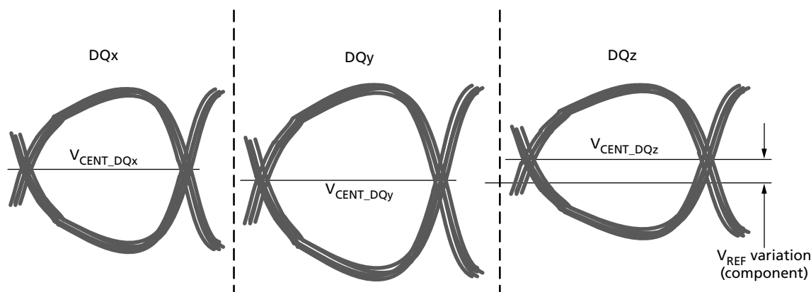
Figure 155: Across Pin V_{REF} DQ Voltage Variation
