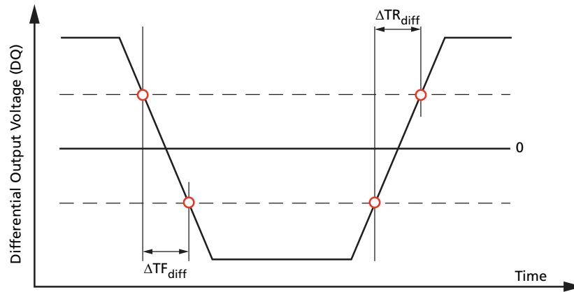
Figure 141: Differential Output Slew Rate Definition
