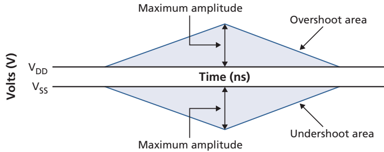
Figure 142: Overshoot and Undershoot Definition
