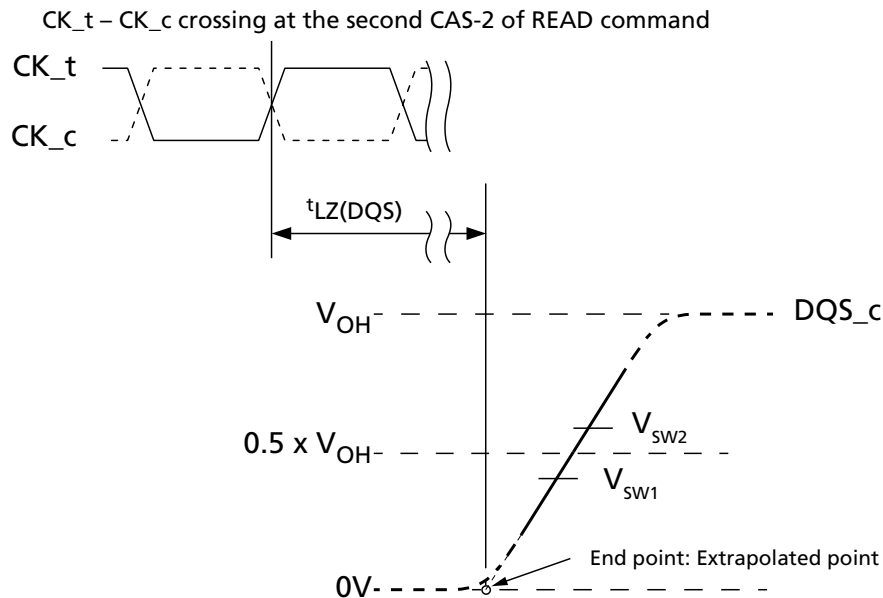
Figure 159: t_{LZ}(DQS) Method for Calculating Transitions and Endpoint
