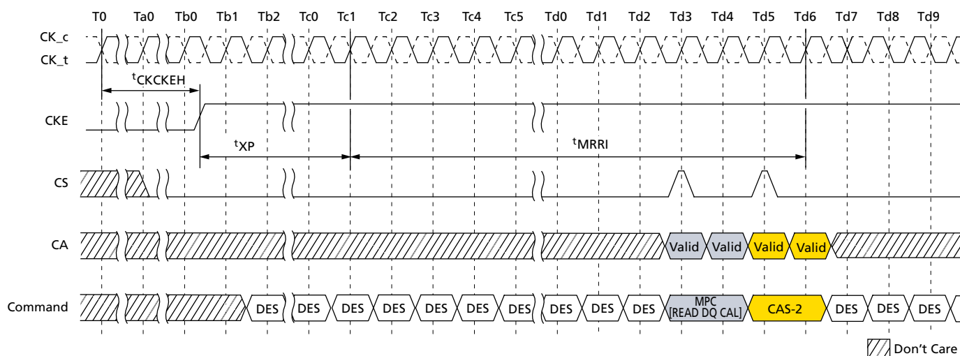
Figure 107: MPC[READ DQ CALIBRATION] Following Power-Down State
