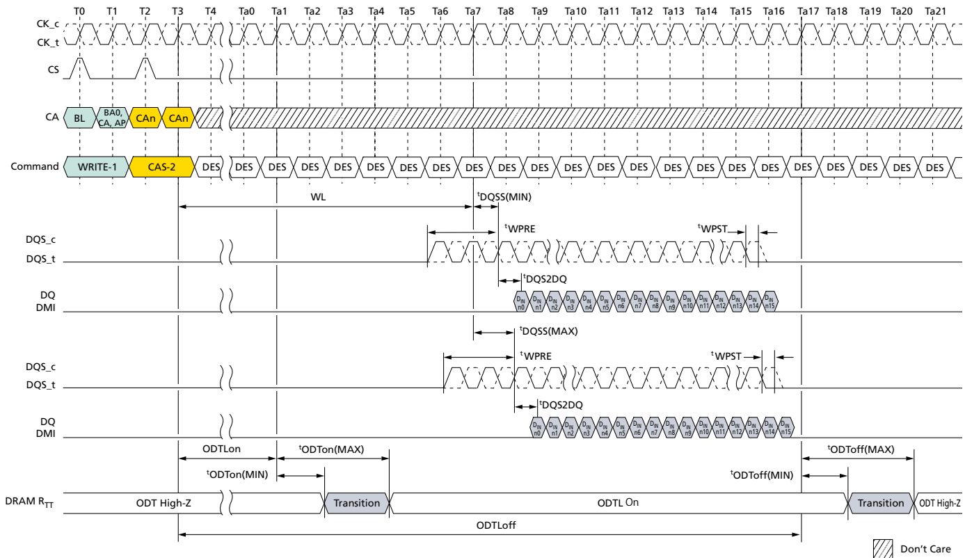
Figure 124: Asynchronous ODTon/ODToff Timing
