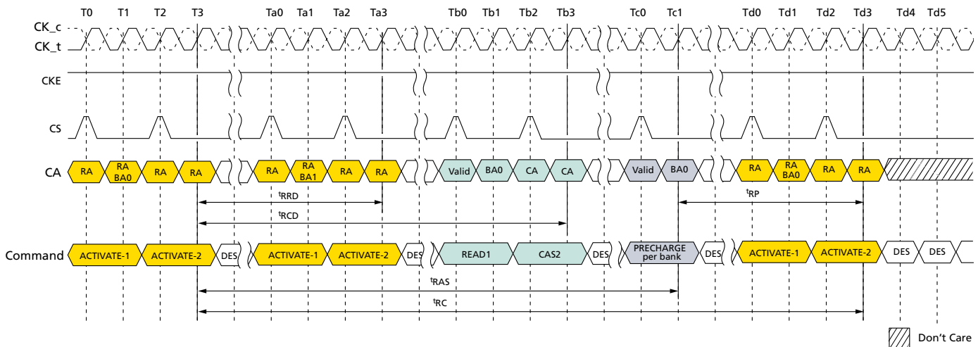
Figure 8: ACTIVATE Command
