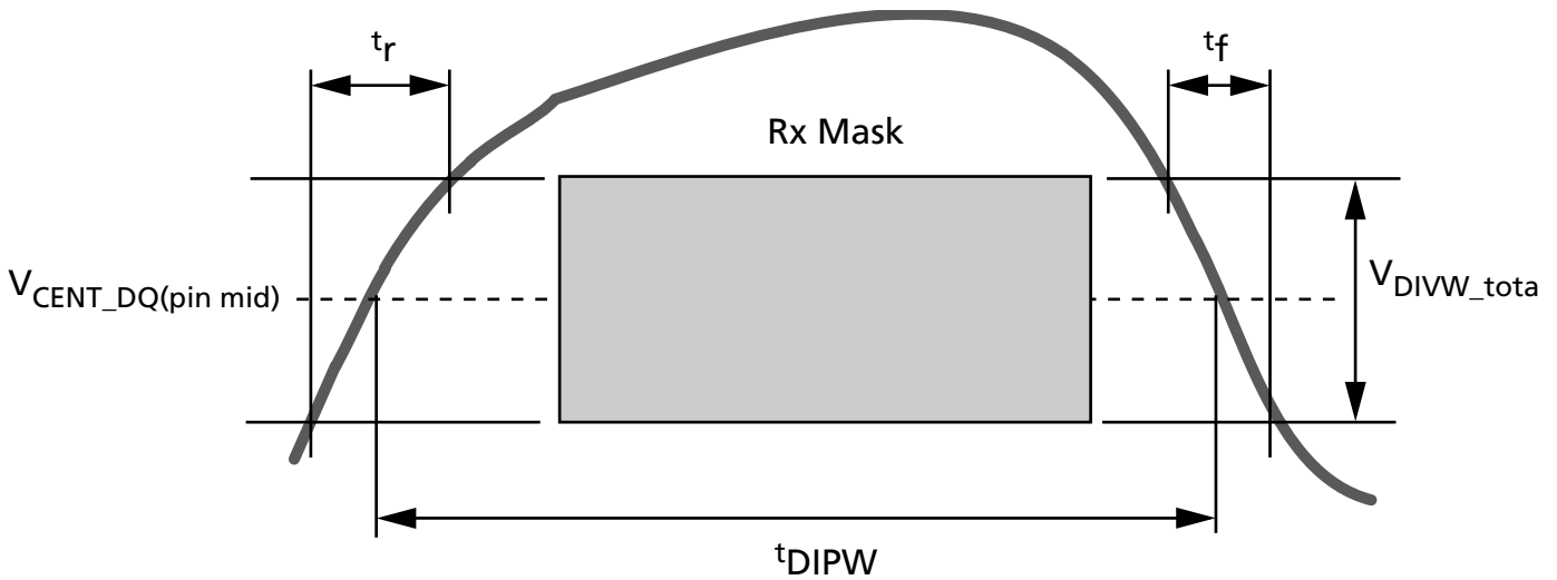
Figure 157: DQ t_{DIPW} and SRIN_dIVW Definition for Each Input Pulse
