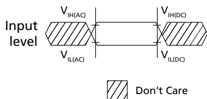
Figure 128: Input Timing Definition for CKE
