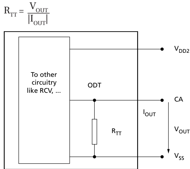
Figure 163: ODT for CA
