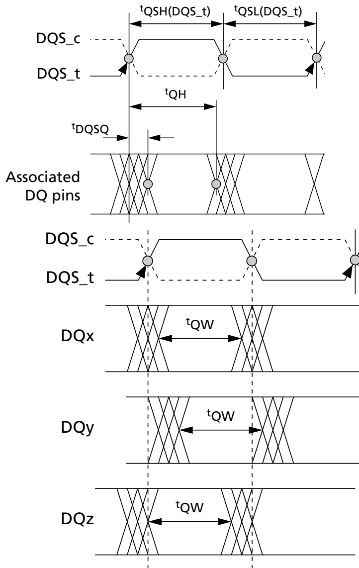
Figure 153: Read Data Timing Definitions – t_{QH} and t_{DQSQ} Across DQ Signals per DQS Group
