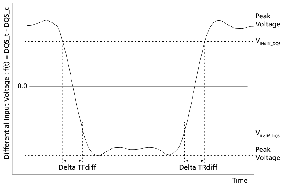
Figure 138: Differential Input Slew Rate Definition for DQS t , DQS c
