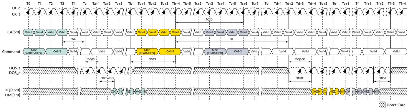
Figure 103: READ-FIFO – t_{WPRE} = 2nCK , t_{WPST} = 0.5nCK , t_{RPRE} = \text{Toggle} , t_{RPST} = 1.5nCK
