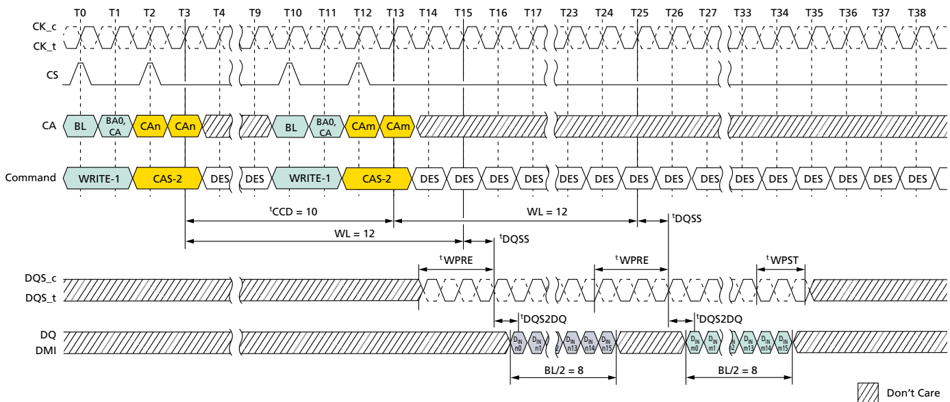
Figure 54: Consecutive WRITE: t_{CCD} = MIN + 2, 1.5nCK Postamble
