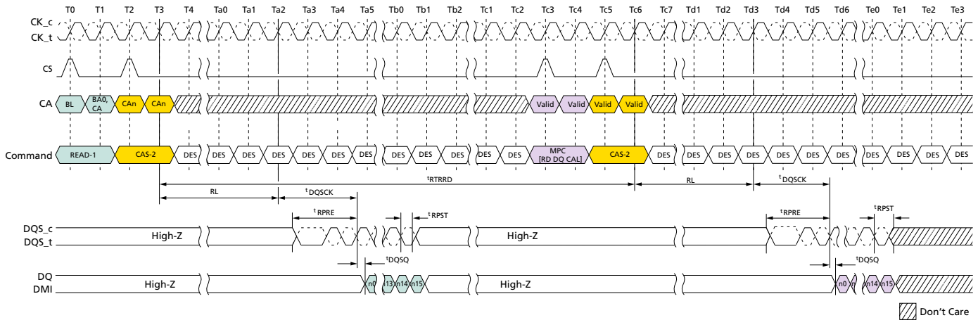
Figure 105: Read DQ Calibration Training Timing: Read-to-Read DQ Calibration
