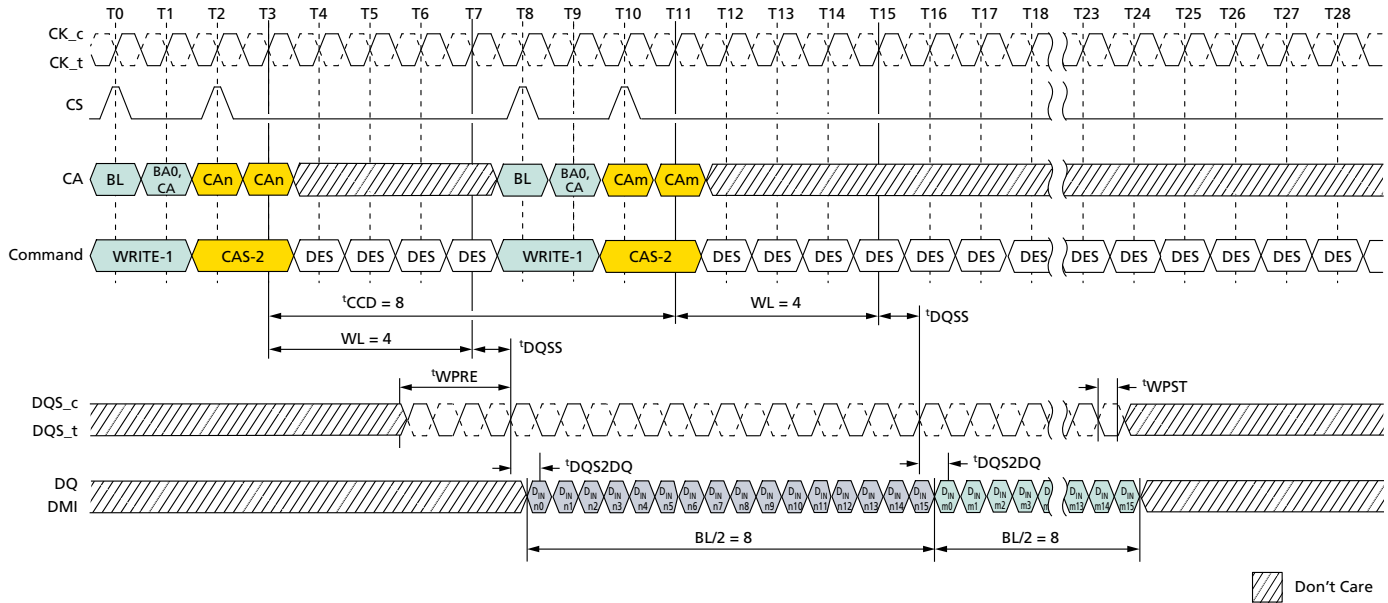
Figure 48: Seamless WRITE: t_{CCD} = \text{MIN}, 0.5nCK Postamble
