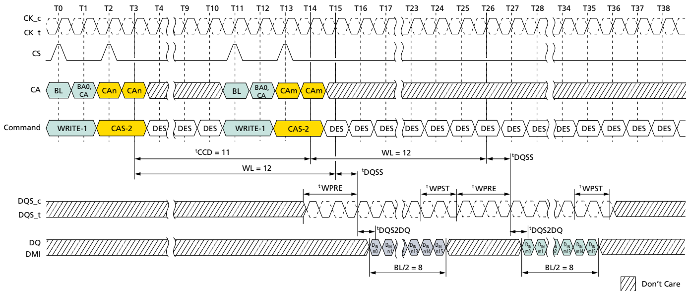
Figure 56: Consecutive WRITE: t_{CCD} = \text{MIN} + 3, 1.5nCK Postamble
