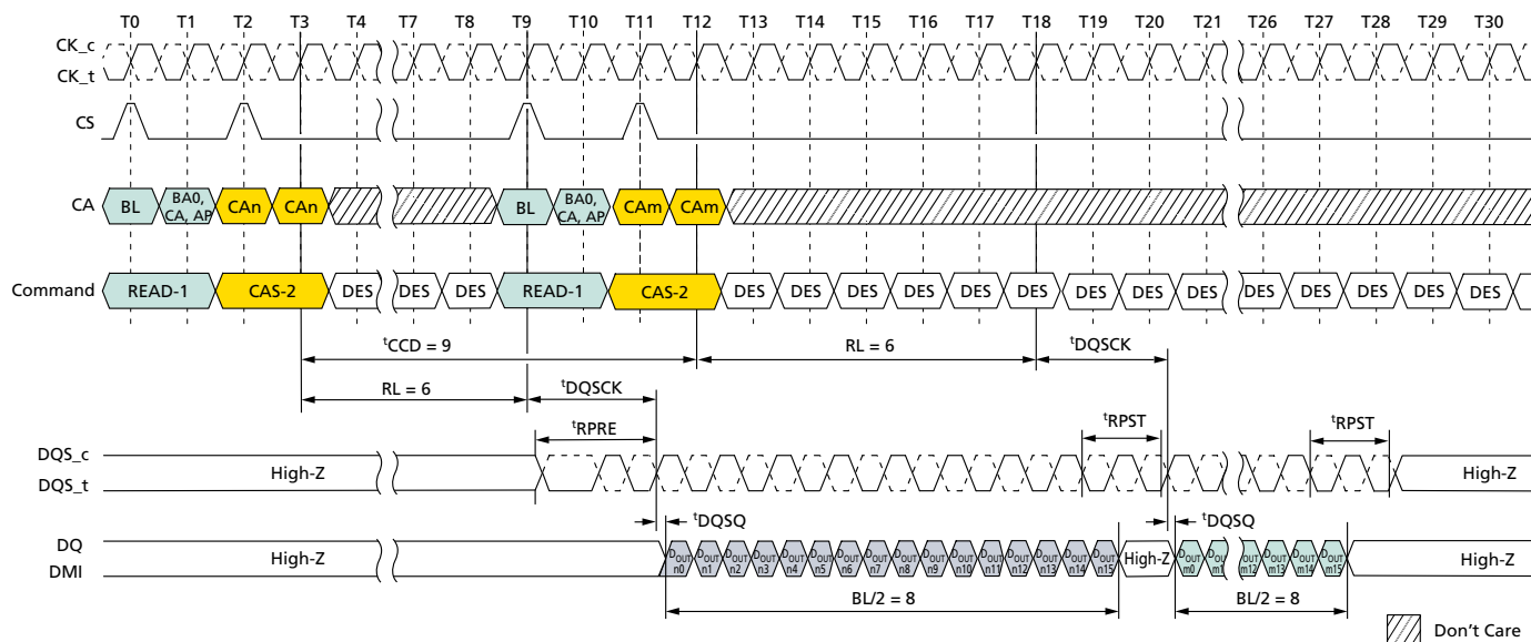
Figure 36: Seamless READ: t_{CCD} = MIN + 1 , Preamble = Toggle, 1.5nCK Postamble
