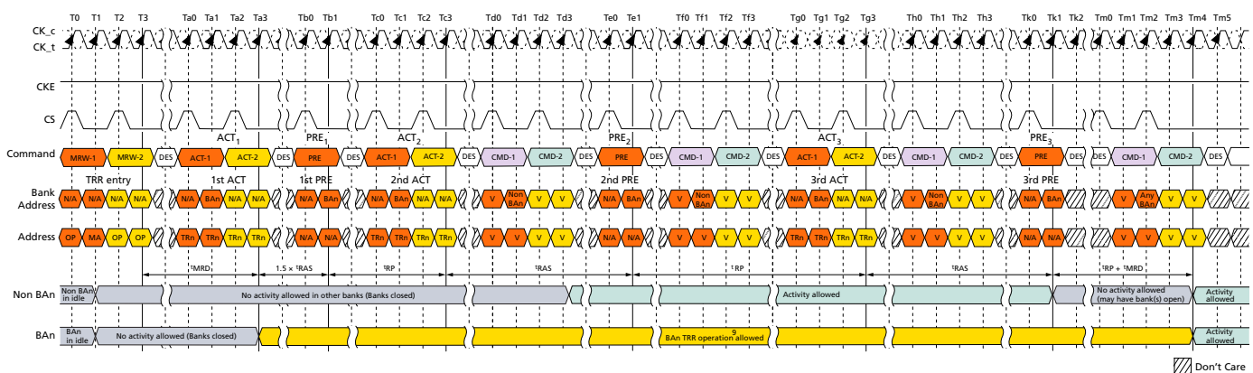
Figure 125: Target Row Refresh Mode
