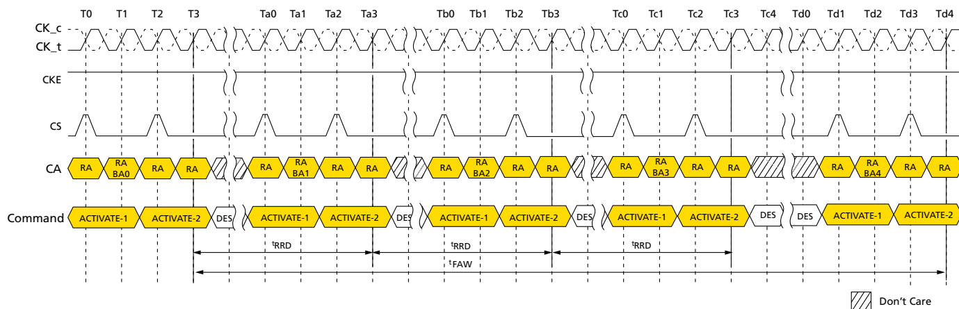
Figure 9: t_{FAW} Timing
