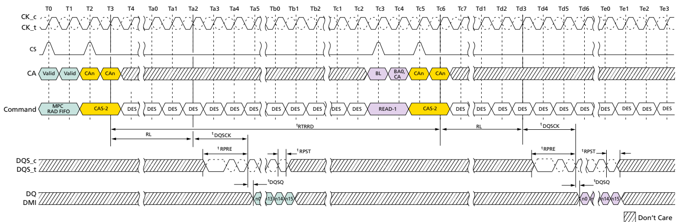
Figure 110: MPC[READ-FIFO] to Read Timing
