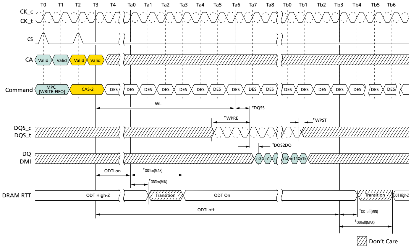
Figure 111: MPC[WRITE-FIFO] with DQ ODT Timing
