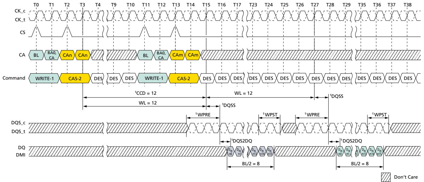
Figure 57: Consecutive WRITE: t_{CCD} = \text{MIN} + 4, 1.5nCK Postamble
