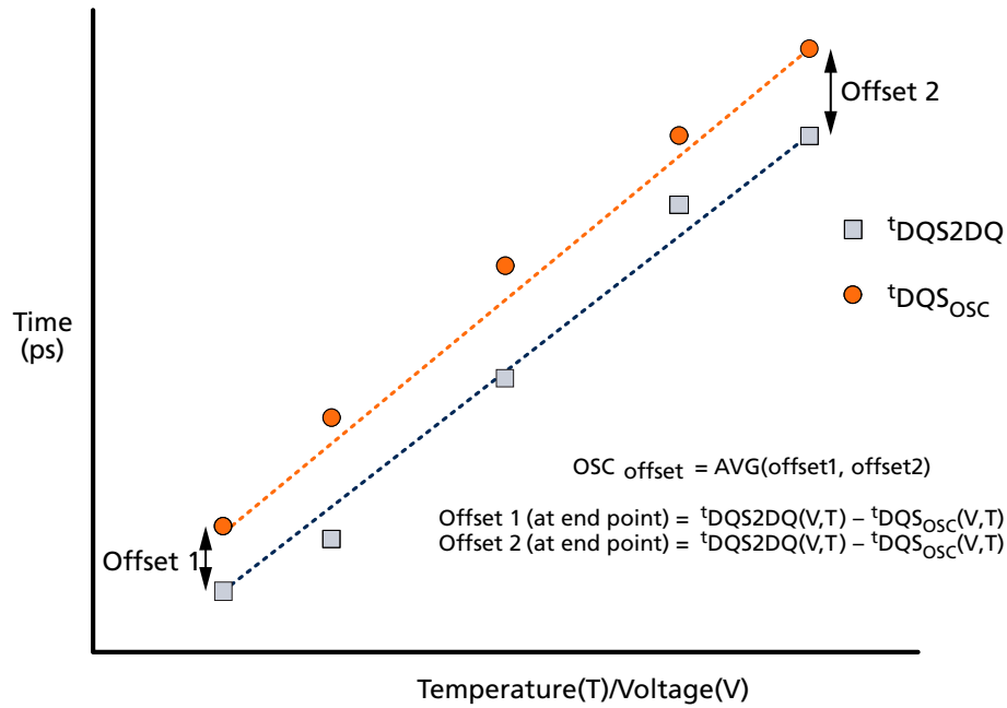
Figure 113: Interval Oscillator Offset – OSC_{offset}
