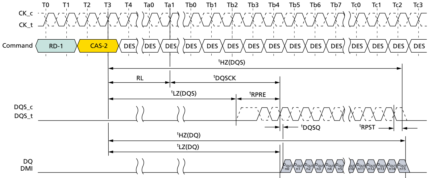
Figure 17: Read Timing
