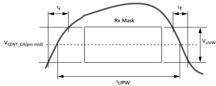
Figure 151: CA t_{clPW} and SRIN_cIVW Definition (for Each Input Pulse)
