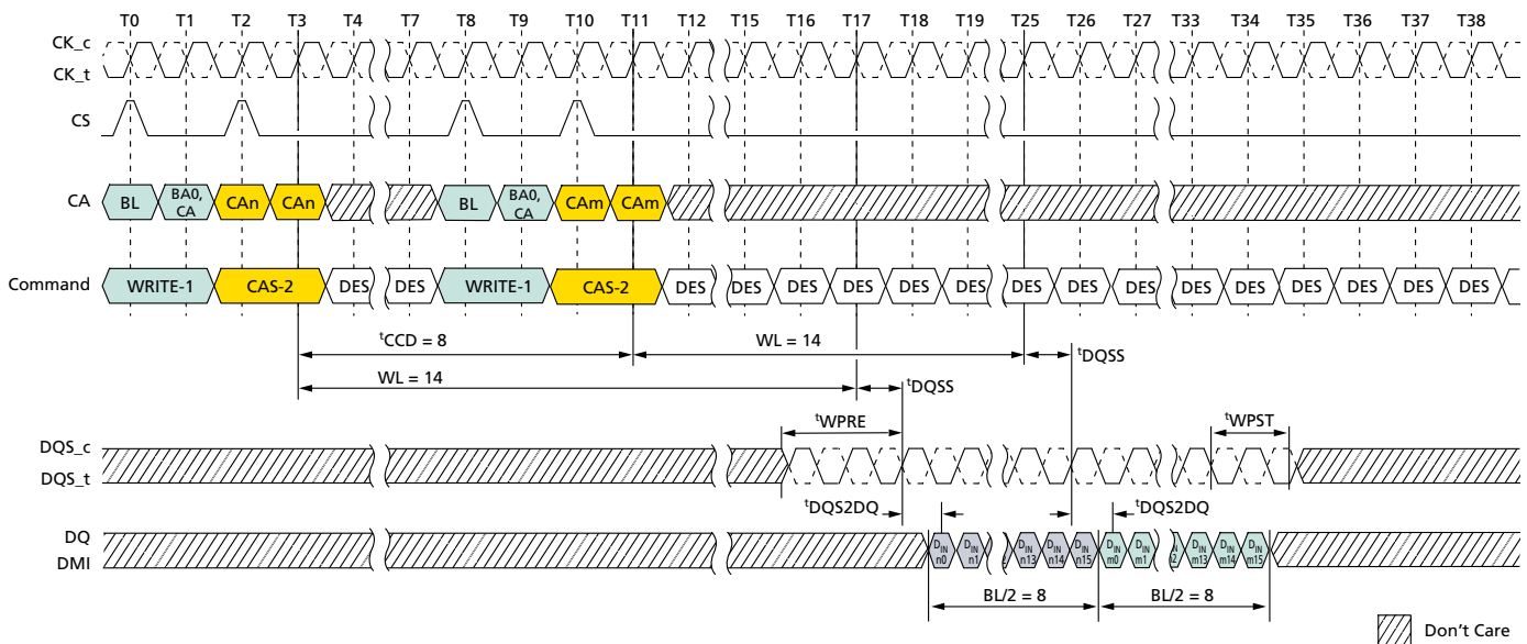
Figure 50: Seamless WRITE: t_{CCD} = \text{MIN} , 1.5n\text{CK} Postamble
