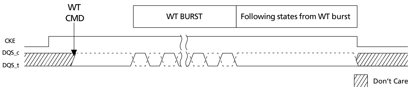
Figure 31: WDQS Control Mode 1
