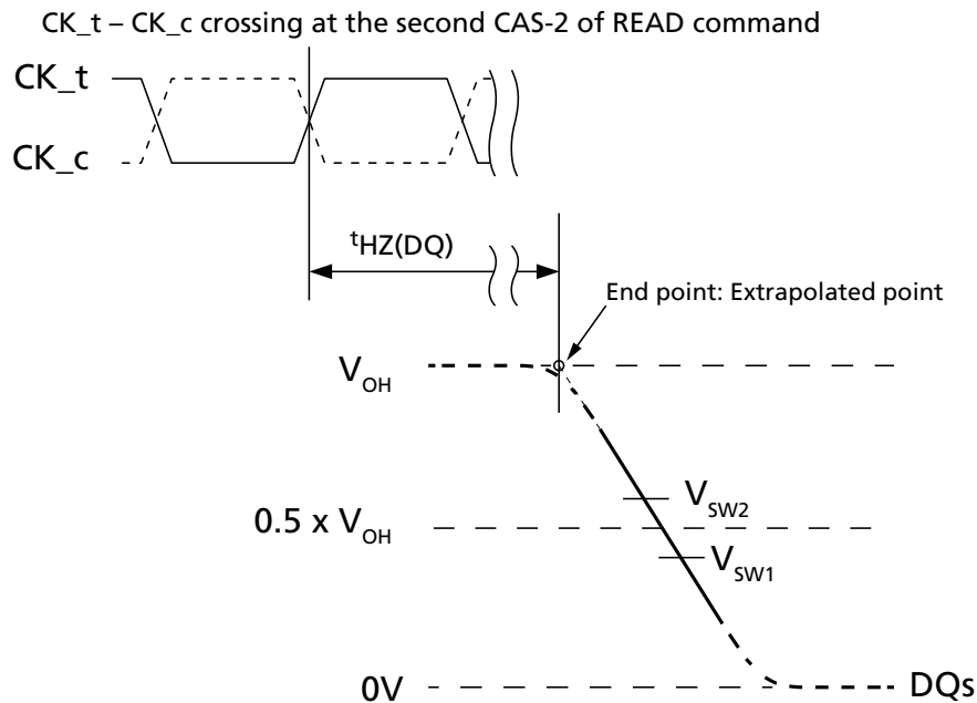
Figure 162: t_{HZ}(DQ) Method for Calculating Transitions and Endpoint
