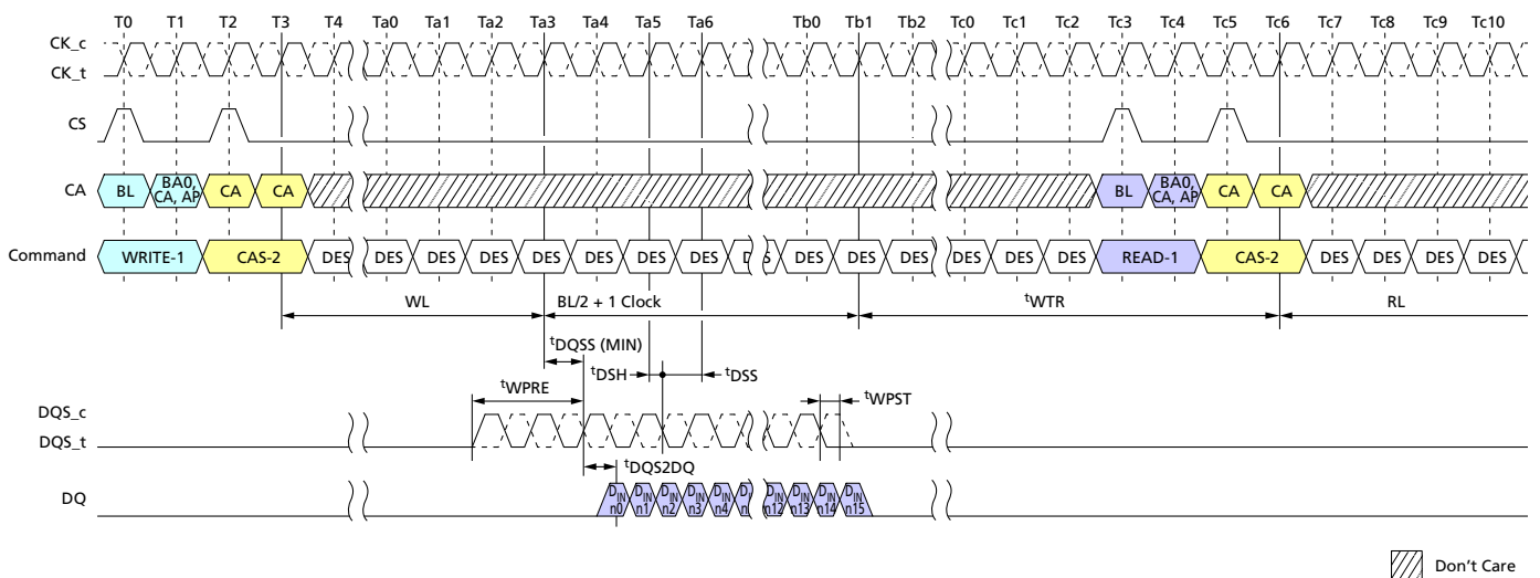
Figure 23: Burst Write Followed by Burst Read
