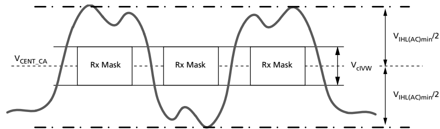
Figure 152: CA V_{IHL\_AC} Definition (for Each Input Pulse)
