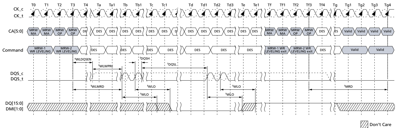
Figure 98: Write Leveling Timing – t_{DQSL}(\text{MAX})
