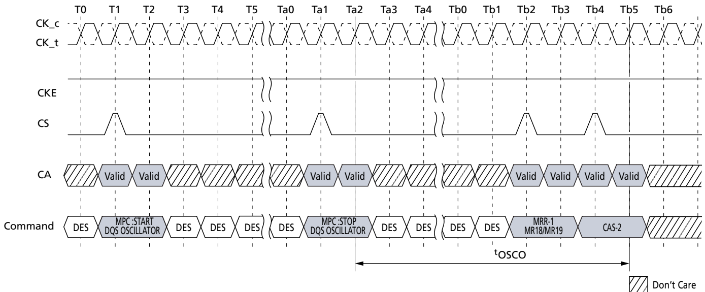
Figure 114: In Case of DQS Interval Oscillator is Stopped by MPC Command
