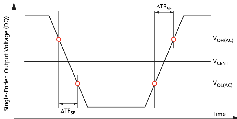
Figure 140: Single-Ended Output Slew Rate Definition
