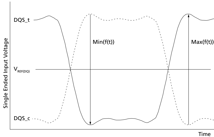
Figure 136: Definition of Differential DQS Peak Voltage
