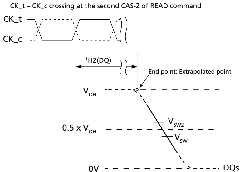
Figure 21: t_{HZ}(DQ) Method for Calculating Transitions and Endpoint
