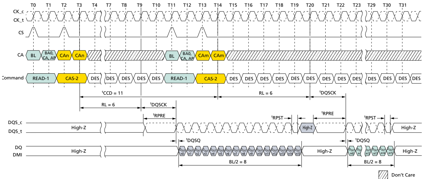
Figure 47: Consecutive READ: t_{CCD} = \text{MIN} + 3 , Preamble = Static, 0.5nCK Postamble
