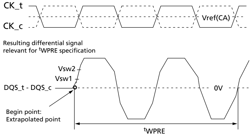
Figure 25: Method for Calculating t_{\text{WPRE}} Transitions and Endpoints
