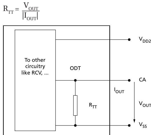
Figure 121: ODT for CA
