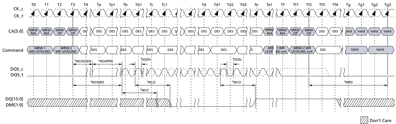
Figure 99: Write Leveling Timing – t_{DQSL}(\text{MIN})
