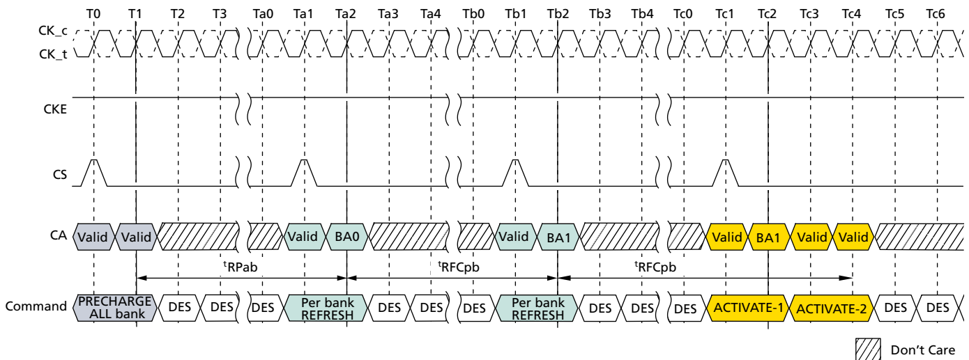
Figure 67: Per-Bank REFRESH Operation
