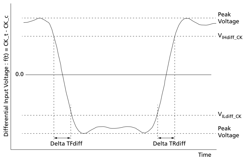
Figure 133: Differential Input Slew Rate Definition for CK t , CK c
