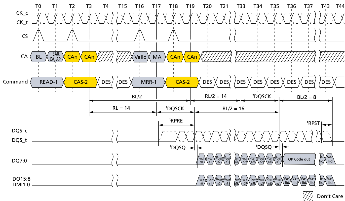
Figure 88: READ-to-MRR Timing
