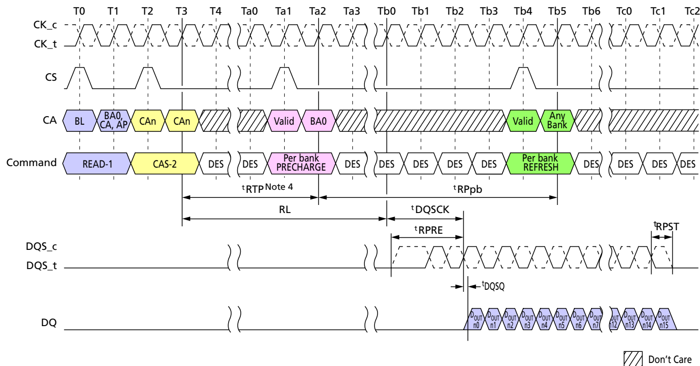
Figure 70: Burst READ Operation Followed by Per Bank Refresh
