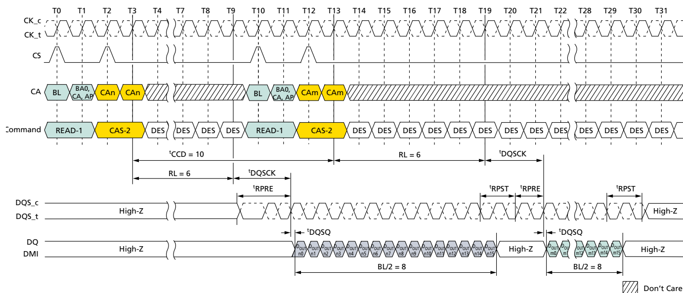
Figure 40: Consecutive READ: t_{CCD} = \text{MIN} + 2 , Preamble = Toggle, 1.5nCK Postamble
