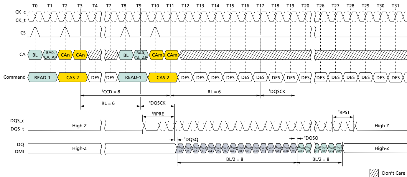
Figure 35: READ Operations: t_{CCD} = \text{MIN} , Preamble = Toggle, 1.5n\text{CK} Postamble
