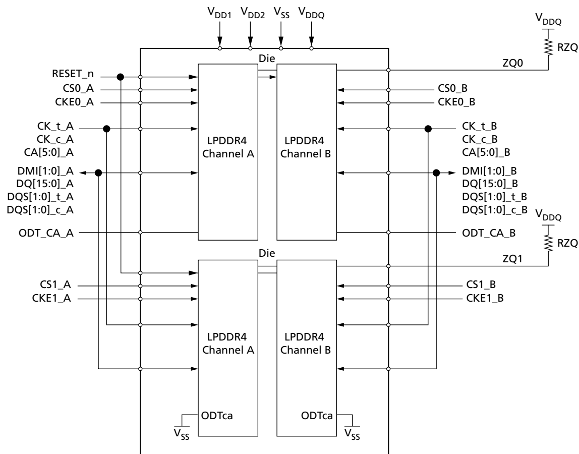
Figure 3: Dual-Die, Dual-Channel, Dual-Rank Package Block Diagram
