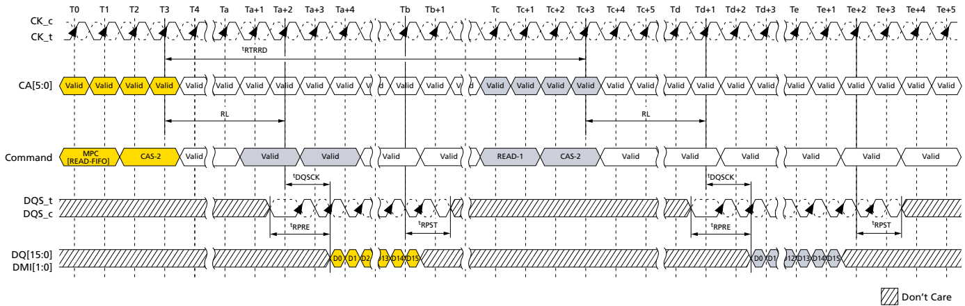
Figure 118: READ-FIFO – t_{\text{RPRE}} = Toggling, t_{\text{RPST}} = 1.5n\text{CK}
