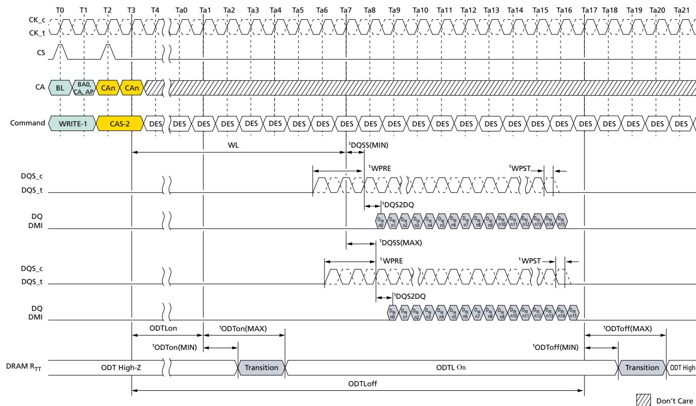
Figure 139: Asynchronous ODTon/ODToff Timing
