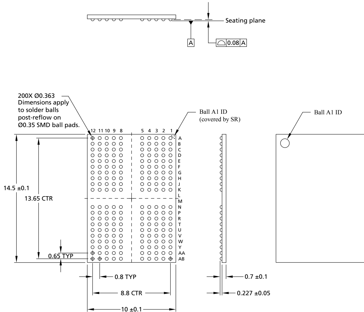
Figure 7: 200-Ball WFBGA – 10mm x 14.5mm (Package Code: DS)
