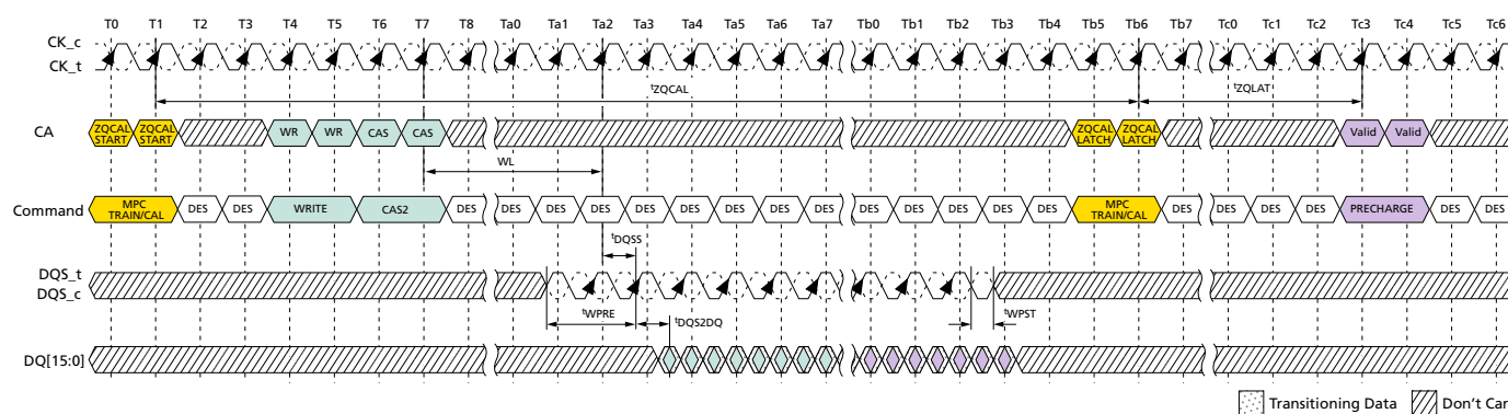
Figure 131: ZQCAL Timing
