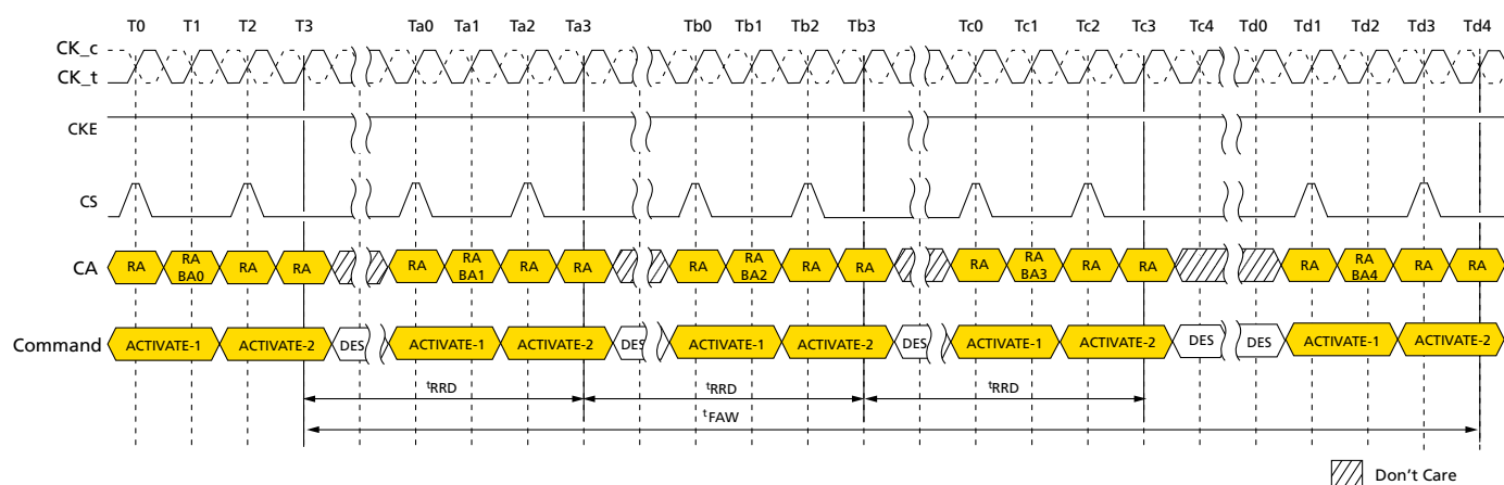
Figure 13: t_{FAW} Timing
