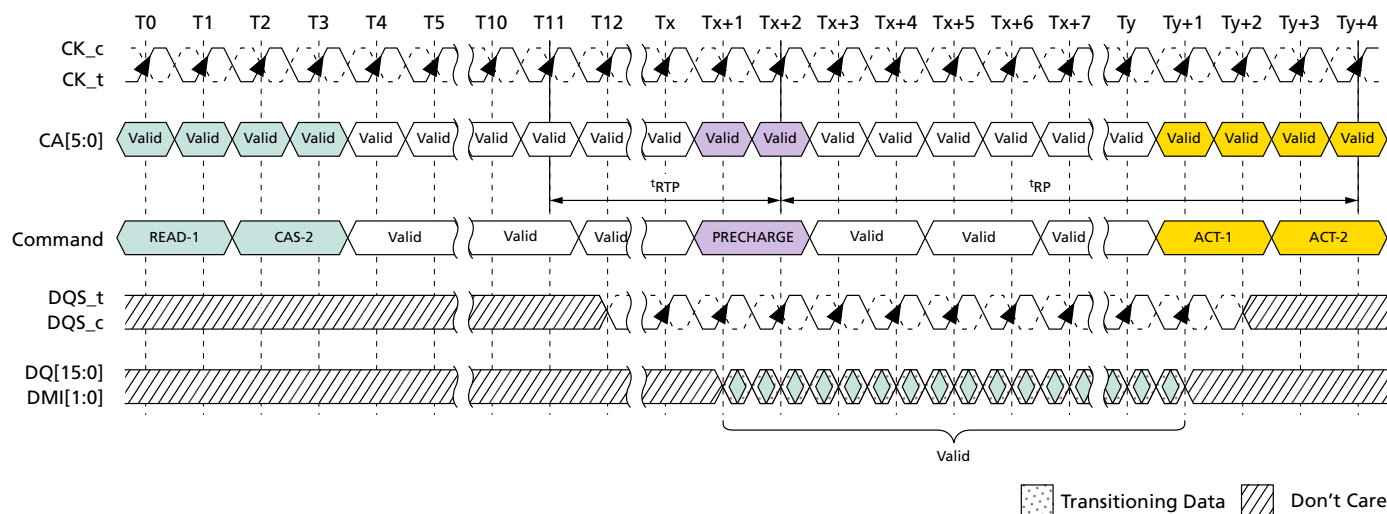
Figure 63: Burst READ Followed by Precharge – BL32, 2 n CK, 0.5nCK Postamble
