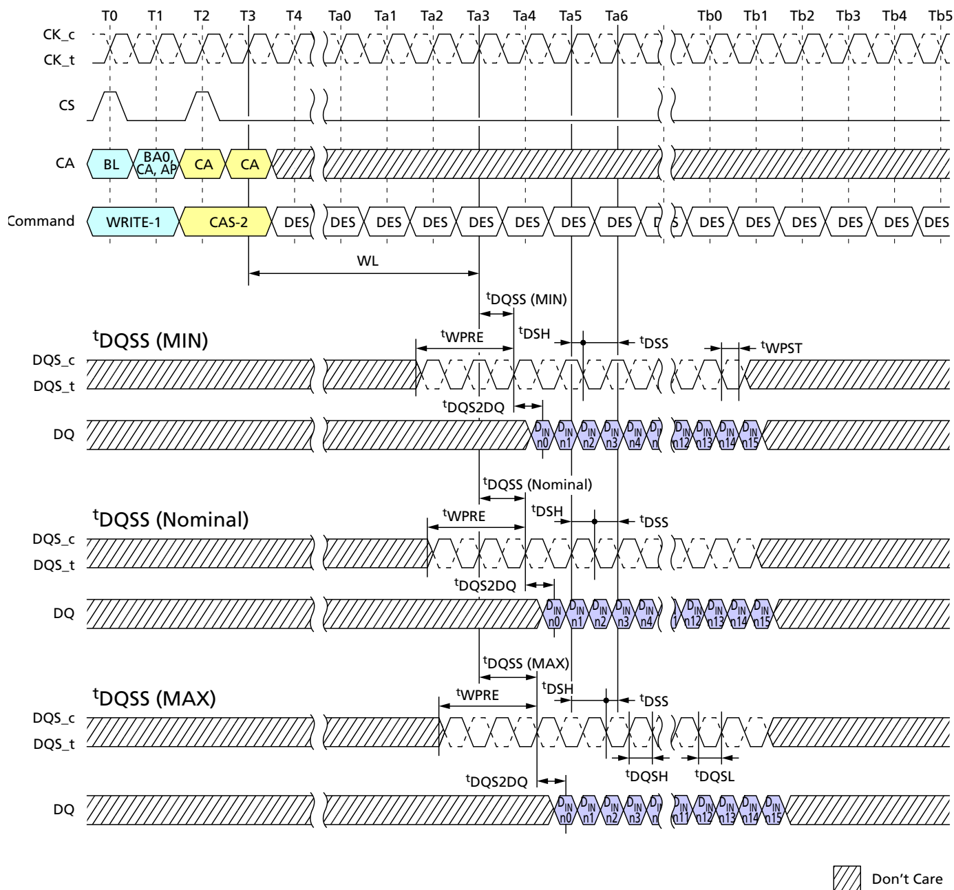
Figure 28: Write Timing
