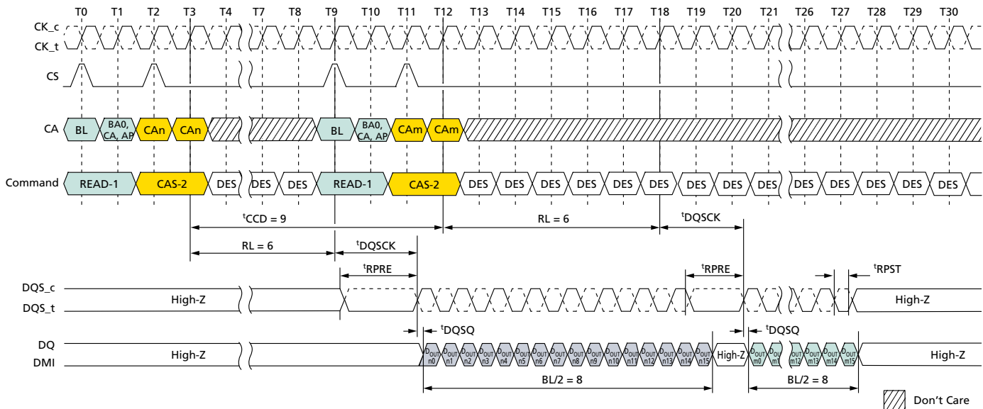
Figure 43: Consecutive READ: t_{CCD} = \text{MIN} + 1 , Preamble = Static, 0.5nCK Postamble
