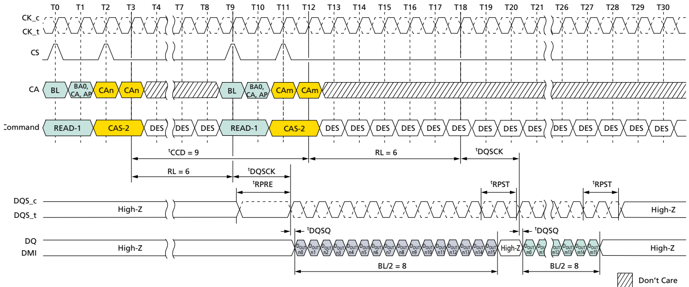
Figure 42: Consecutive READ: t_{CCD} = \text{MIN} + 1 , Preamble = Static, 1.5nCK Postamble
