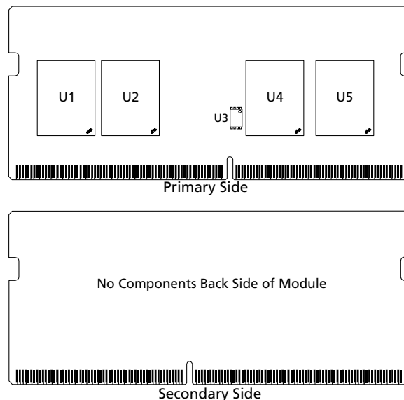
Figure 1: 260-Pin SODIMM
