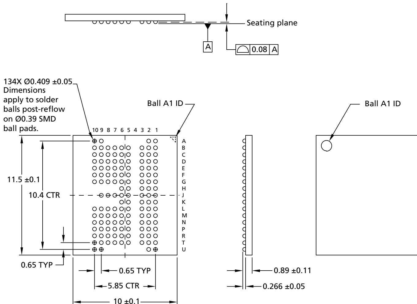
Figure 6: 134-Ball VFBGA – 10mm x 11.5mm (Package Code: HE)
