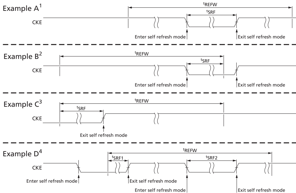
Figure 40: t_{SRF} Definition
