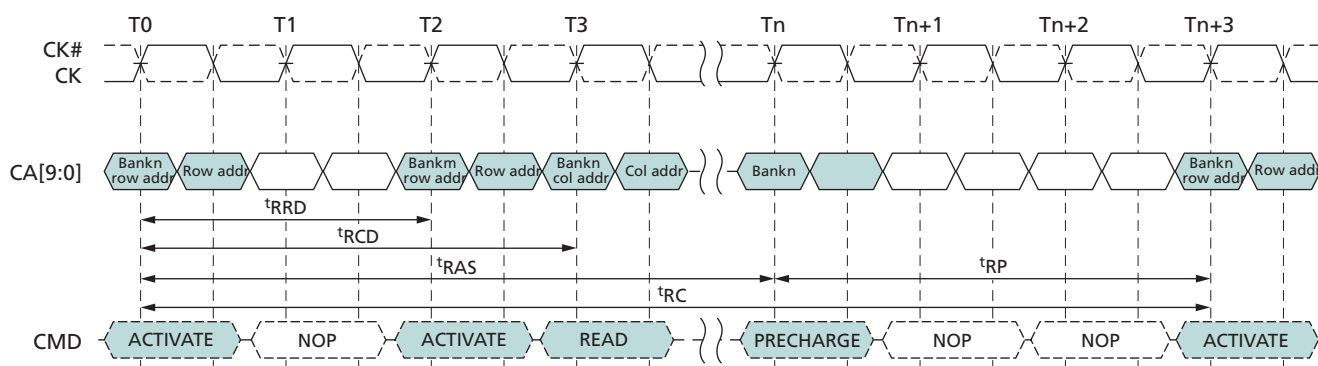
Figure 10: ACTIVATE Command
