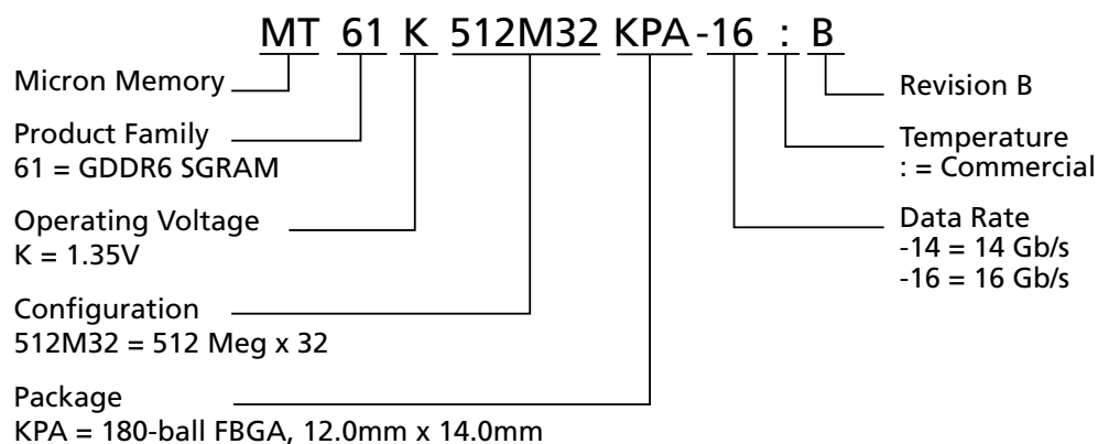
Figure 1: Part Numbering
