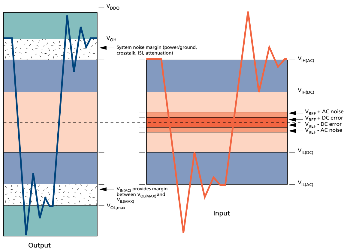
Figure 12: Voltage Waveform
