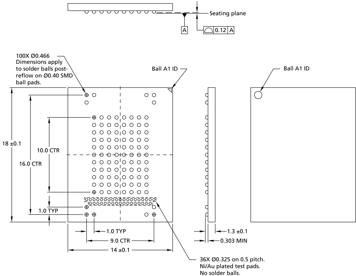
Figure 4: 100-Ball LBGGA – 14mm x 18.00mm x 1.4mm (Package Code: DQ)
