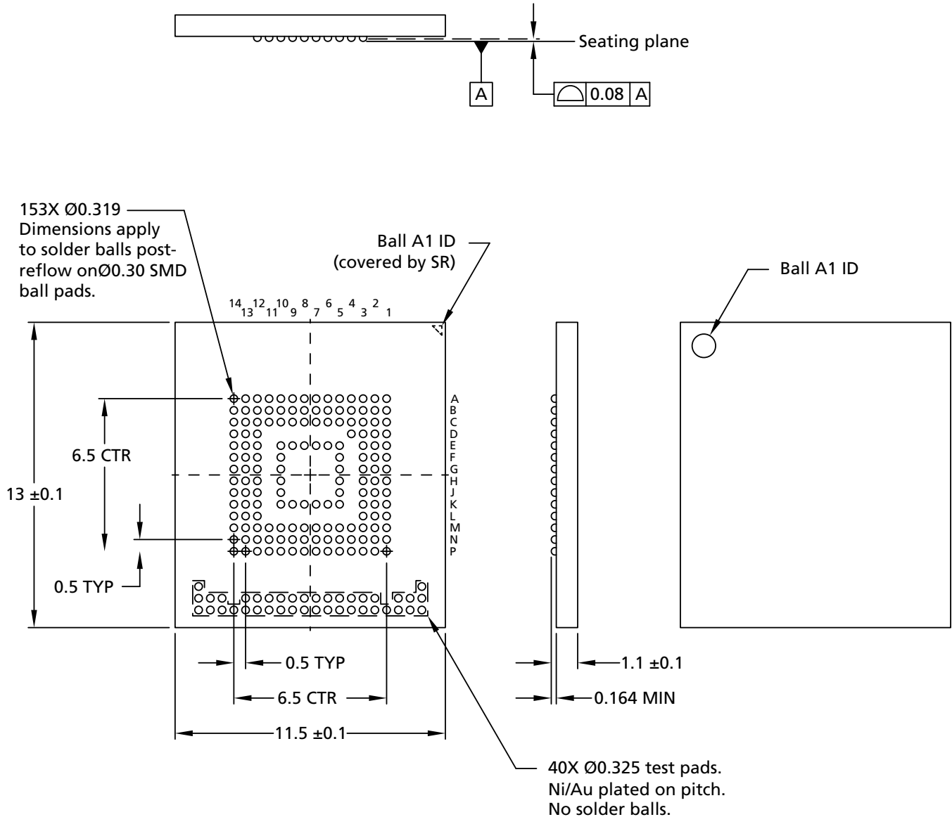
Figure 5: 153-Ball TFBGA – 11.50mm x 13.00mm x 1.2mm (Package Code: DM)
